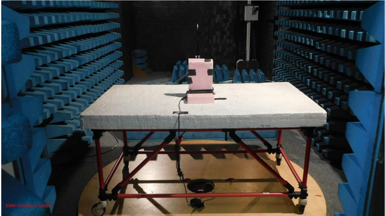
Picture 5: CDC, test setup radiated emission test 9 kHz -30 MHz - PCB antenna set 2063503:4477 (front view)
