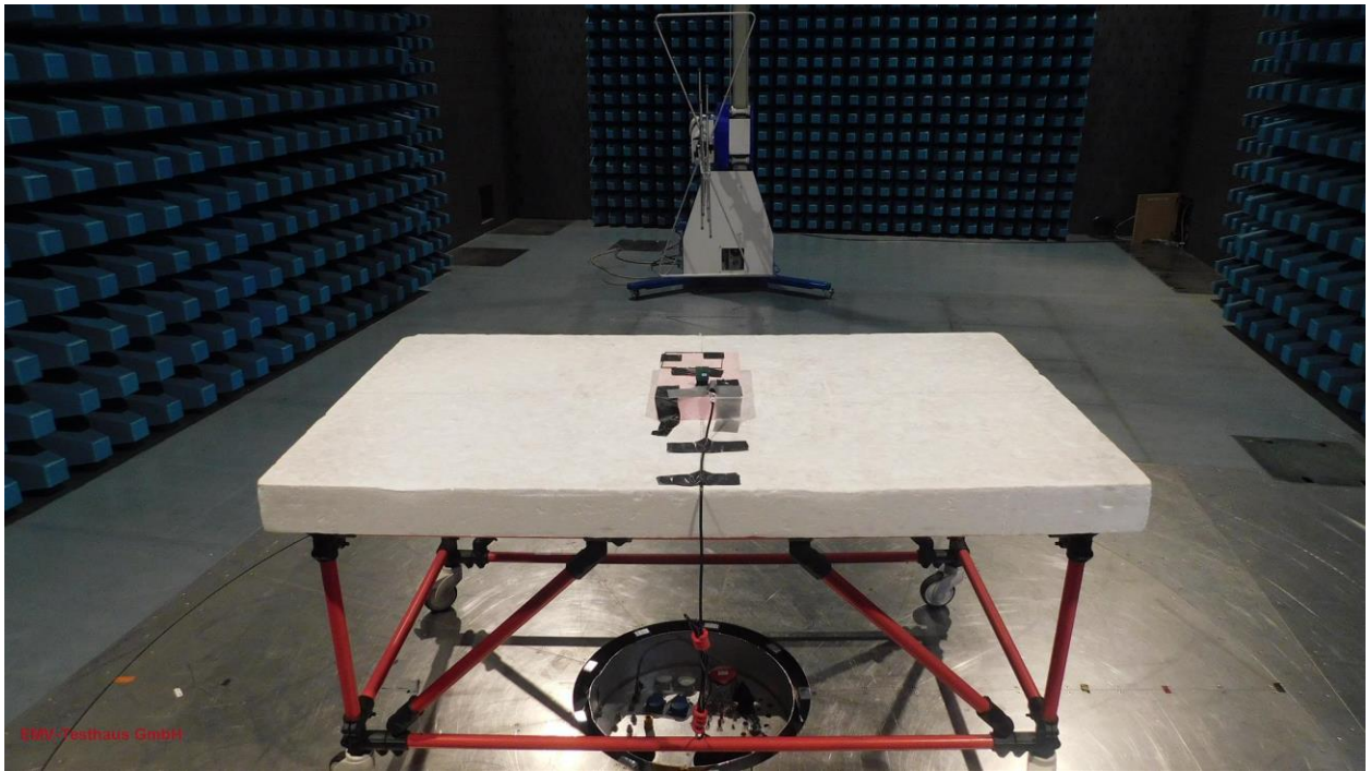
Picture 11: SAC, radiated emission test 30 MHz -1 GHz - PCB antenna 2063512:4612 (front view)
