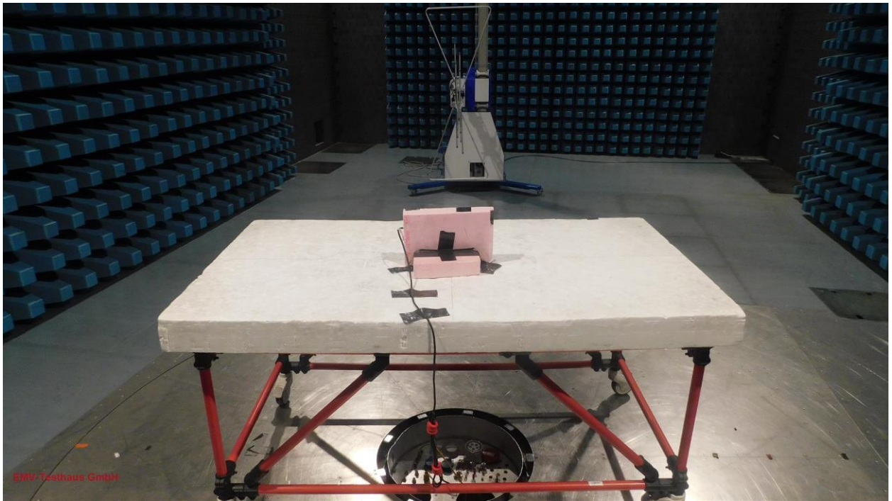
Picture 17: SAC, radiated emission test 30 MHz -1 GHz - PCB antenna 2063513:5170 (front view)
