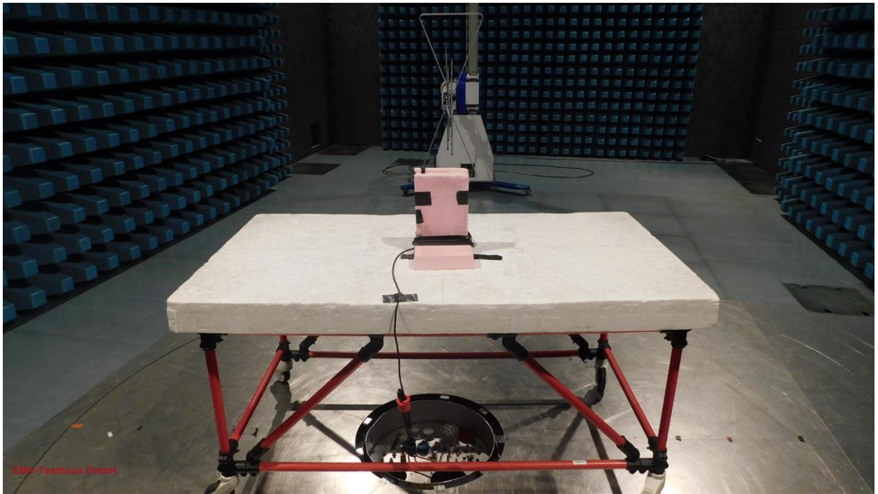
Picture 15: SAC, radiated emission test 30 MHz -1 GHz - PCB antenna set 2063503:4477 (front view)
