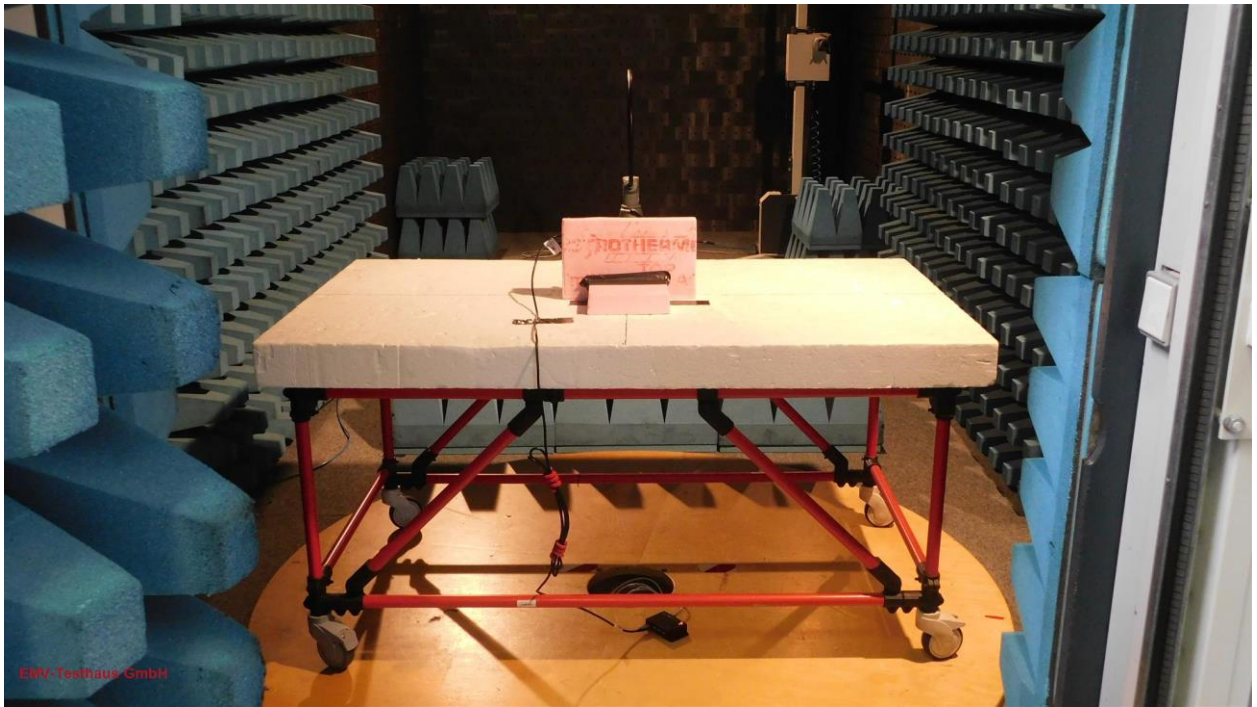
Picture 1: CDC, test setup radiated emission test 9 kHz -30 MHz - PCB antenna 2063512:4612 (front view)
