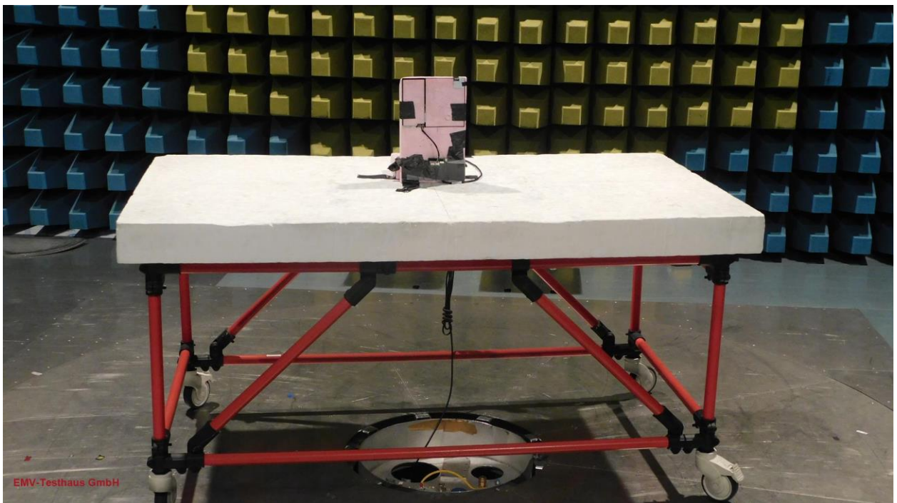
Picture 16: SAC, radiated emission test 30 MHz -1 GHz - PCB antenna set 2063503:4477 (rear view)
