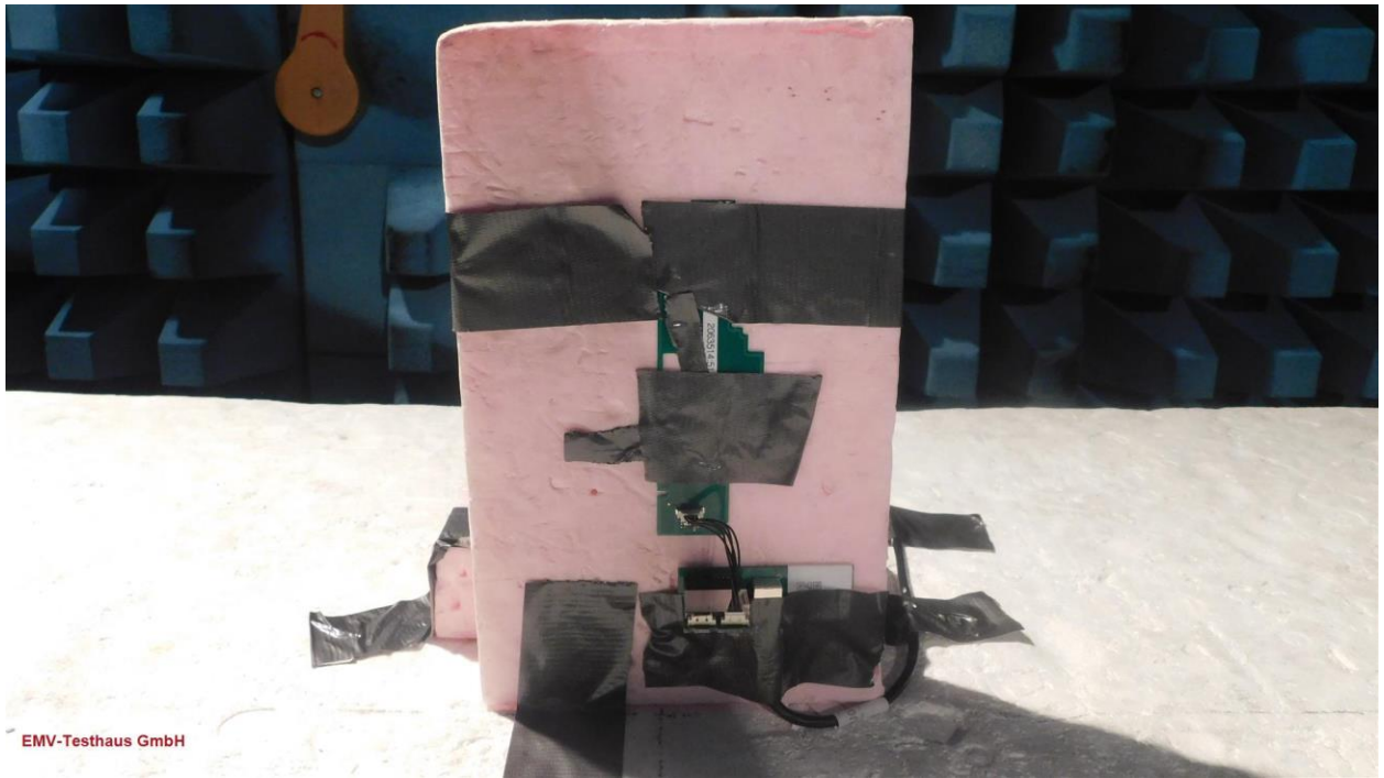
Picture 33: EUT-position 1 - PCB antenna set 2063514:5171
