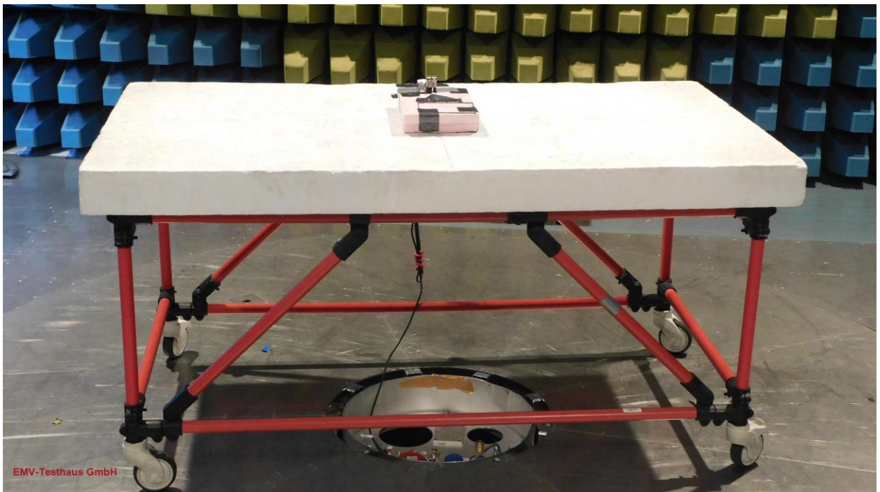
Picture 12: SAC, radiated emission test 30 MHz -1 GHz - PCB antenna 2063512:4612 (rear view)
