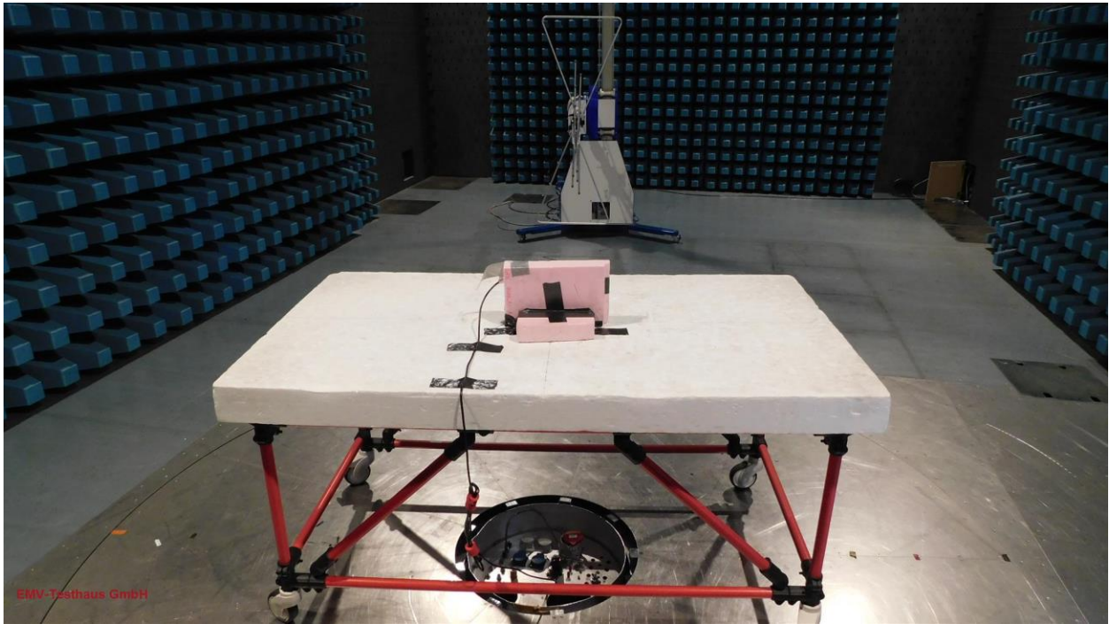
Picture 13: SAC, radiated emission test 30 MHz -1 GHz - PCB antenna 2009168:4834 (front view)
