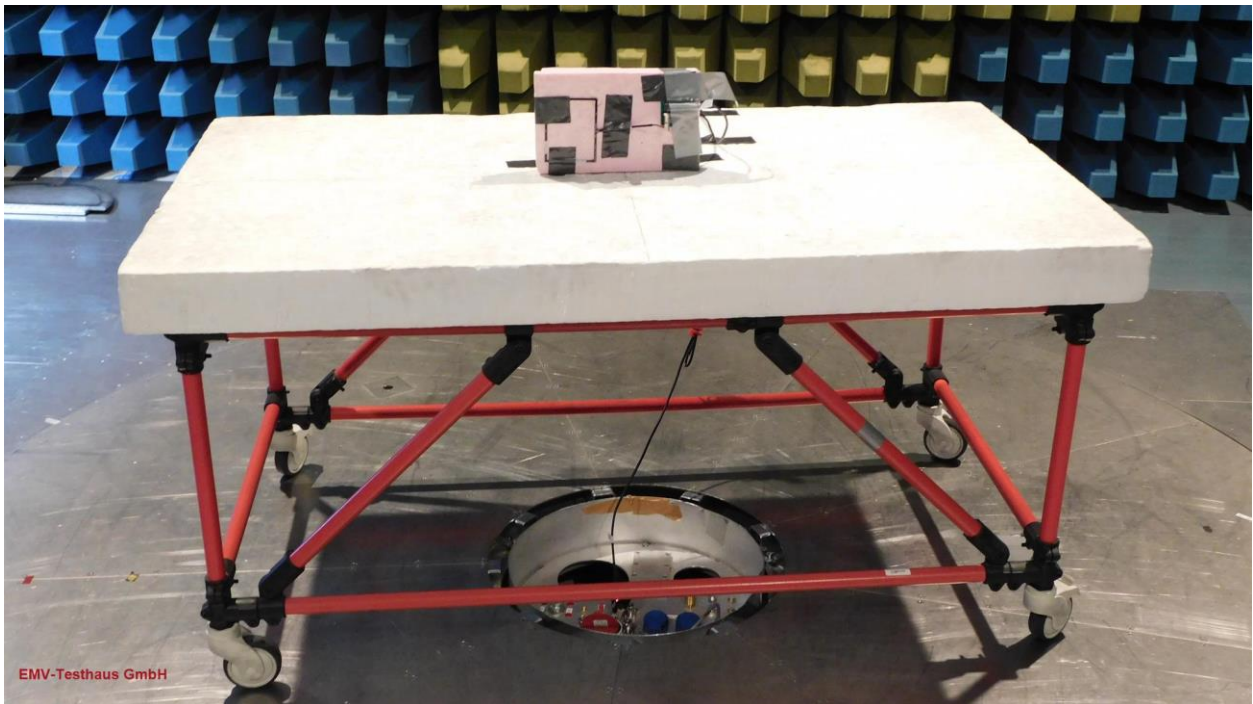
Picture 14: SAC, radiated emission test 30 MHz -1 GHz - PCB antenna 2009168:4834 (rear view)
