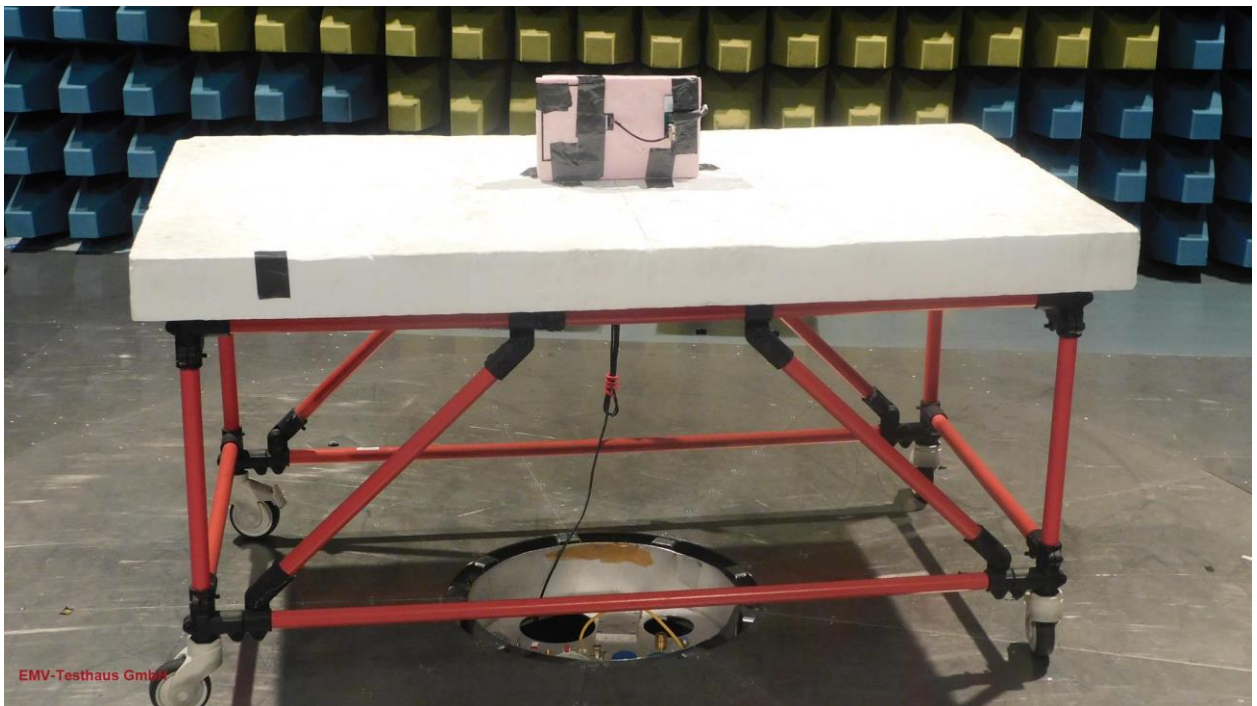
Picture 18: SAC, radiated emission test 30 MHz -1 GHz - PCB antenna 2063513:5170 (rear view)
