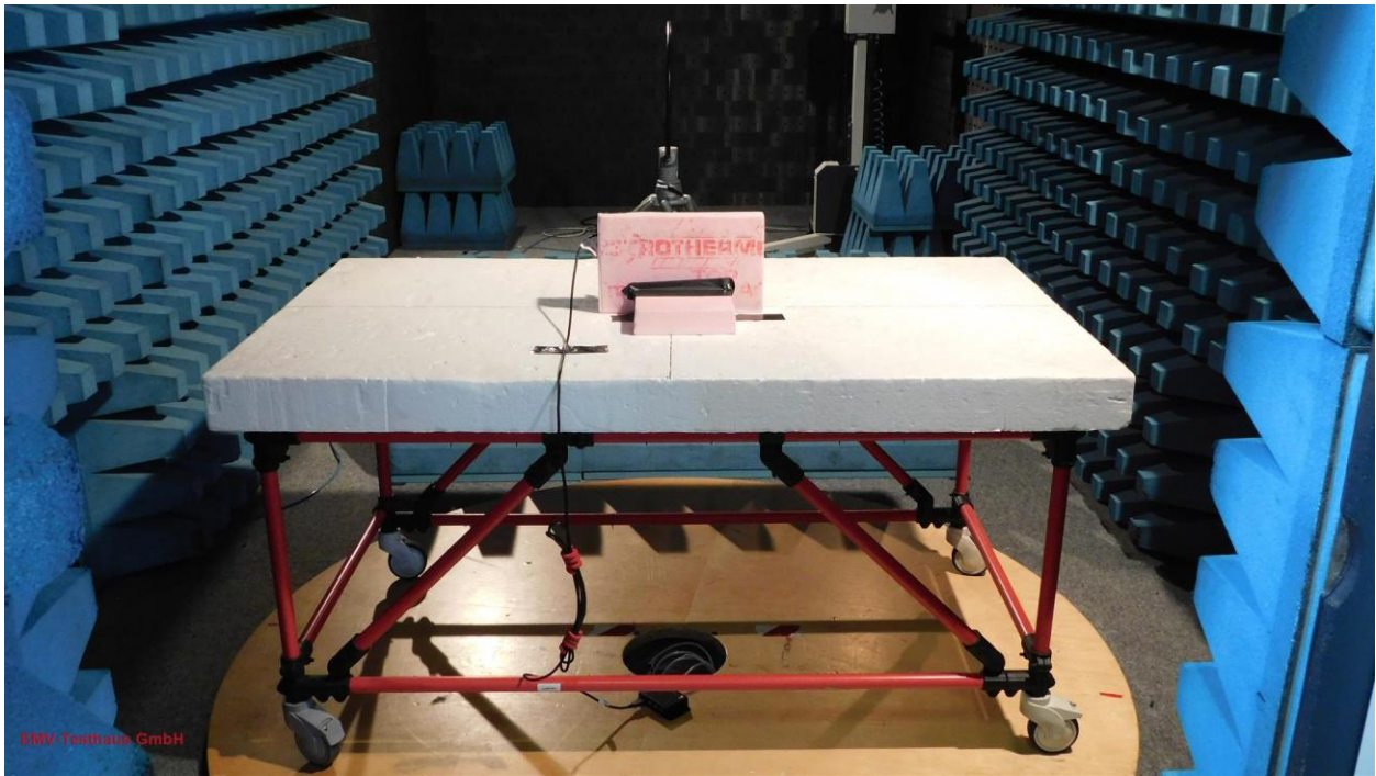
Picture 3: CDC, test setup radiated emission test 9 kHz -30 MHz - PCB antenna 2009168:4834 (front view)
