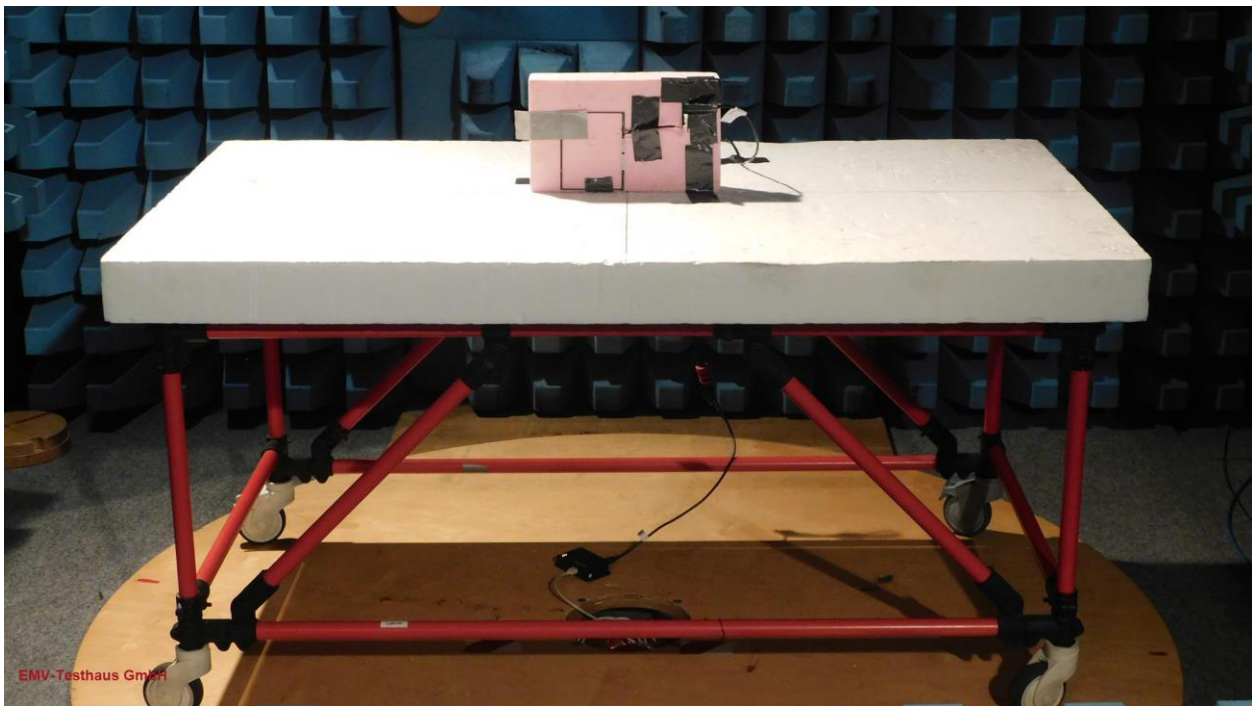
Picture 2: CDC, test setup radiated emission test 9 kHz -30 MHz - PCB antenna 2063512:4612 (rear view)
