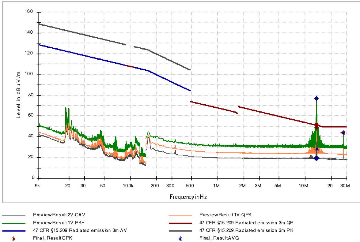
Figure 15: Chart of emissions test below 30 MHz with tag in position 2, antenna in line at 3 m
