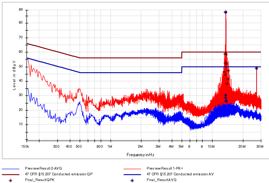
Figure 8: Chart of AC power-line conducted emissions test – phase N – without termination
