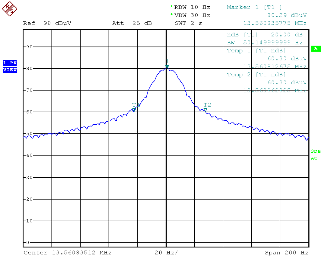
Figure 12: Chart of 20 dB bandwidth tests
