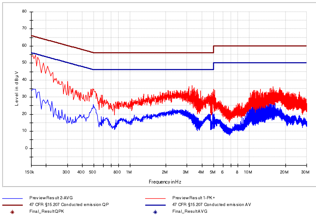
Figure 10: Chart of AC power-line conducted emissions test – phase L1 – with termination
