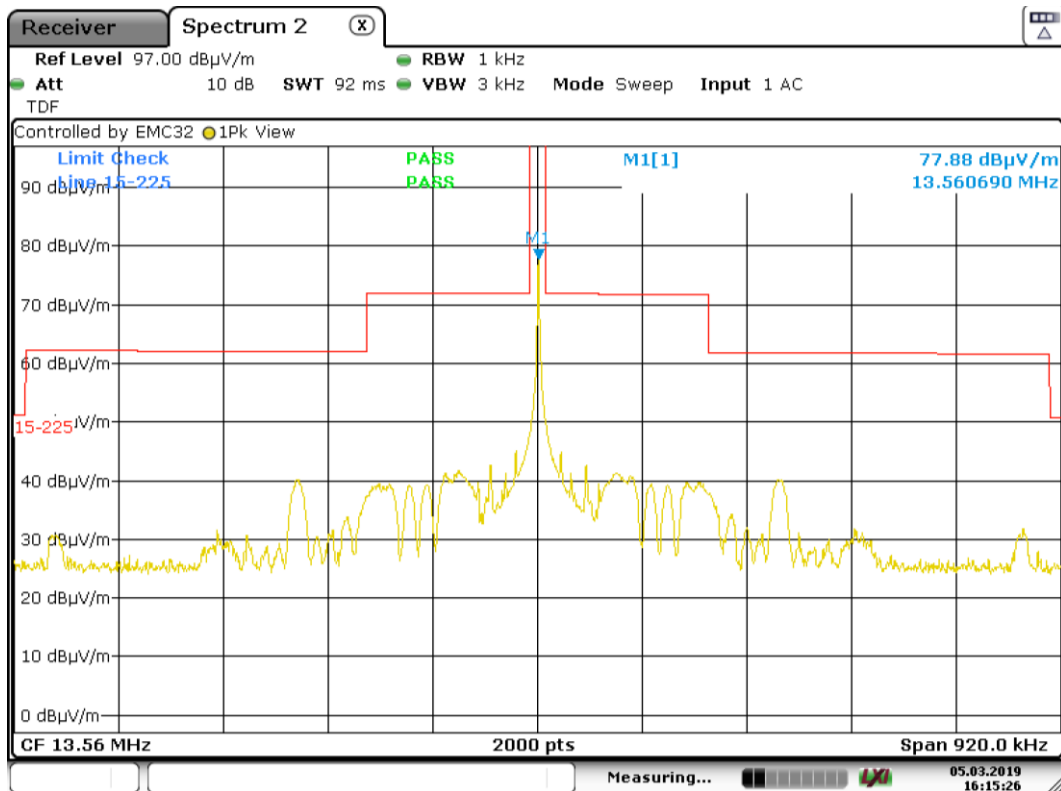
Figure 14: Chart of emission within the band 13.110 MHz to 14.010 MHz, without tag, position 3, antenna in line @ 3m distance
