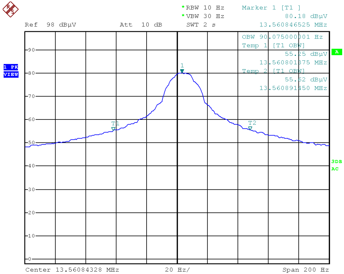
Figure 13: Chart of occupied bandwidth test
