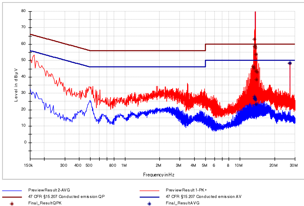
Figure 6: Chart of AC power-line conducted emissions test – phase L1 – without termination
