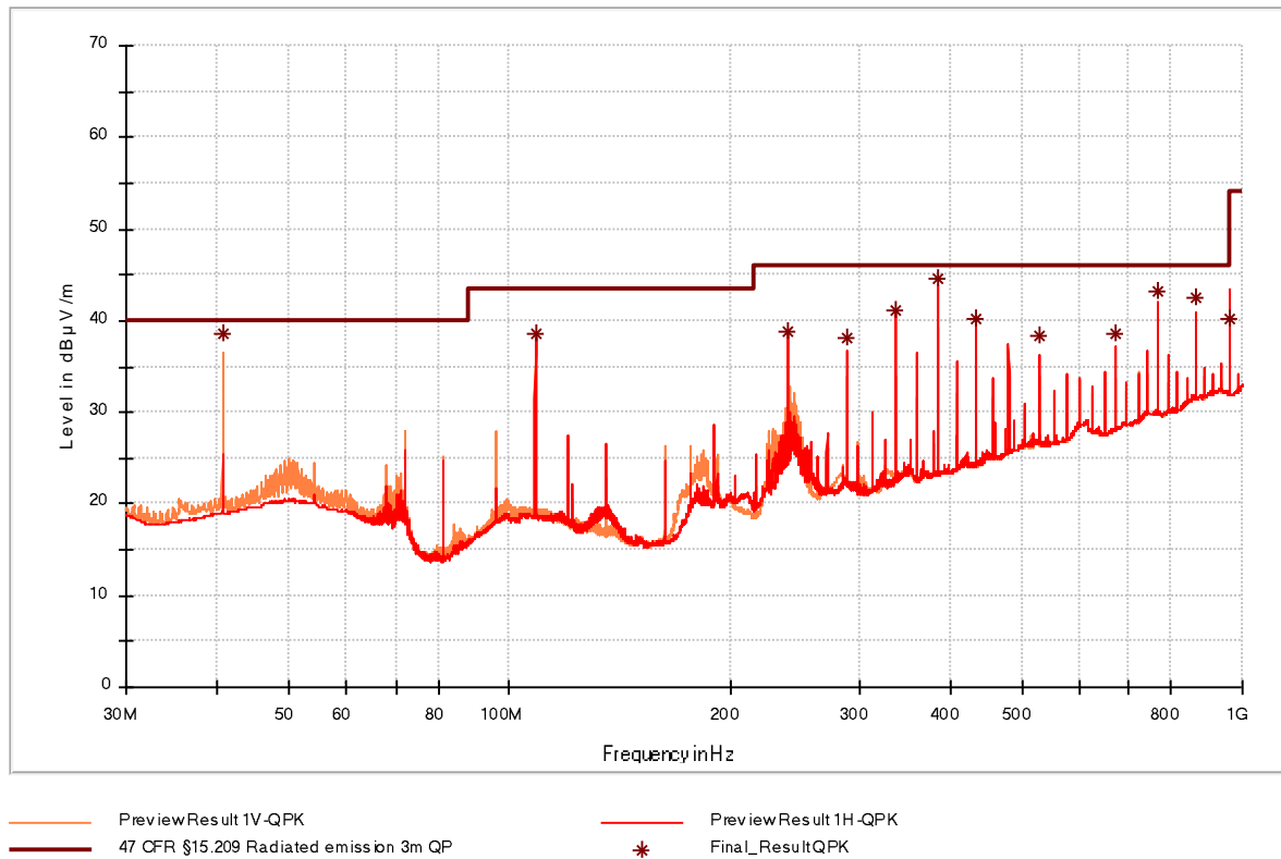
Figure 16: Chart of emissions test from 30 MHz to 1 GHz with tag in position 1 at 3 m
