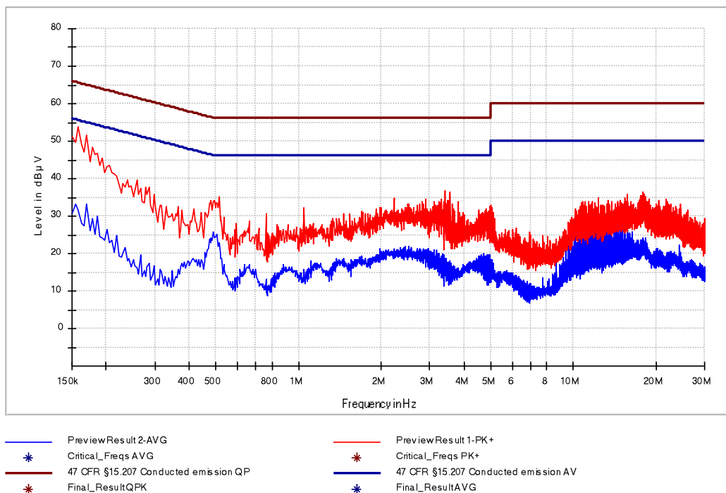
Figure 11: Chart of AC power-line conducted emissions test – phase N – with termination
