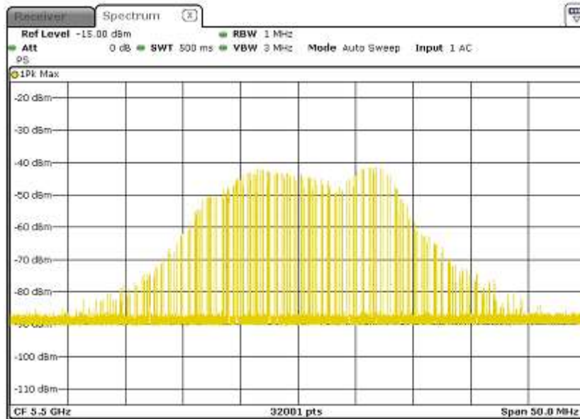
EUT (master) links with Client on 5500MHz
