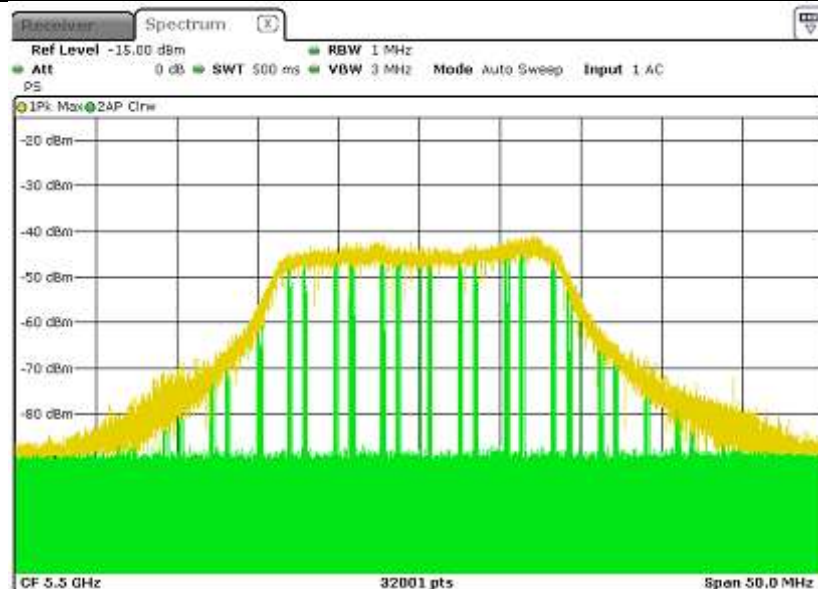
Client performed with channel-loading via master.
