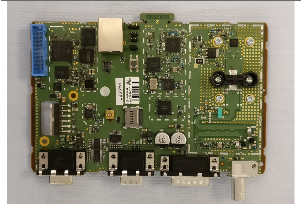
MDT-500-2 PCB Top face with screening cans removed
