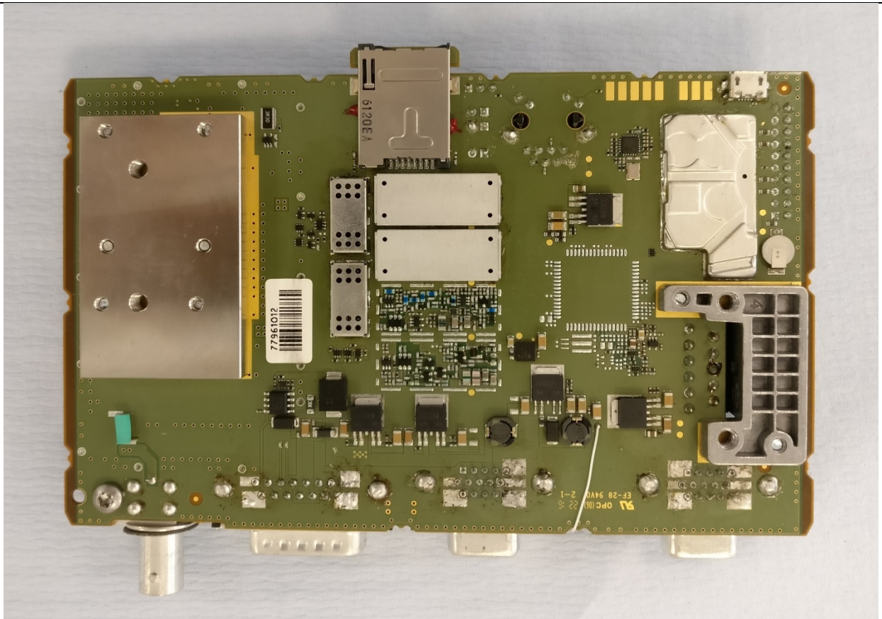
MDT-500-2 PCB Bottom face with screening cans fitted
