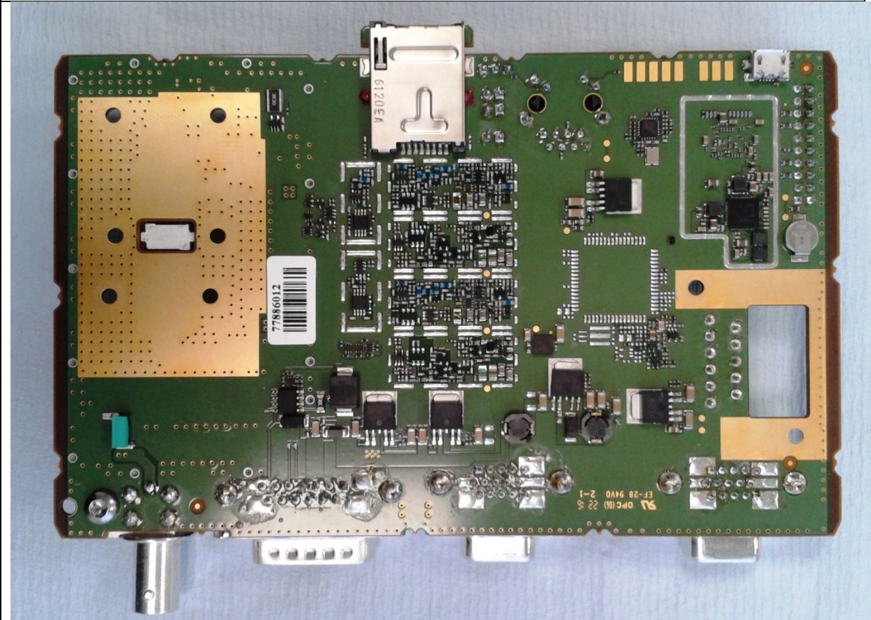
MDT-500-2 PCB Bottom face with screening cans removed
