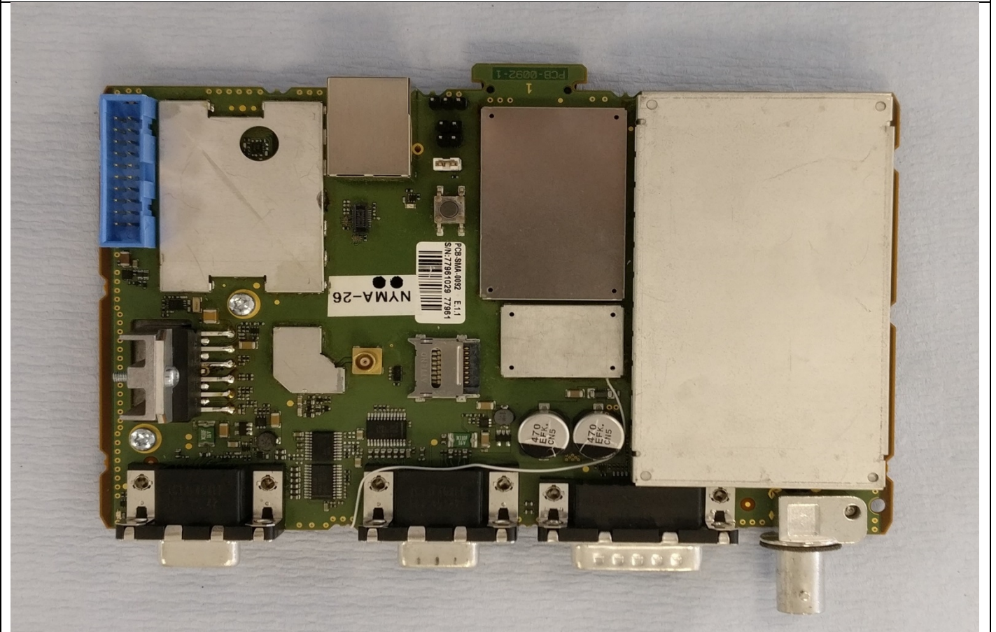
MDT-500-2 PCB Top face with screening cans fitted
