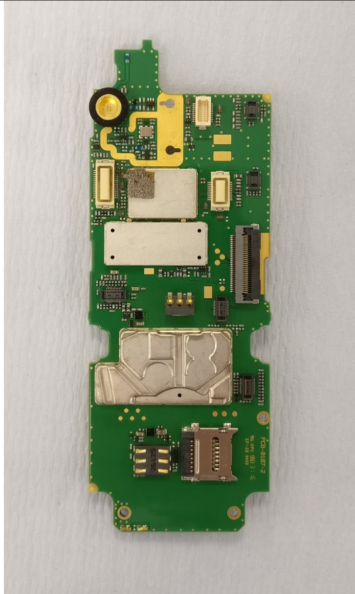
HTT-500-2 PCB rear with screening cans
