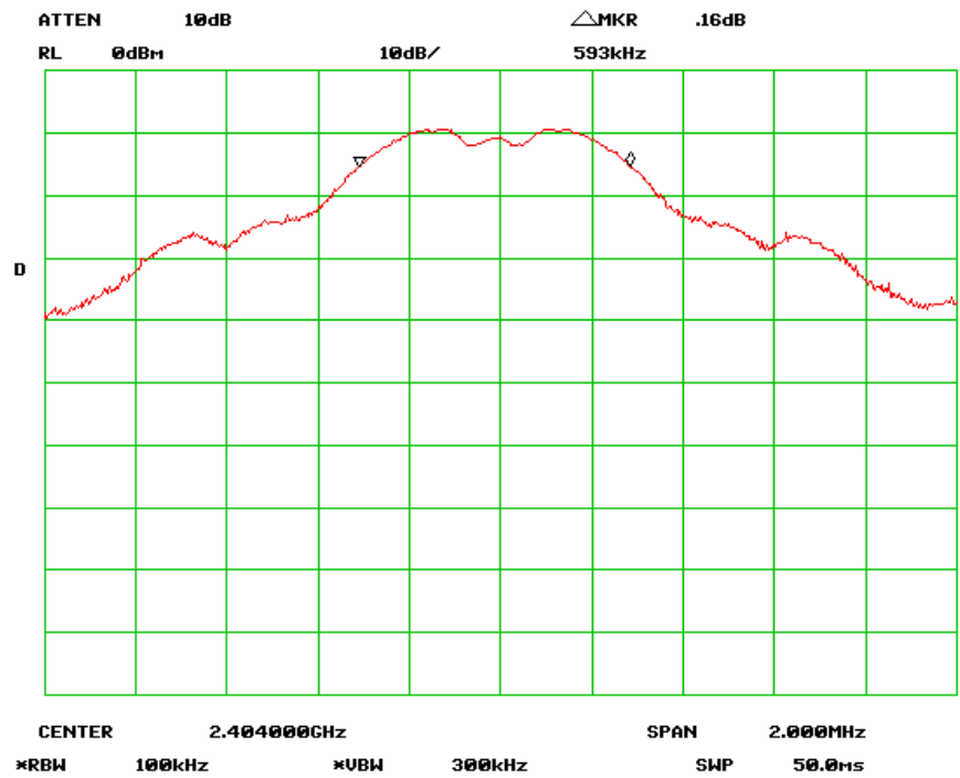
6dB Bandwidth – Low Channel
