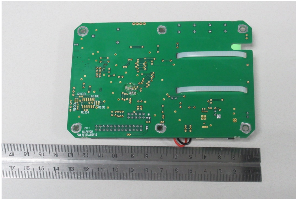
PCB 2 Bottom:
