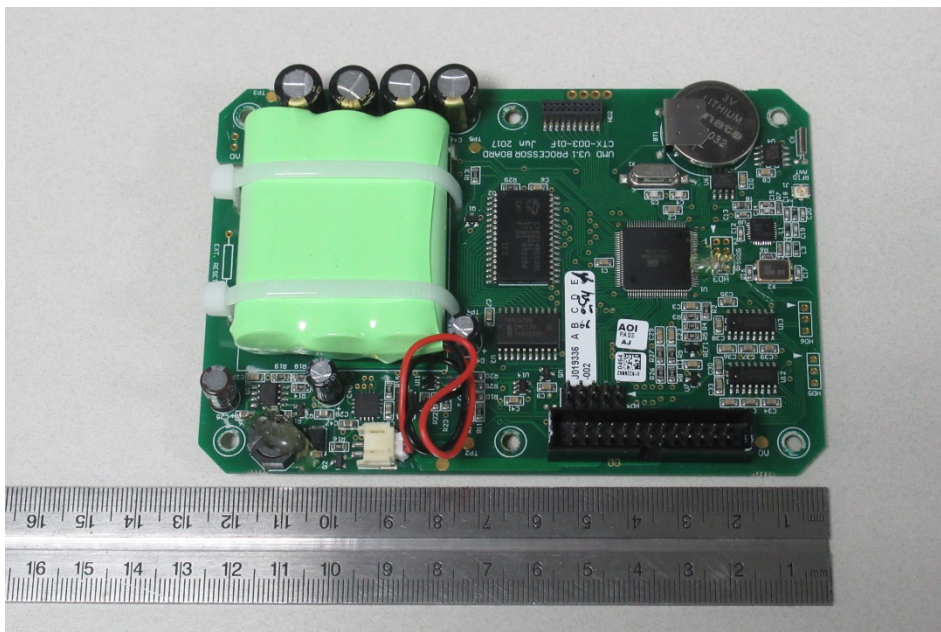
PCB 2 Top:
