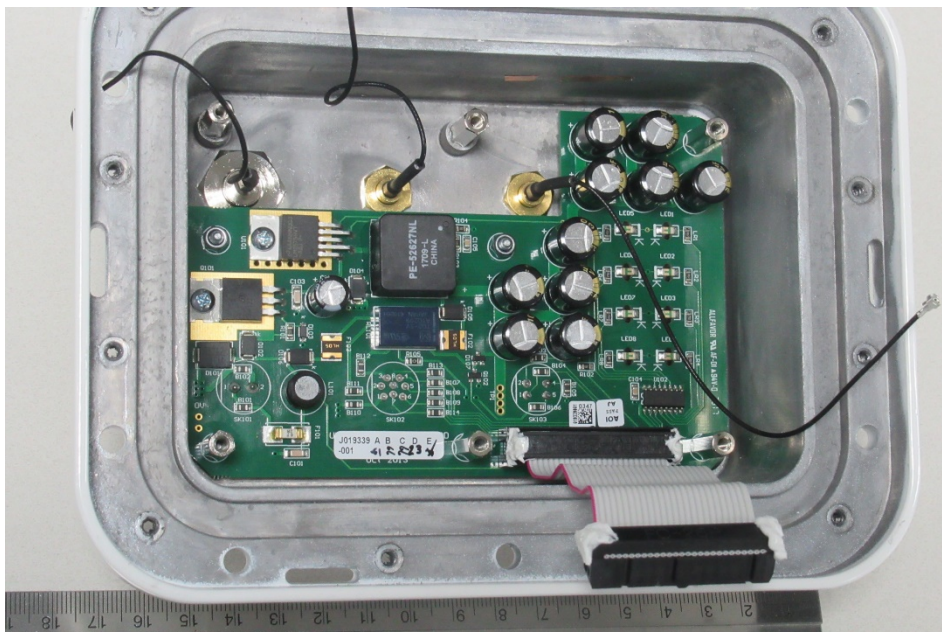
PCB 3 Top:
