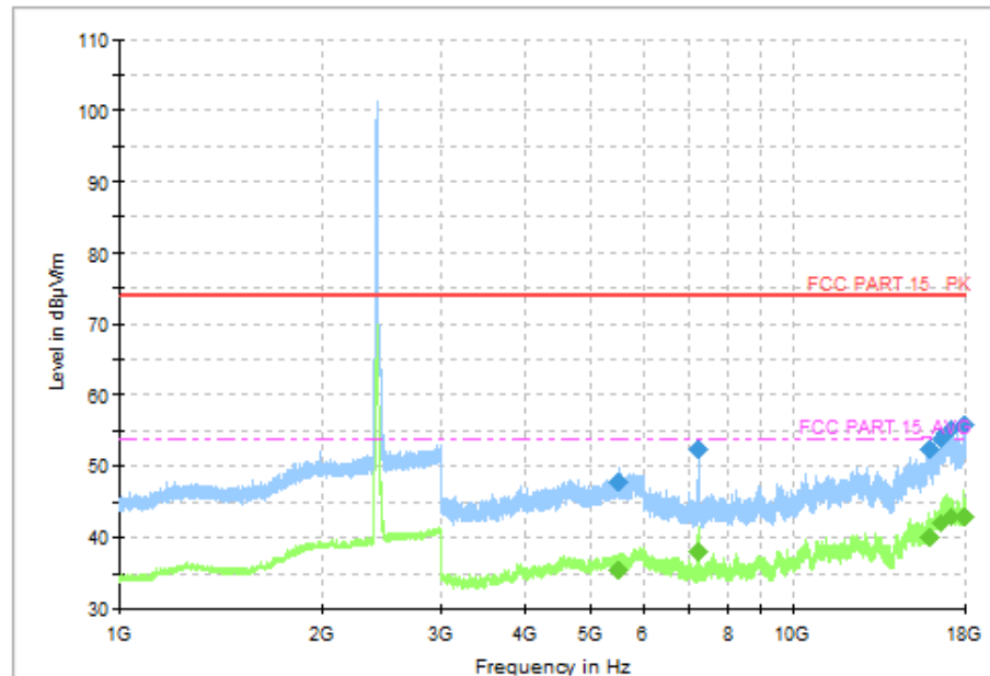
Fig.62 Radiated Spurious Emission (802.11n-HT20, CH1, 1 GHz-18 GHz)
