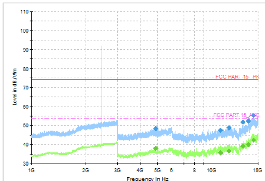
Fig.19 Radiated Spurious Emission (CH19, 1 GHz ~18 GHz), LE 1M
