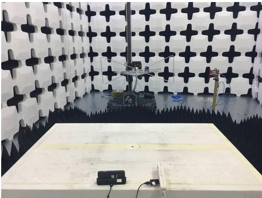
6. Radiated Emissions (Part 15B Charging mode) (Above 1GHz)
