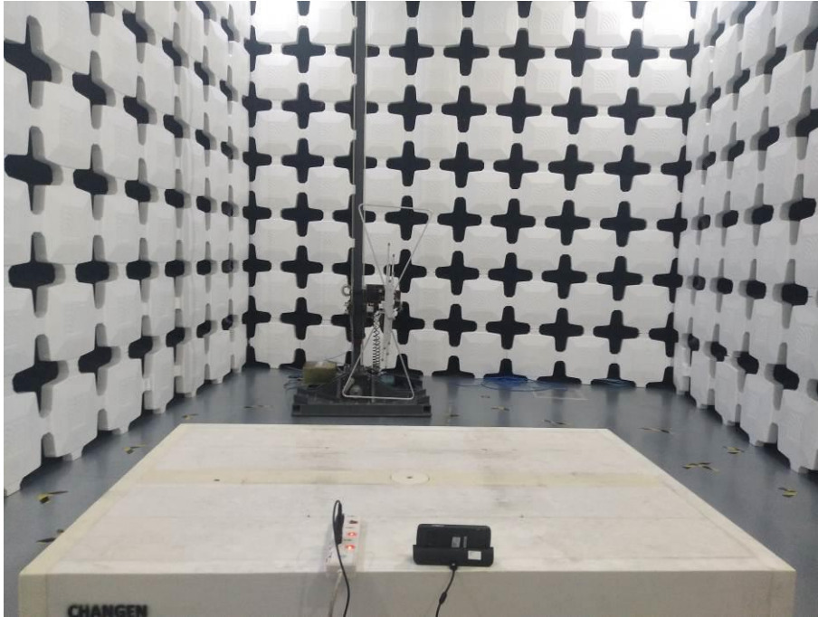
5. Radiated Emissions (Part 15B Charging mode) (below 1GHz)
