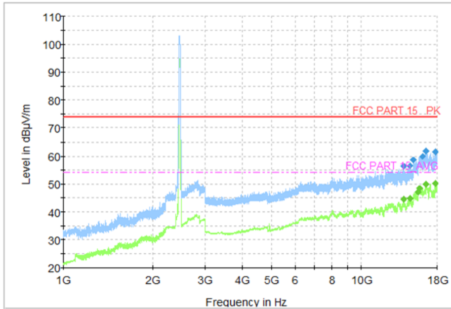
Fig.95 Radiated Spurious Emission (802.11g, Ch11, 1 GHz-18 GHz)
