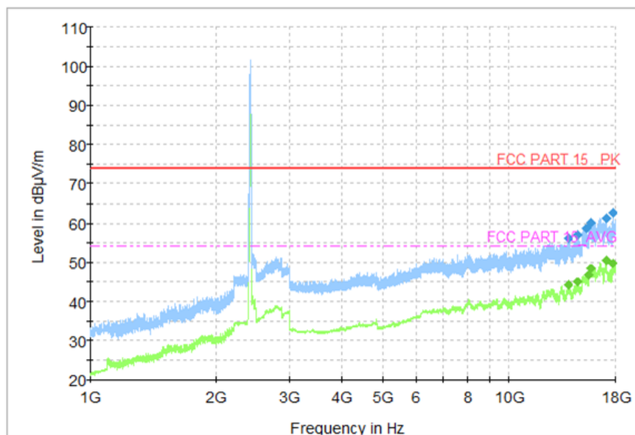
Fig.90 Radiated Spurious Emission (802.11g, Ch1, 1 GHz-18 GHz)
