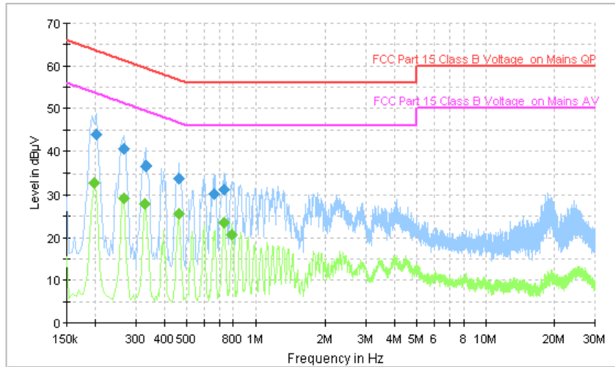
Fig.117 AC Powerline Conducted Emission (Idle, AE2, 120V)
