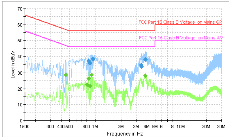
Fig.114 AC Powerline Conducted Emission (Traffic, AE1, 120V)
