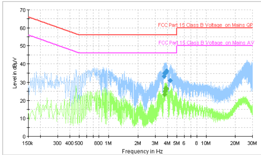
Fig.115 AC Powerline Conducted Emission (Idle, AE1, 120V)
