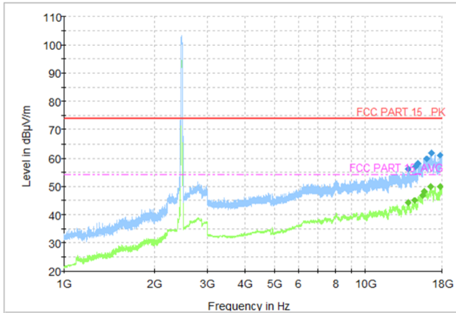
Fig.103 Radiated Spurious Emission (802.11n-20MHz, Ch11, 1 GHz-18 GHz)
