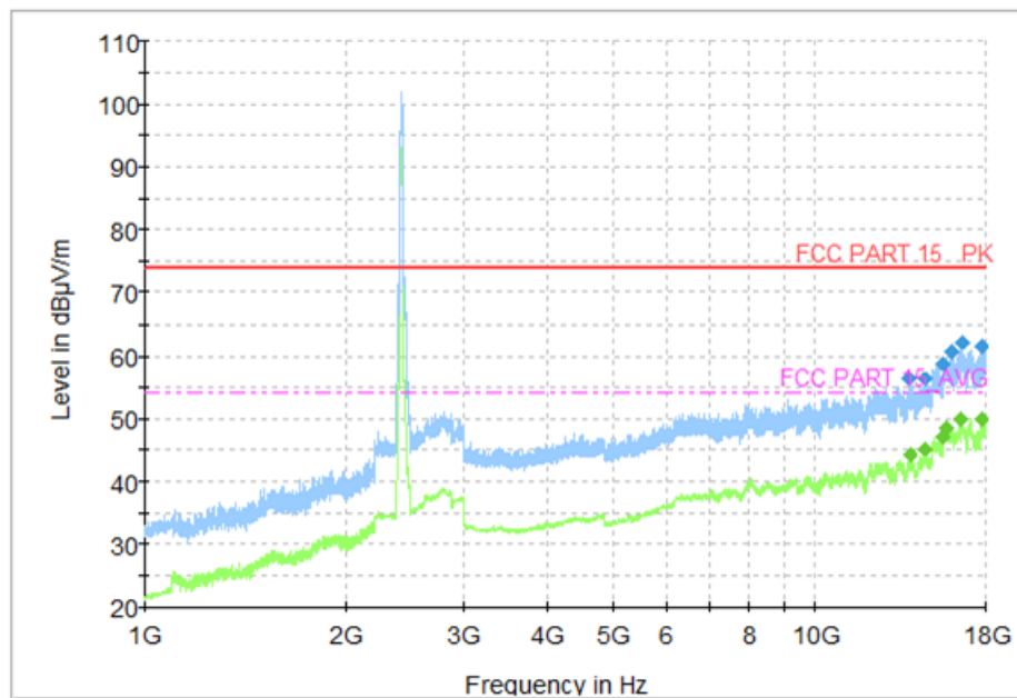
Fig.106 Radiated Spurious Emission (802.11n-40MHz, Ch3, 1 GHz-18 GHz)
