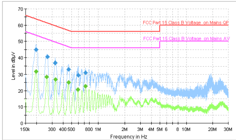
Fig.116 AC Powerline Conducted Emission (Traffic, AE2, 120V)
