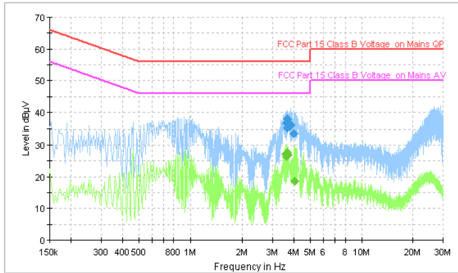
Fig.119 AC Powerline Conducted Emission (Idle, AE1, 240V)
