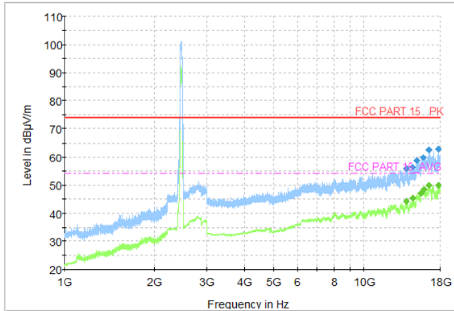
Fig.111 Radiated Spurious Emission (802.11n-40MHz, Ch9, 1 GHz-18 GHz)
