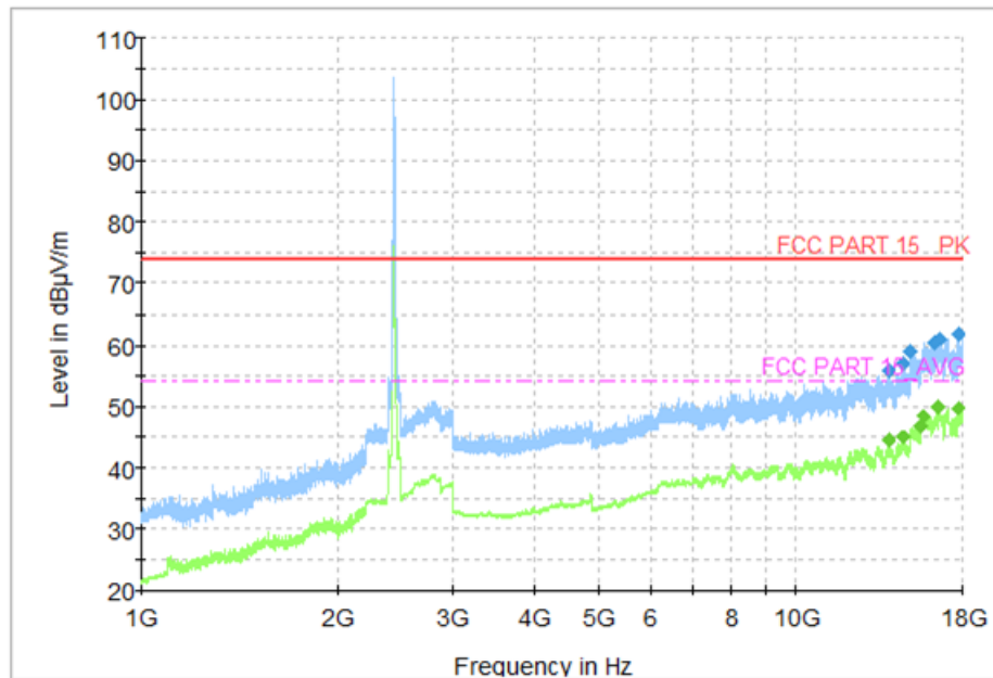
Fig.93 Radiated Spurious Emission (802.11g, Ch6, 1 GHz-18 GHz)
