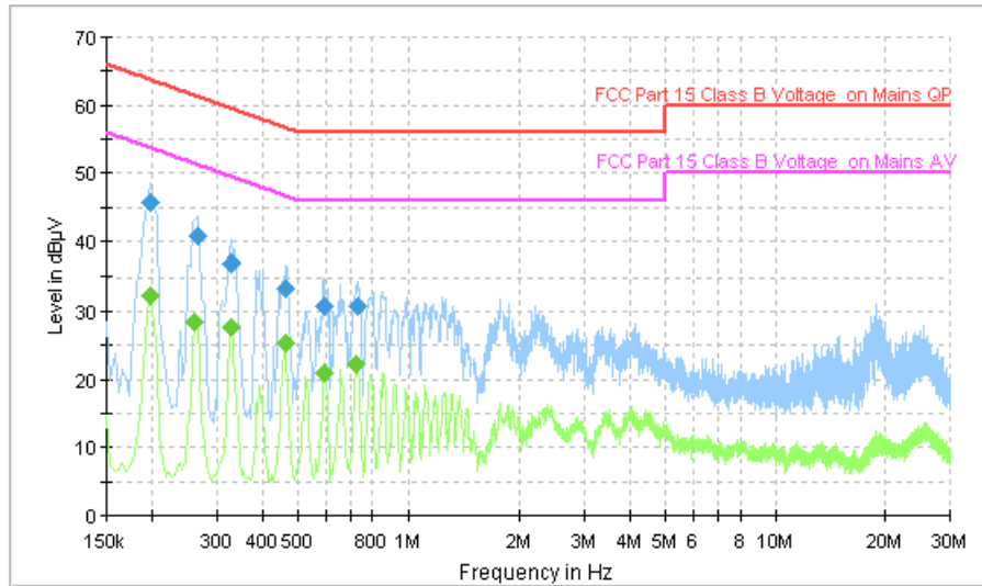
Fig.120 AC Powerline Conducted Emission (Traffic, AE2, 240V)
