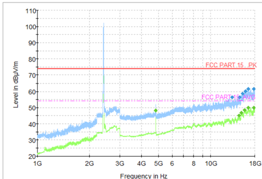
Fig.82 Radiated Spurious Emission (802.11b, Ch1, 1 GHz-18GHz)
