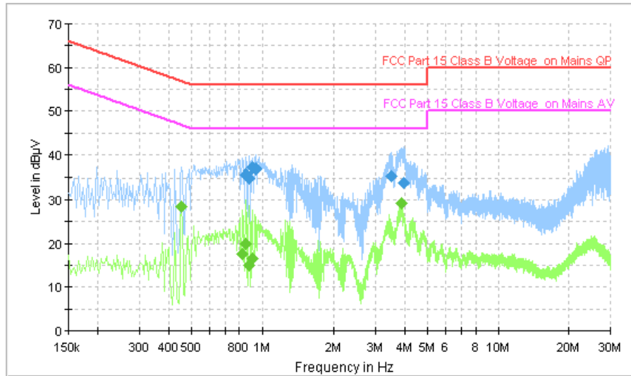
Fig.118 AC Powerline Conducted Emission (Traffic, AE1, 240V)
