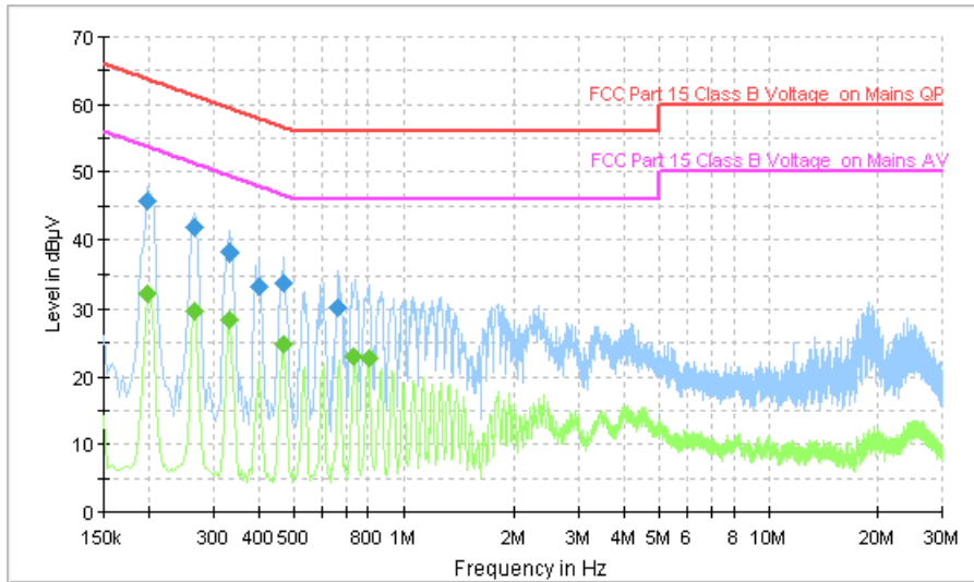
Fig.121 AC Powerline Conducted Emission (Idle, AE2, 240V)
