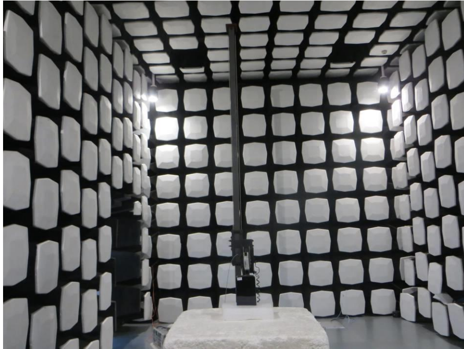
13. Radiated Emissions (Part 22/24) (Above 18GHz)
