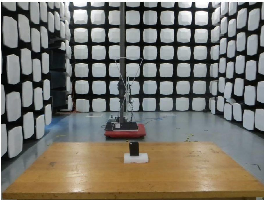
8. Radiated Emissions (Part 15C) 30M-1GHz)
