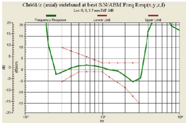
Fig 7.4 GSM1900 Ch661
