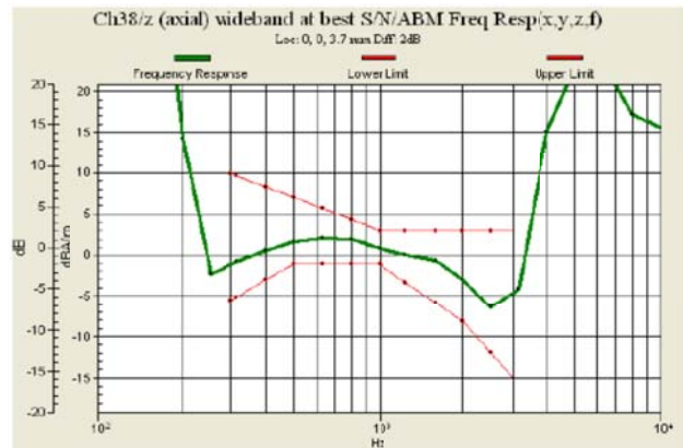
Fig 7.2 GSM900 Ch38
