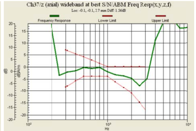
Fig 7.2 GSM900 Ch37
