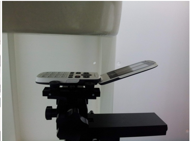
Left Tilted position - Separation distance 6.5cm between mouth and antenna For Sample 1
