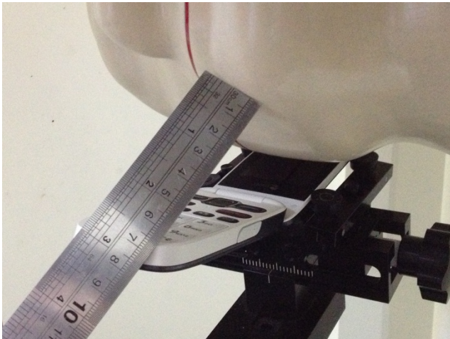
Right Tilted position - Separation distance 6.6cm between mouth and antenna For Sample 1
