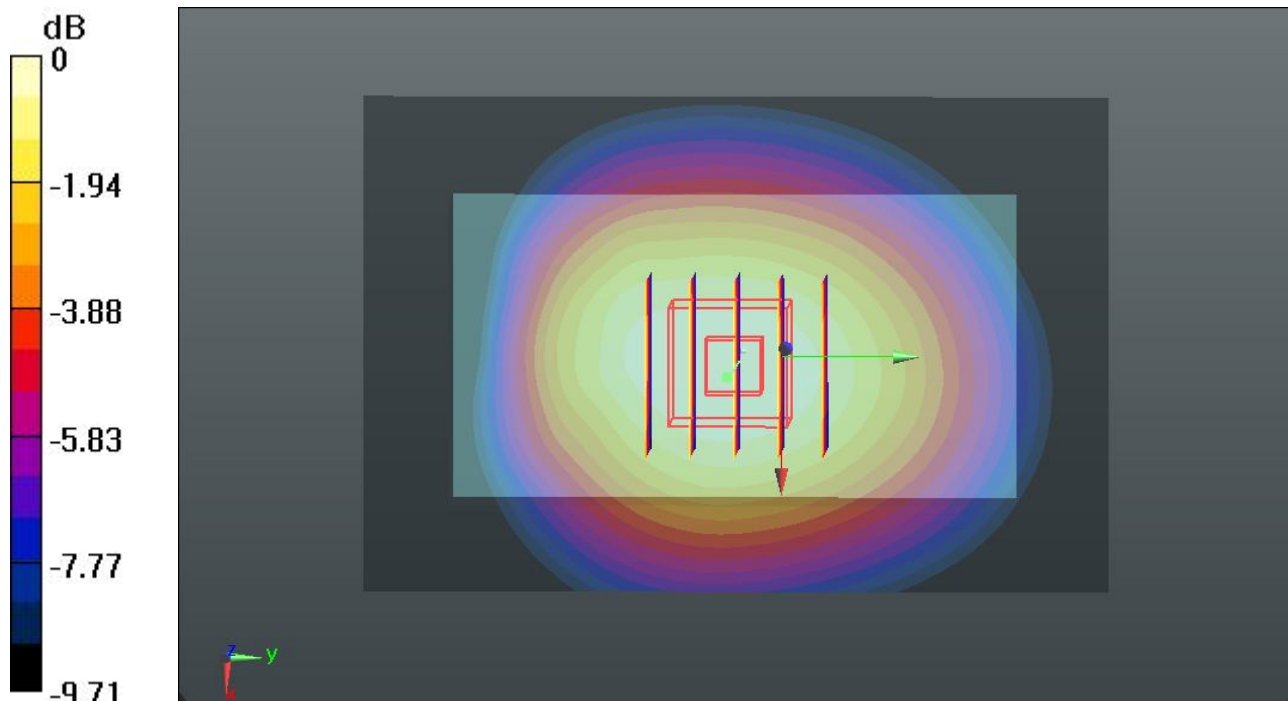
0 dB = 0.825 W/kg
