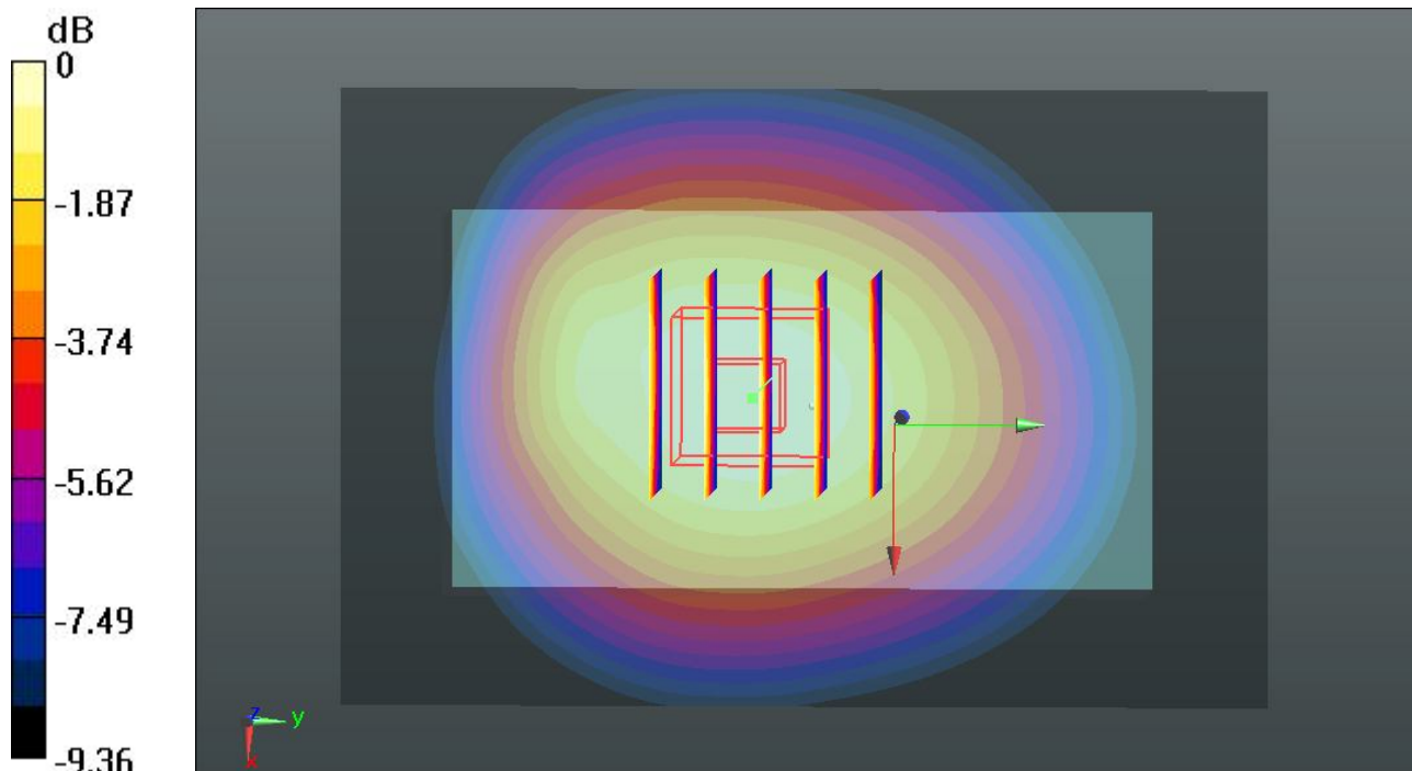
0 dB = 0.472 W/kg
