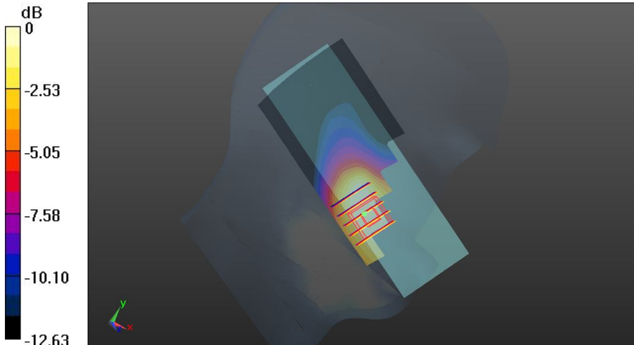
0 dB = 0.475 W/kg
