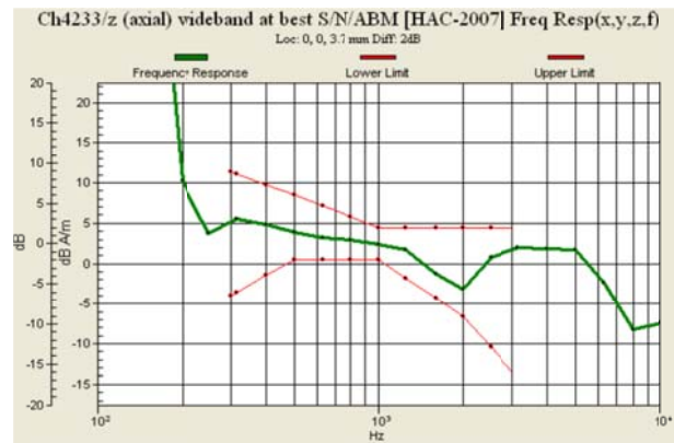
Fig. 9.12 WCDMA Band V Ch4233
