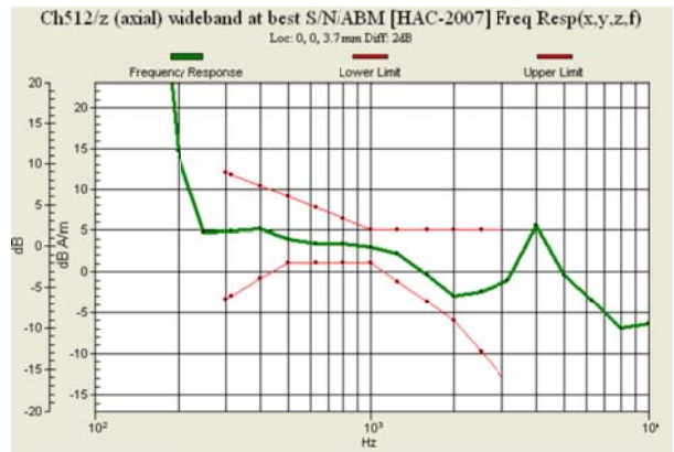
Fig. 9.4 GSM1900 Ch512
