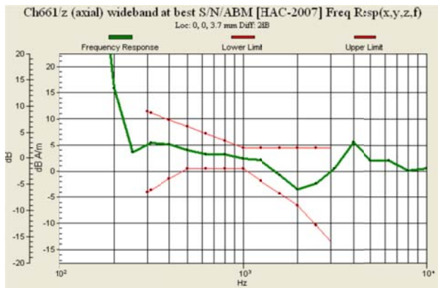
Fig. 9.5 GSM1900 Ch661
