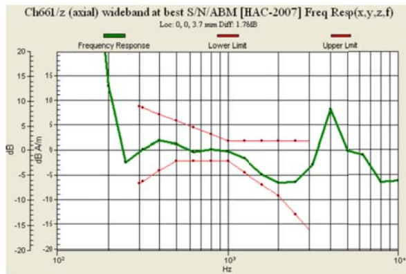
Fig. 9.5 GSM1900 Ch661
