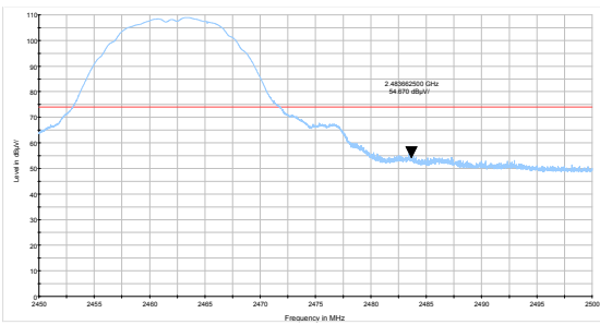
802.11b-Channel 11 Peak
