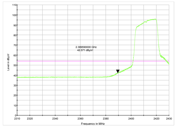
802.11g-Channel 1 Average
