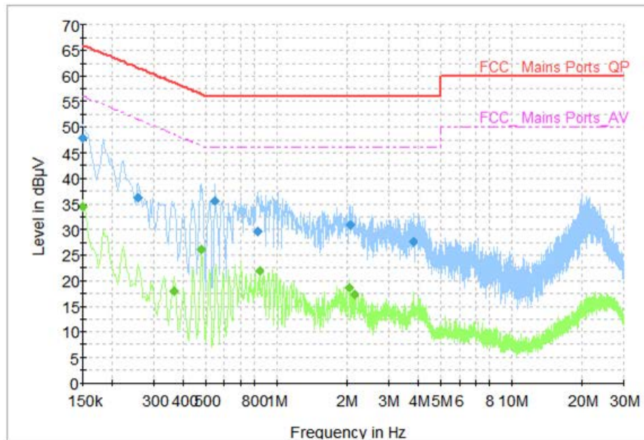
Fig.53 AC Power line Conducted Emission (Idle)
