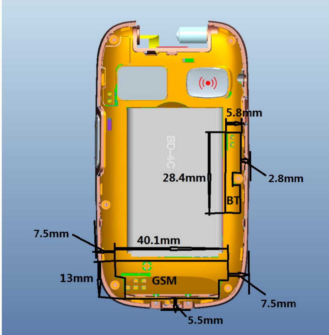
c: Antenna
