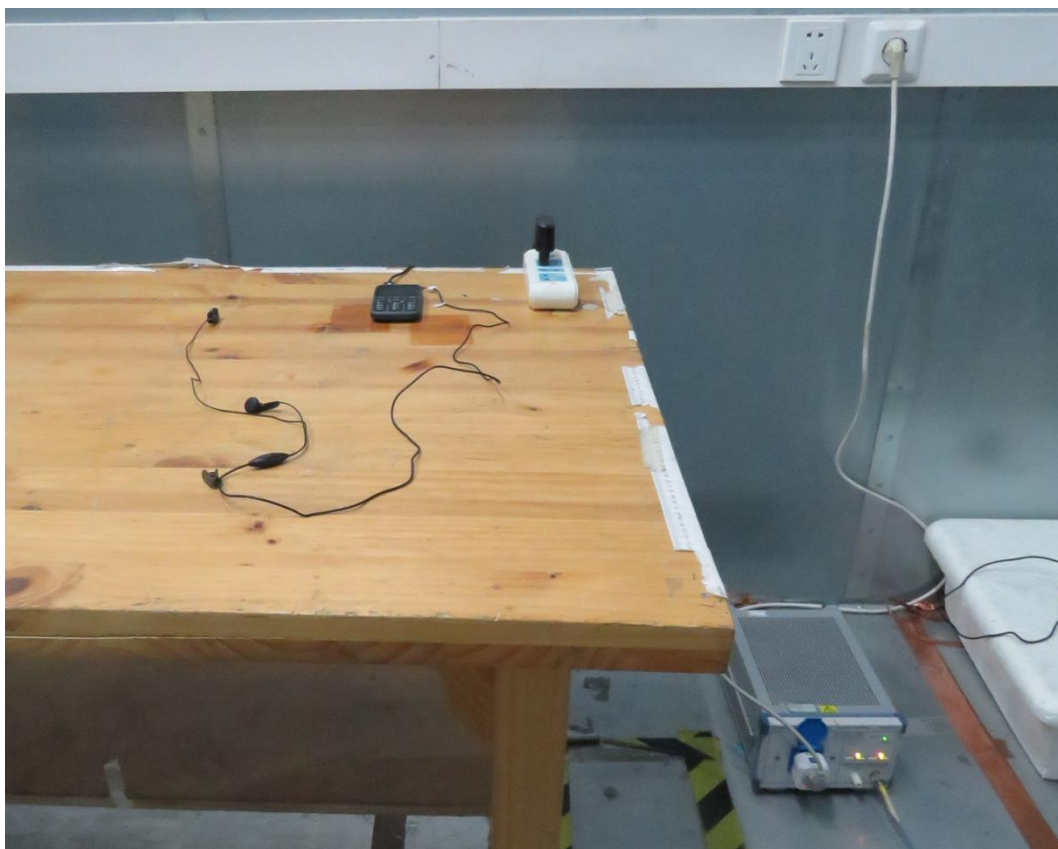
Picture 3 Conducted Emission Test Setup
