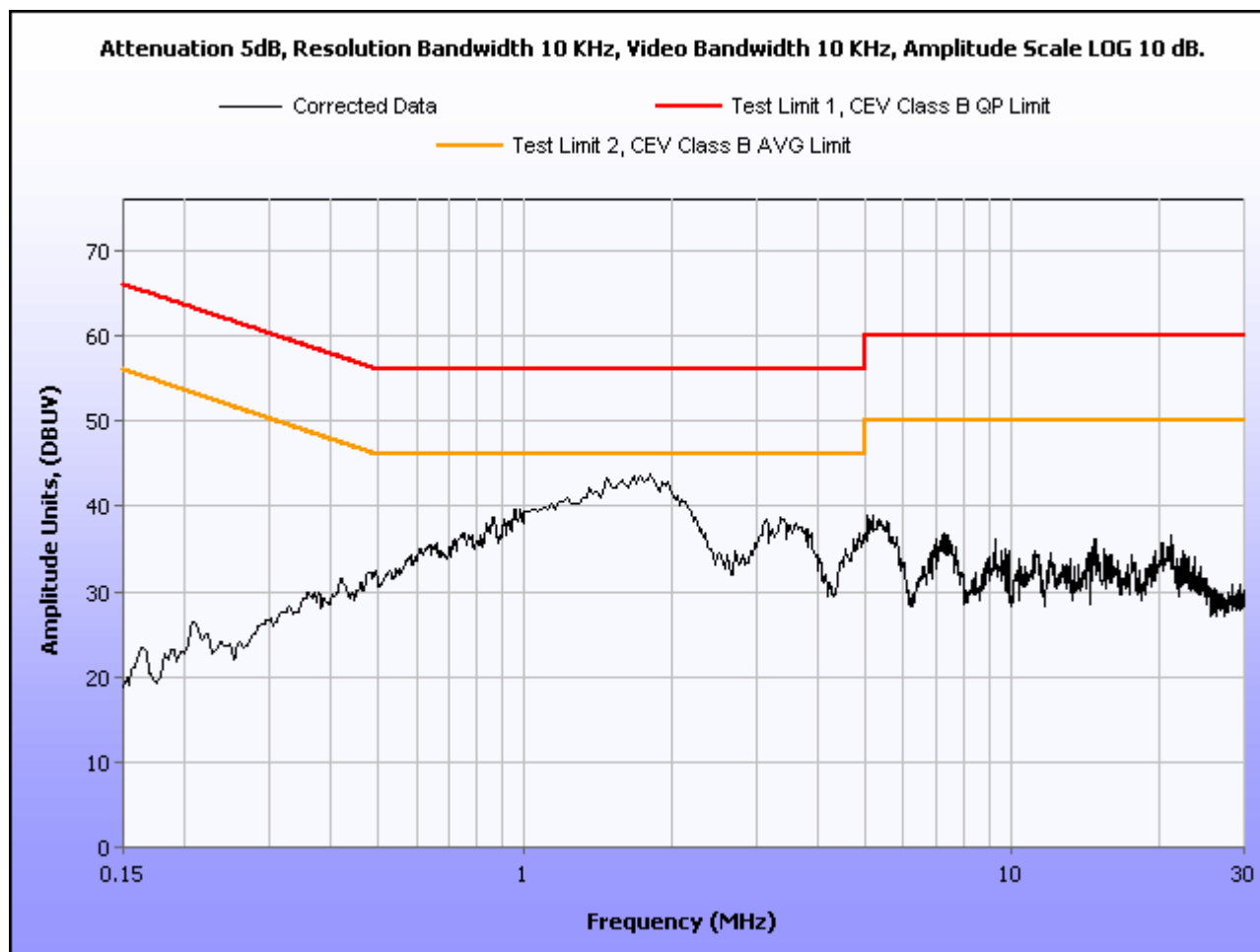
Plot 1. Conducted Emission Limits, Phase Line Plot
