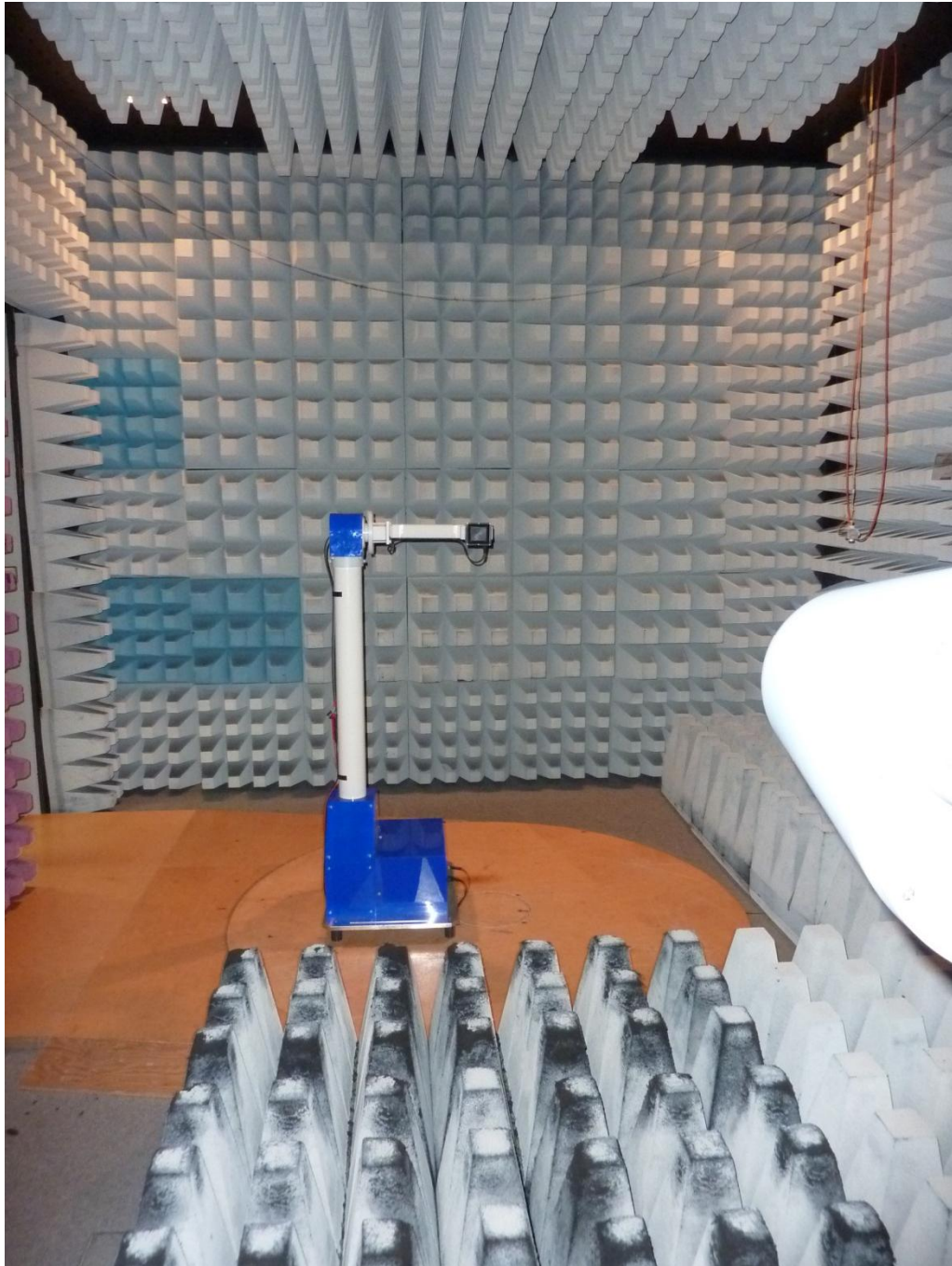
170913_uc.JPG: RMS320-343300, test setup fully anechoic chamber
