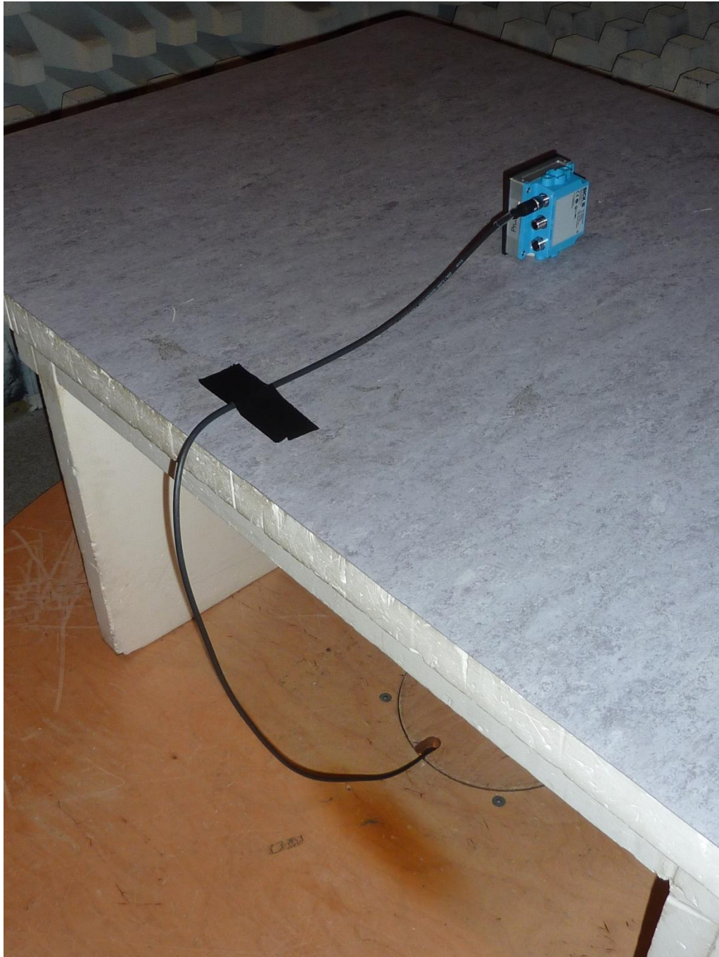
170913_uf.JPG: RMS320-343300, test setup fully anechoic chamber (table, pos. 2)
