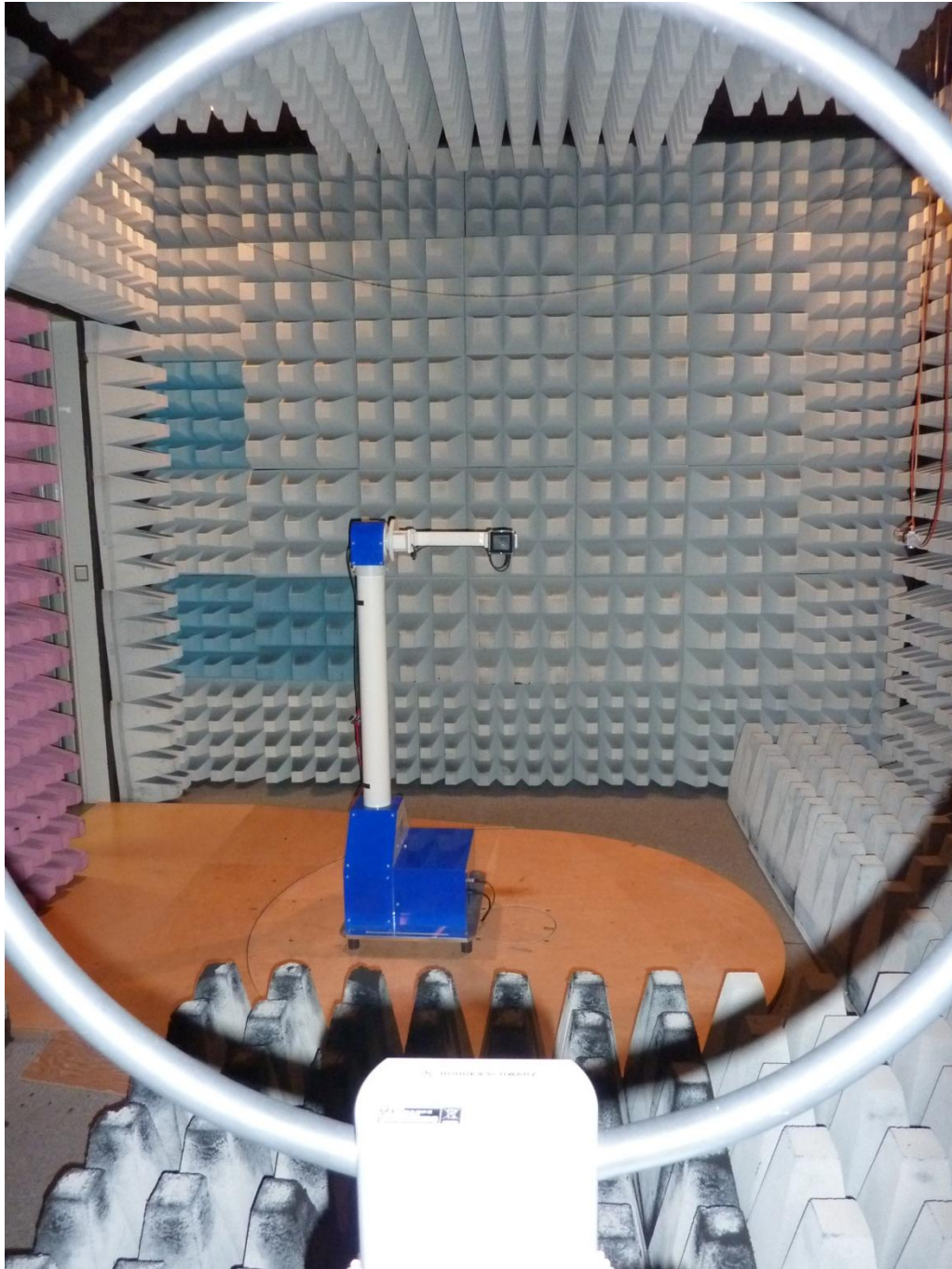
170913_ua.JPG: RMS320-343300, test setup fully anechoic chamber
