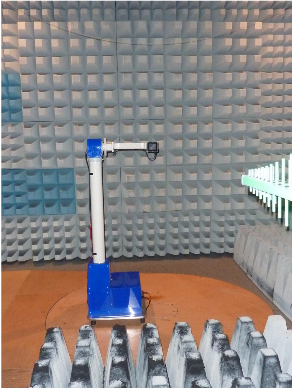
170913_ub.JPG: RMS320-343300, test setup fully anechoic chamber
