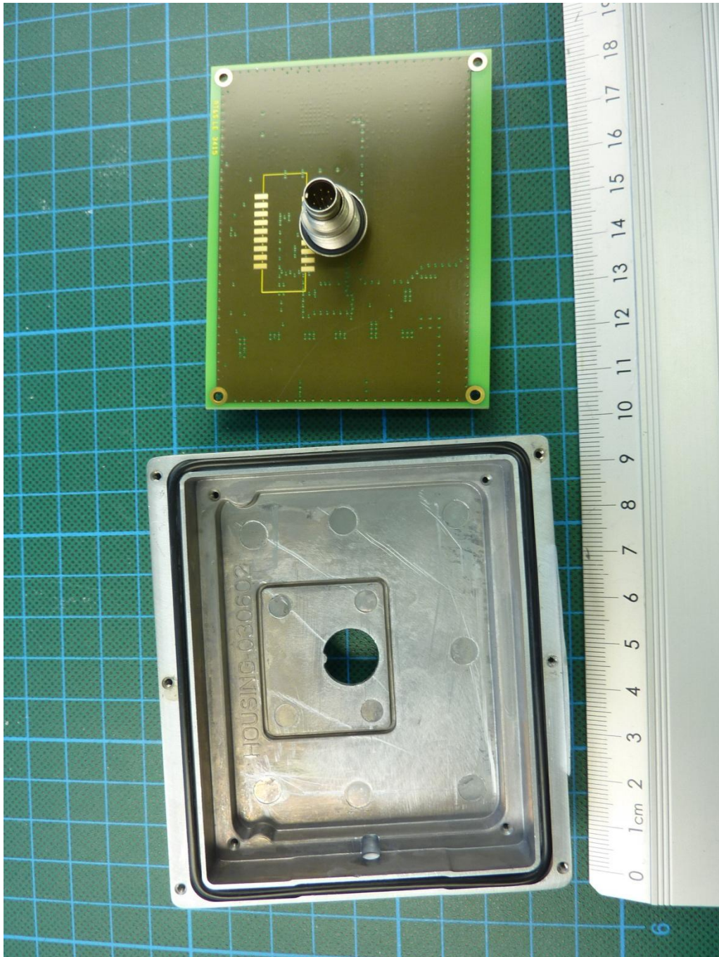
170913_14.JPG: RMS320-343300, radar module, internal view 2
