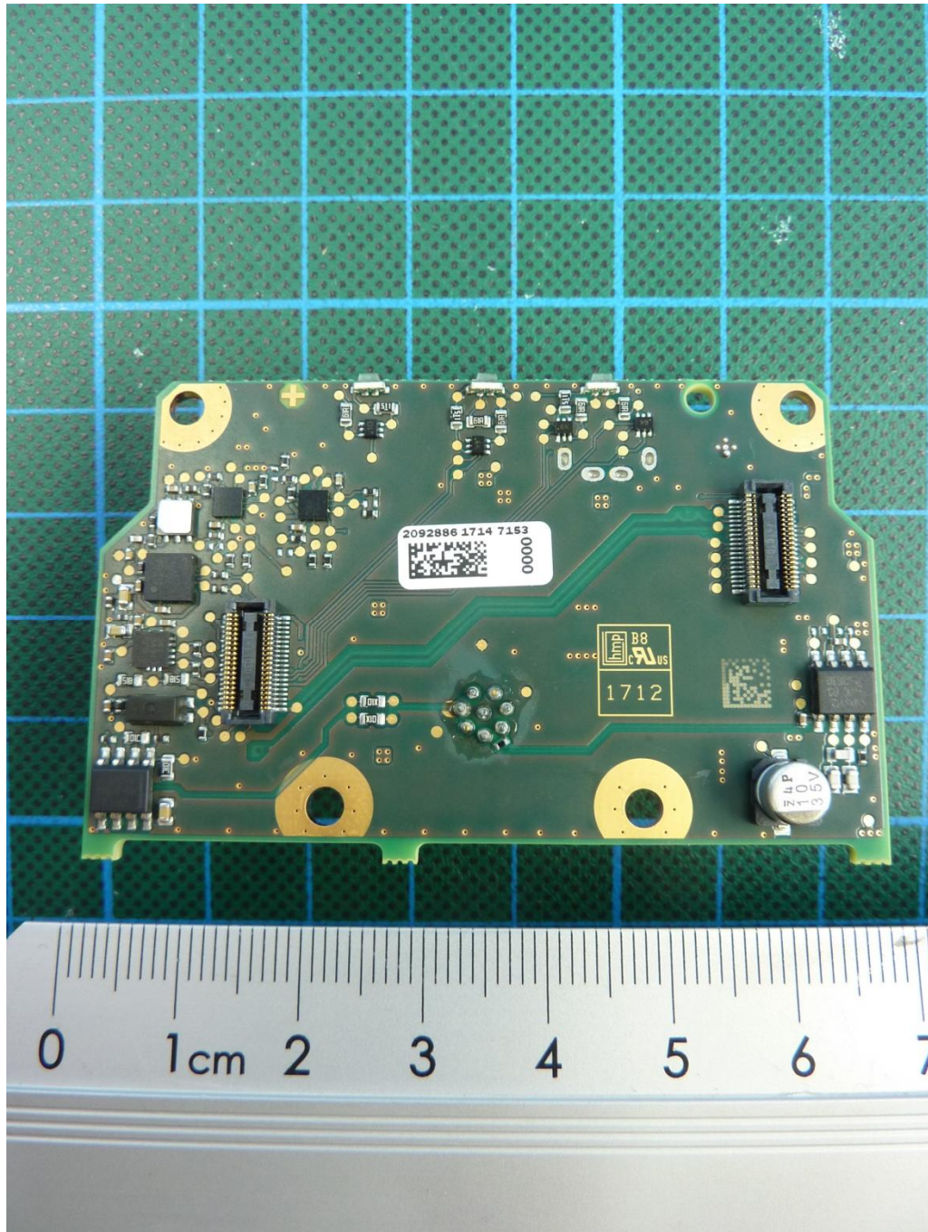
170913_16.JPG: RMS320-343300, PCB 1, bottom view
