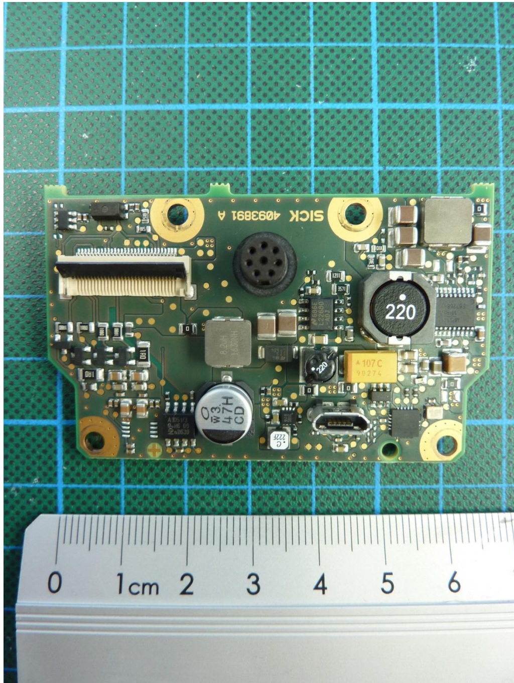
170913_15.JPG: RMS320-343300, PCB 1, top view
