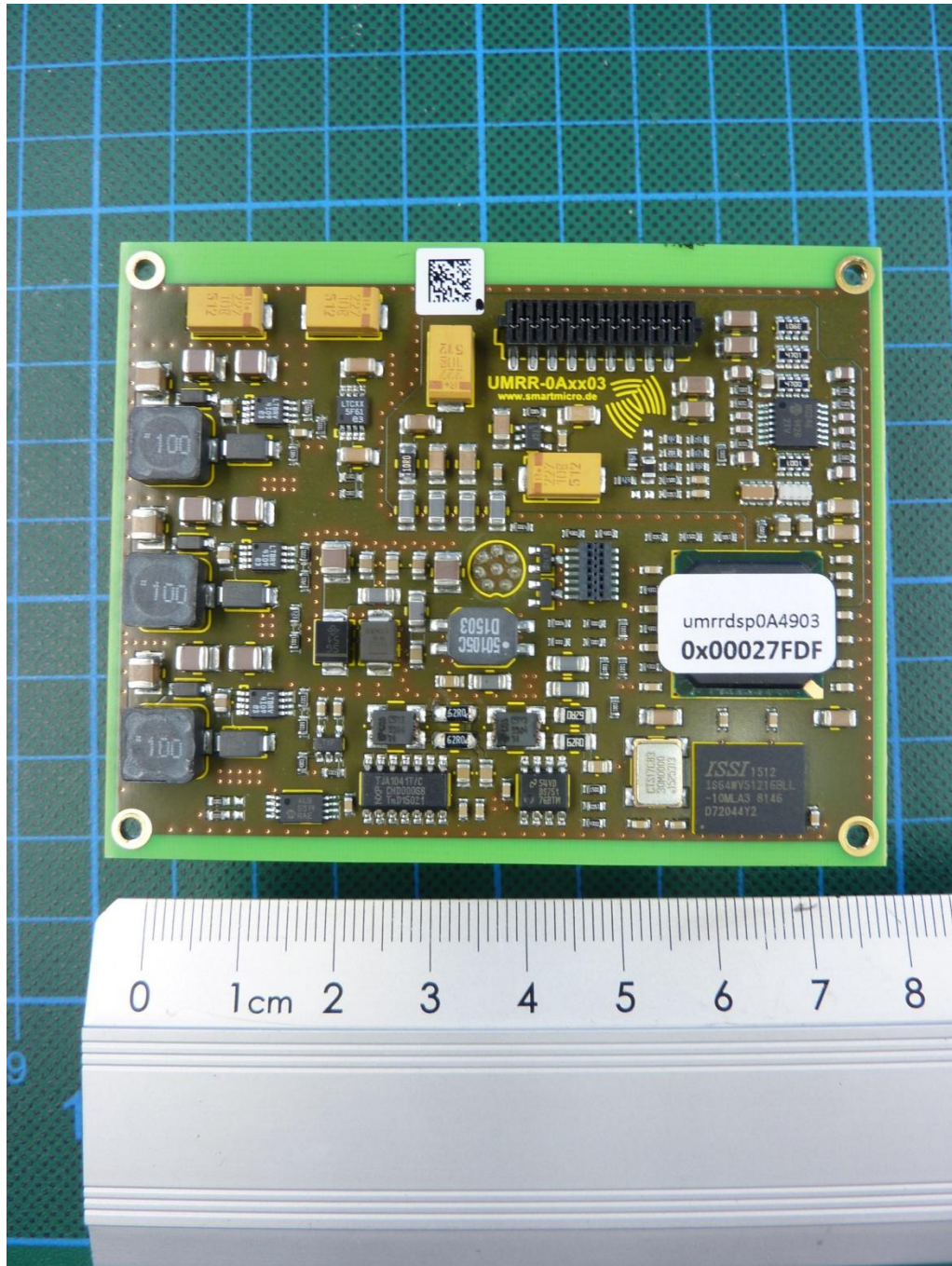
170913_24.JPG: RMS320-343300, radar module, PCB 2, top view
