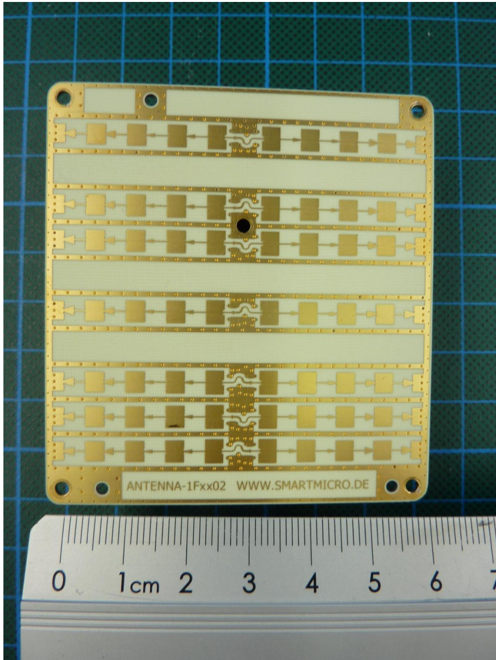
170913_21.JPG: RMS320-343300, radar module, RF-PCB, top view
