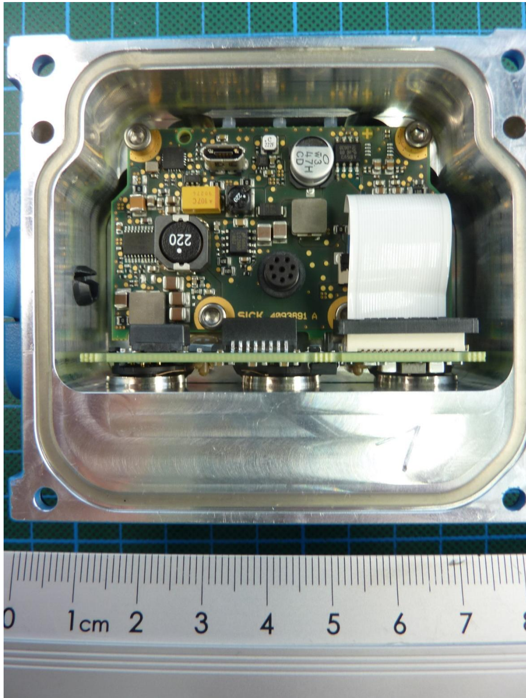
170913_6.JPG: RMS320-343300, internal view 2 (radar module removed)
