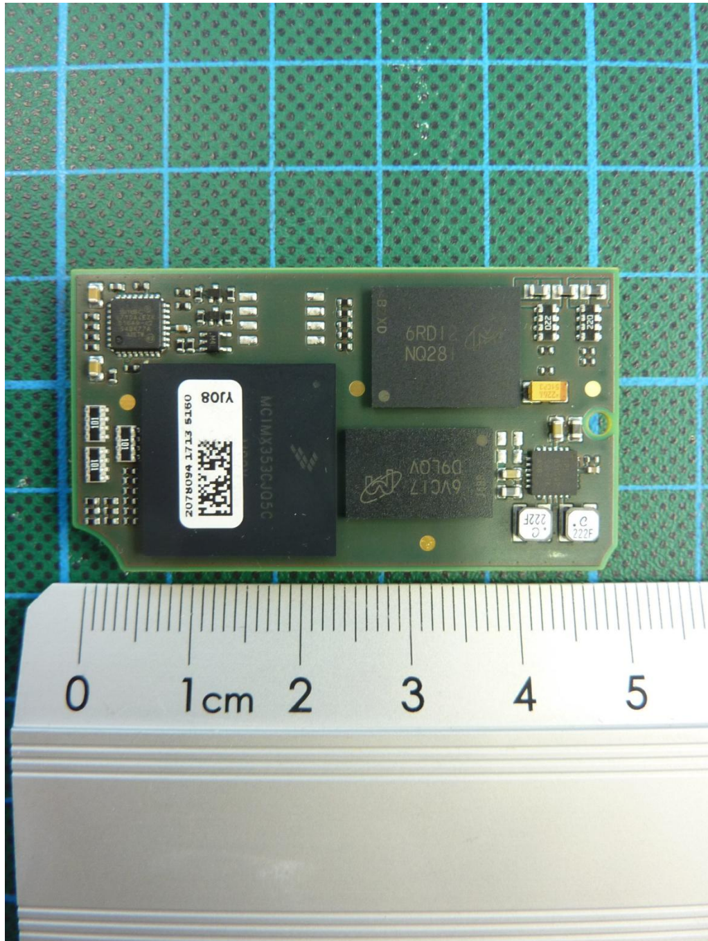
170913_18.JPG: RMS320-343300, PCB 2, bottom view
