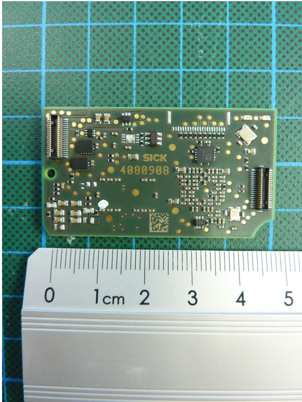
170913_17.JPG: RMS320-343300, PCB 2, top view
