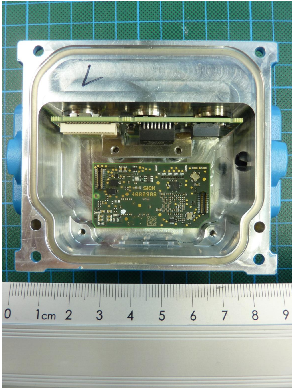
170913_8.JPG: RMS320-343300, internal view 3 (radar module and PCB 1 removed)
