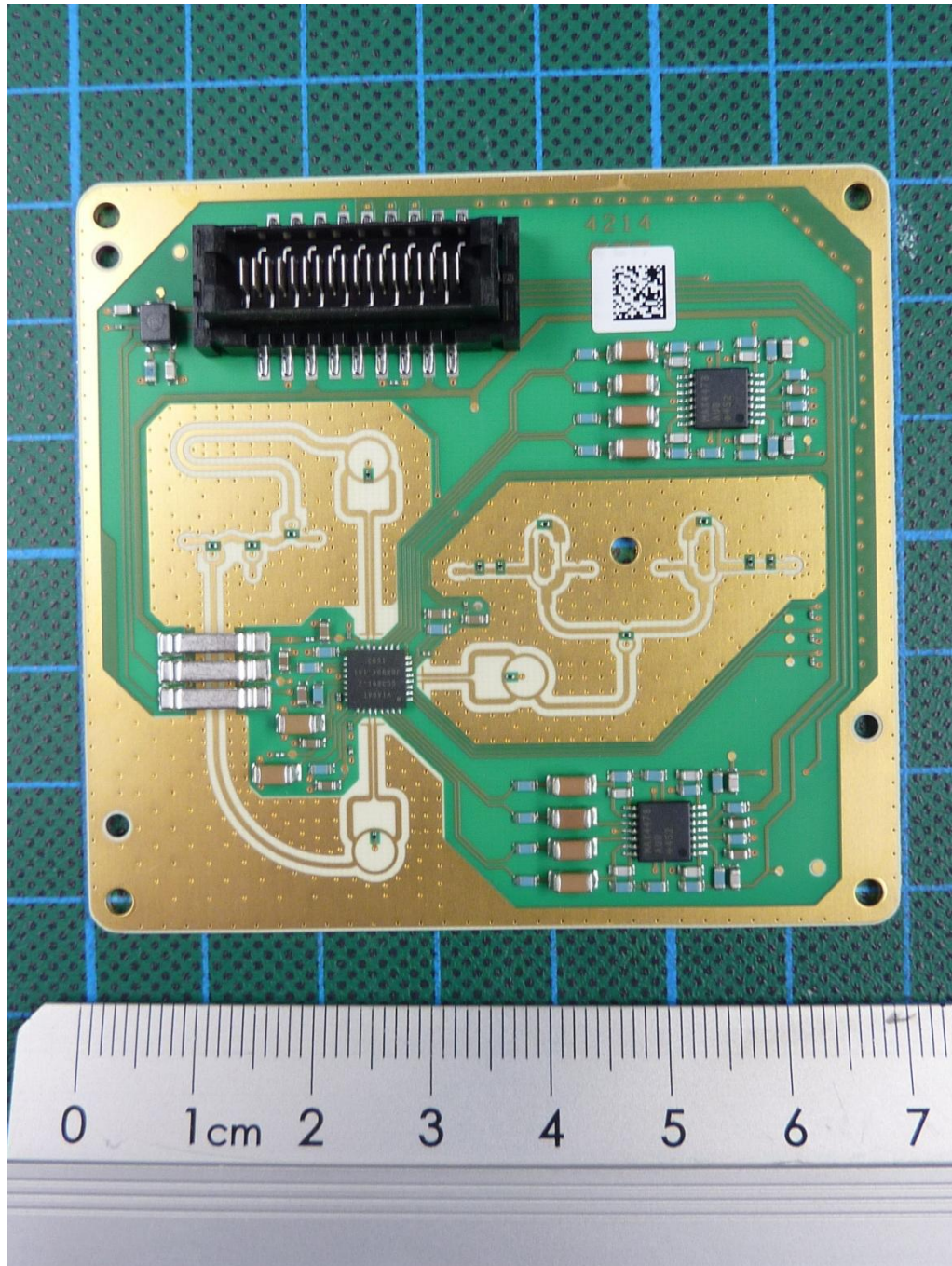
170913_22.JPG: RMS320-343300, radar module, RF-PCB, bottom view
