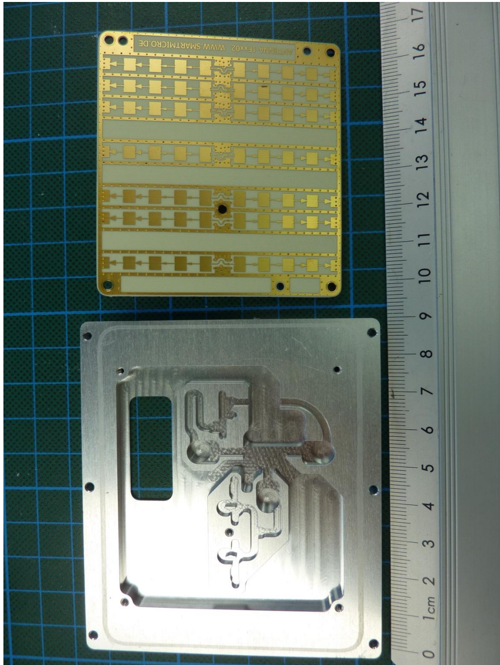
170913_13.JPG: RMS320-343300, radar module, internal view 1
