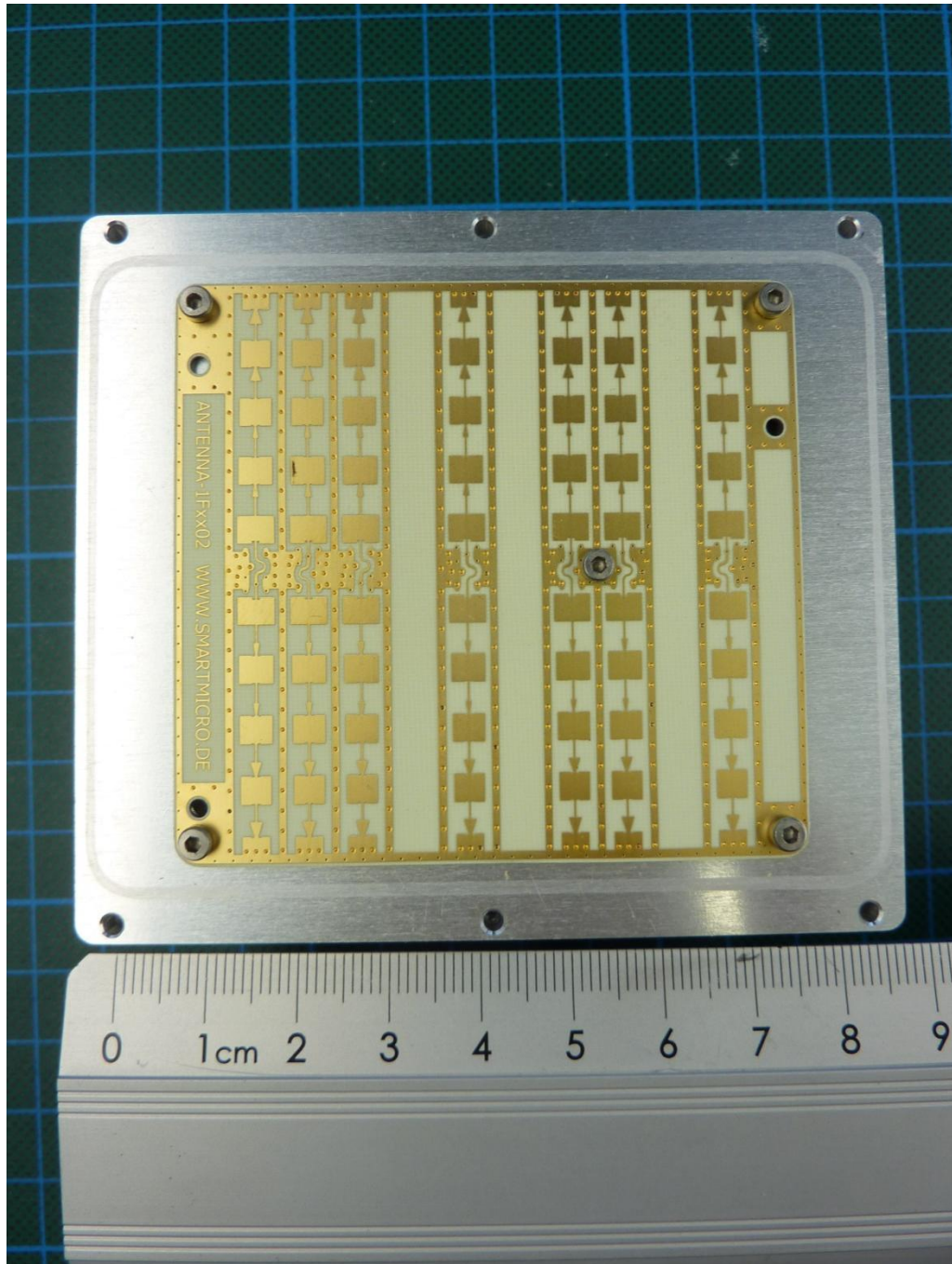
170913_12.JPG: RMS320-343300, radar module, front housing removed
