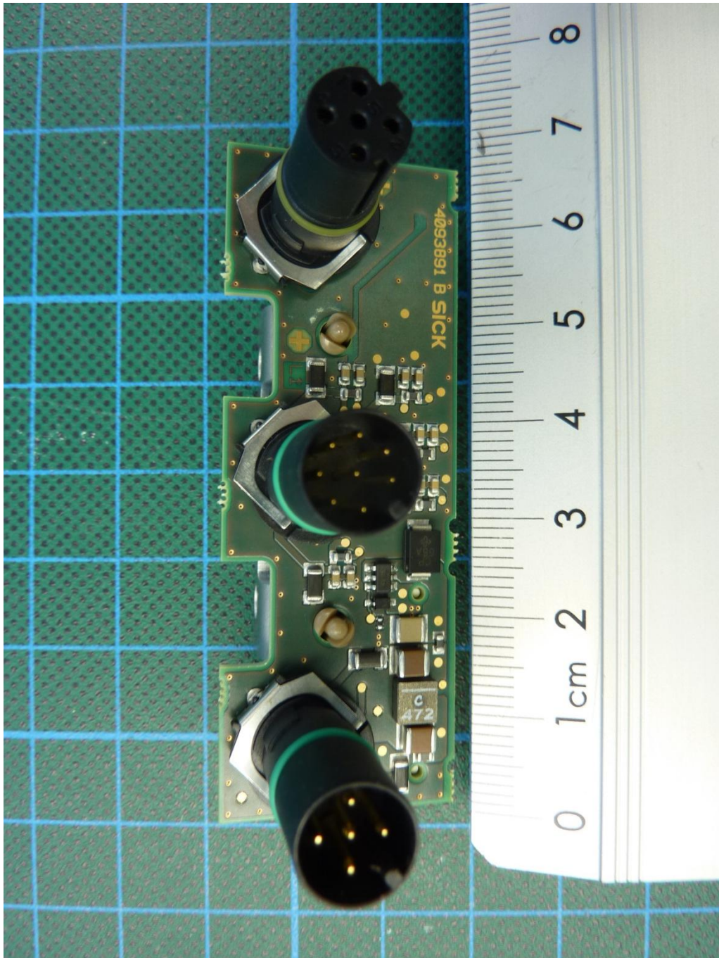
170913_20.JPG: RMS320-343300, PCB 3, bottom view
