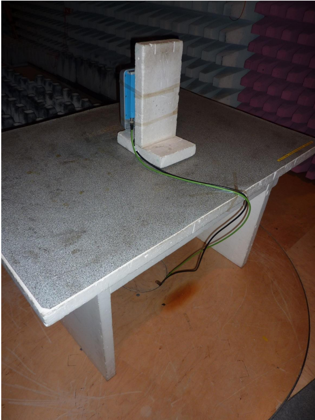
135012_a.JPG: RFU630, test set-up fully anechoic chamber
