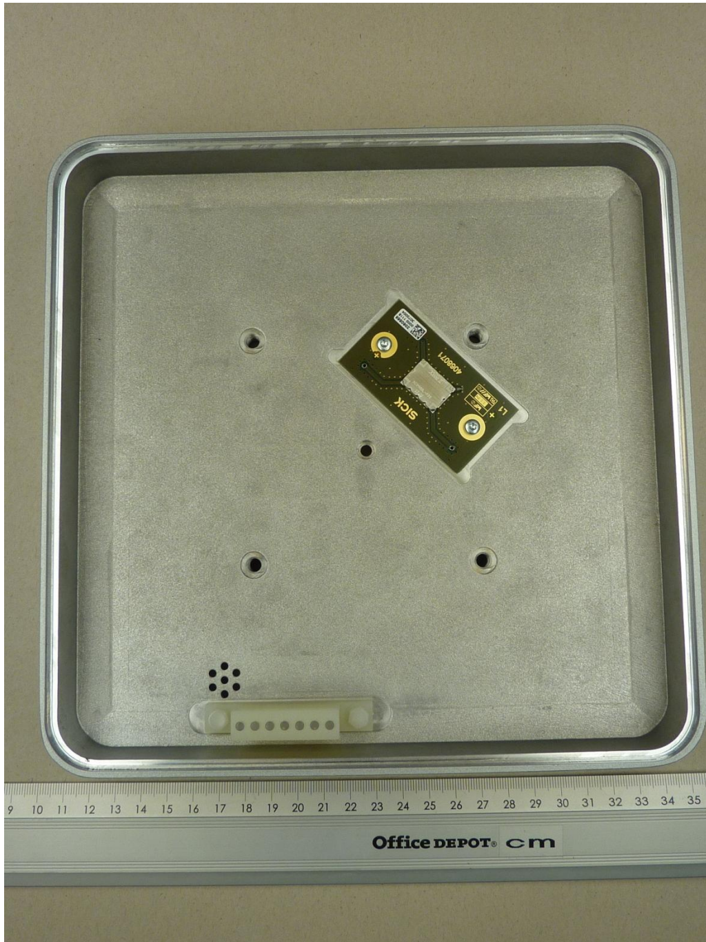
135012_14.JPG: RFU630, internal view 3 (antenna removed)
