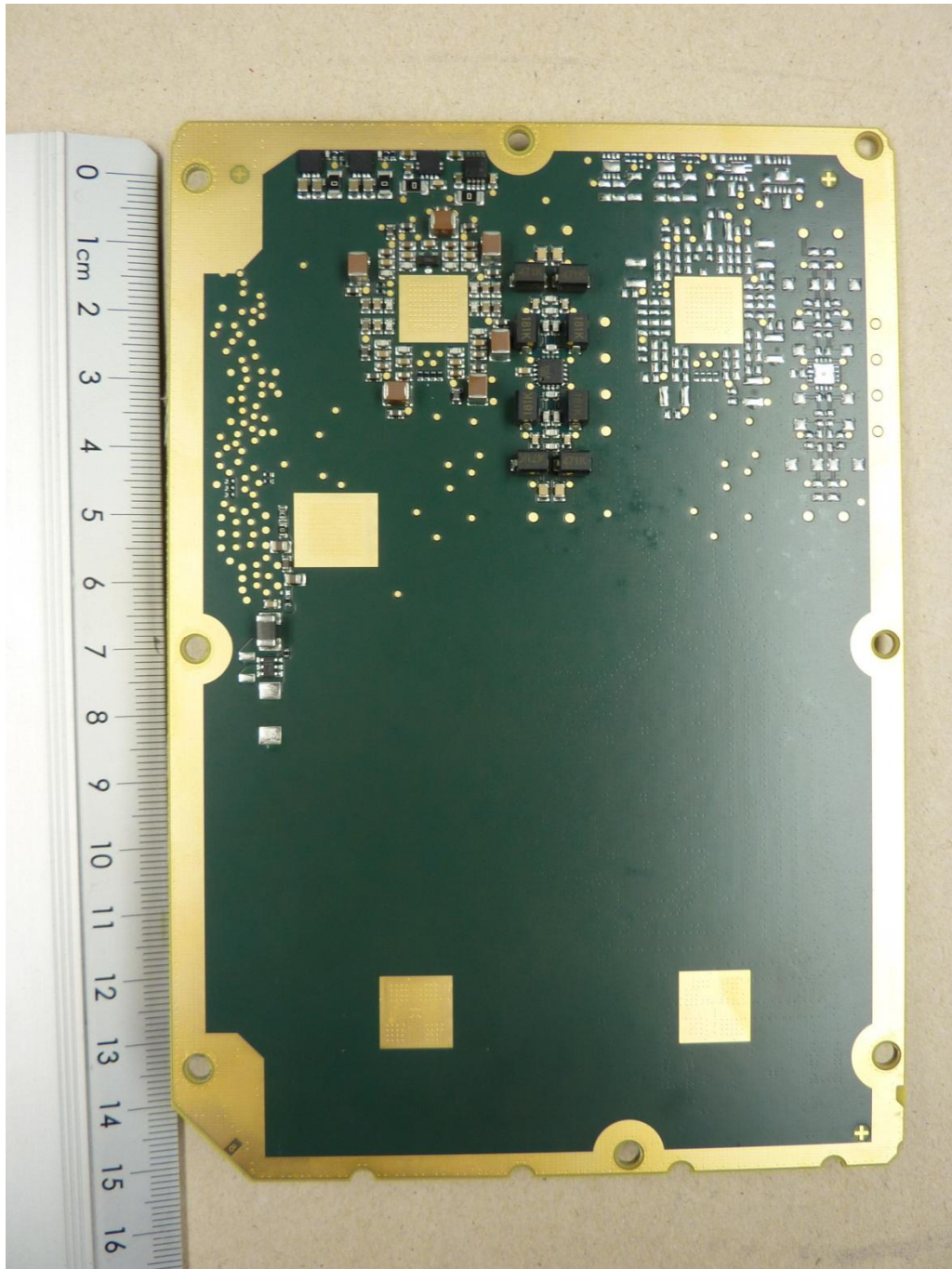
135012_10.JPG: RFU630, PCB 2 bottom view
