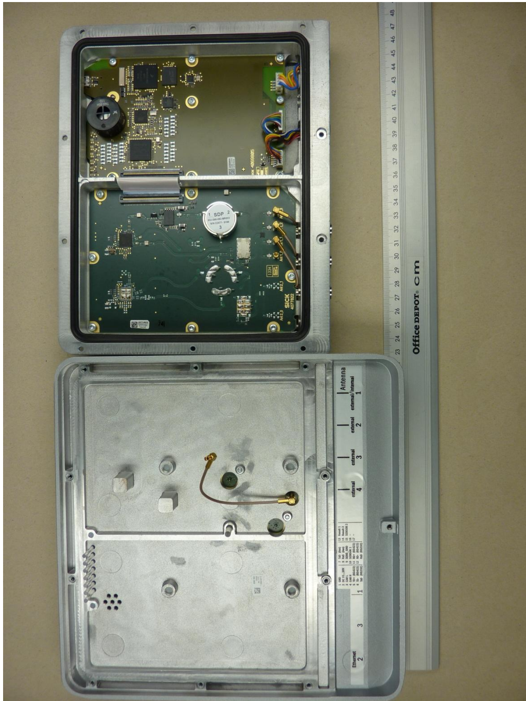
135012_5.JPG: RFU630, internal view 1
