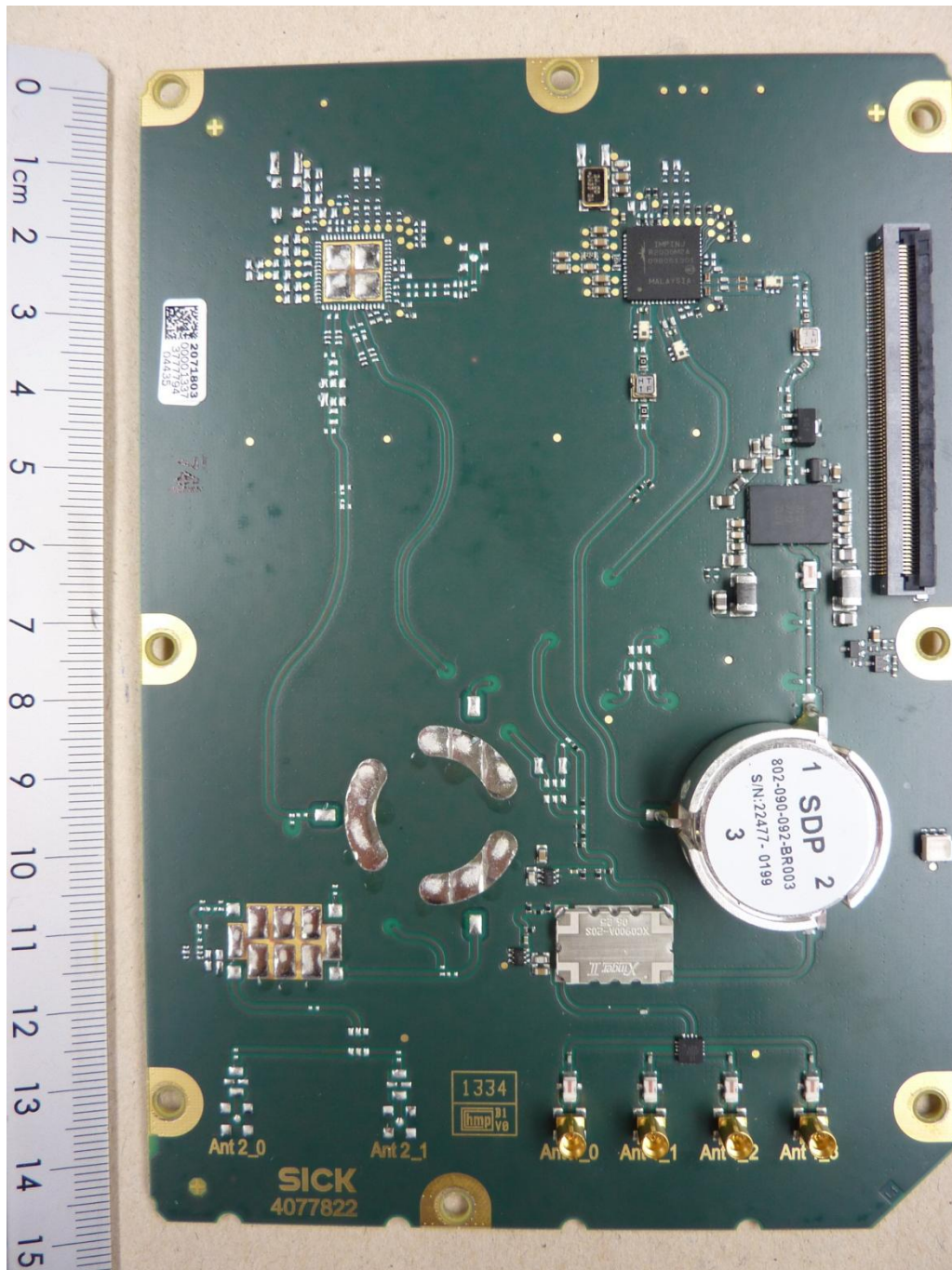
135012_11.JPG: RFU630 PCB 2, top view
