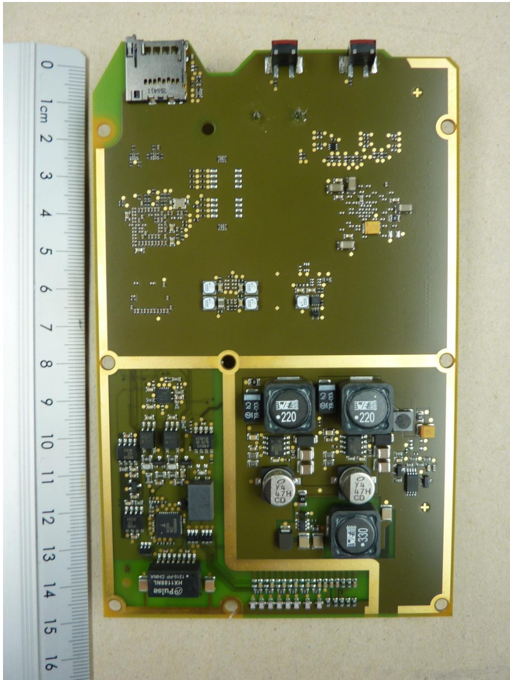
135012_8.JPG: RFU630, PCB 1 bottom view
