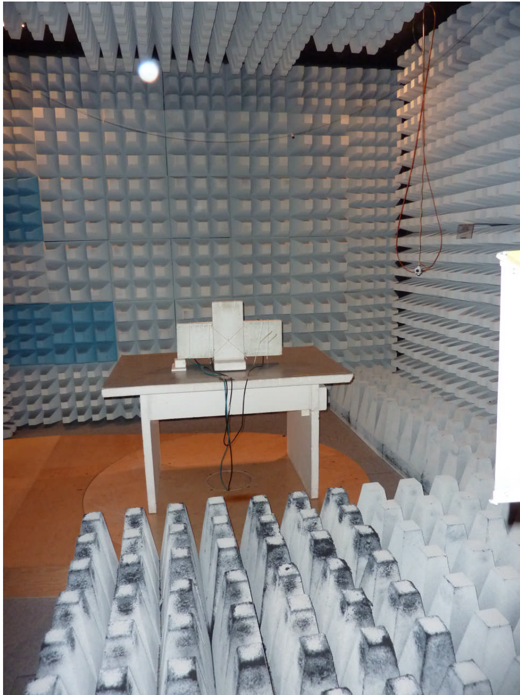
113961_y.JPG: EUT with external ULORA antenna, test set-up fully anechoic chamber
