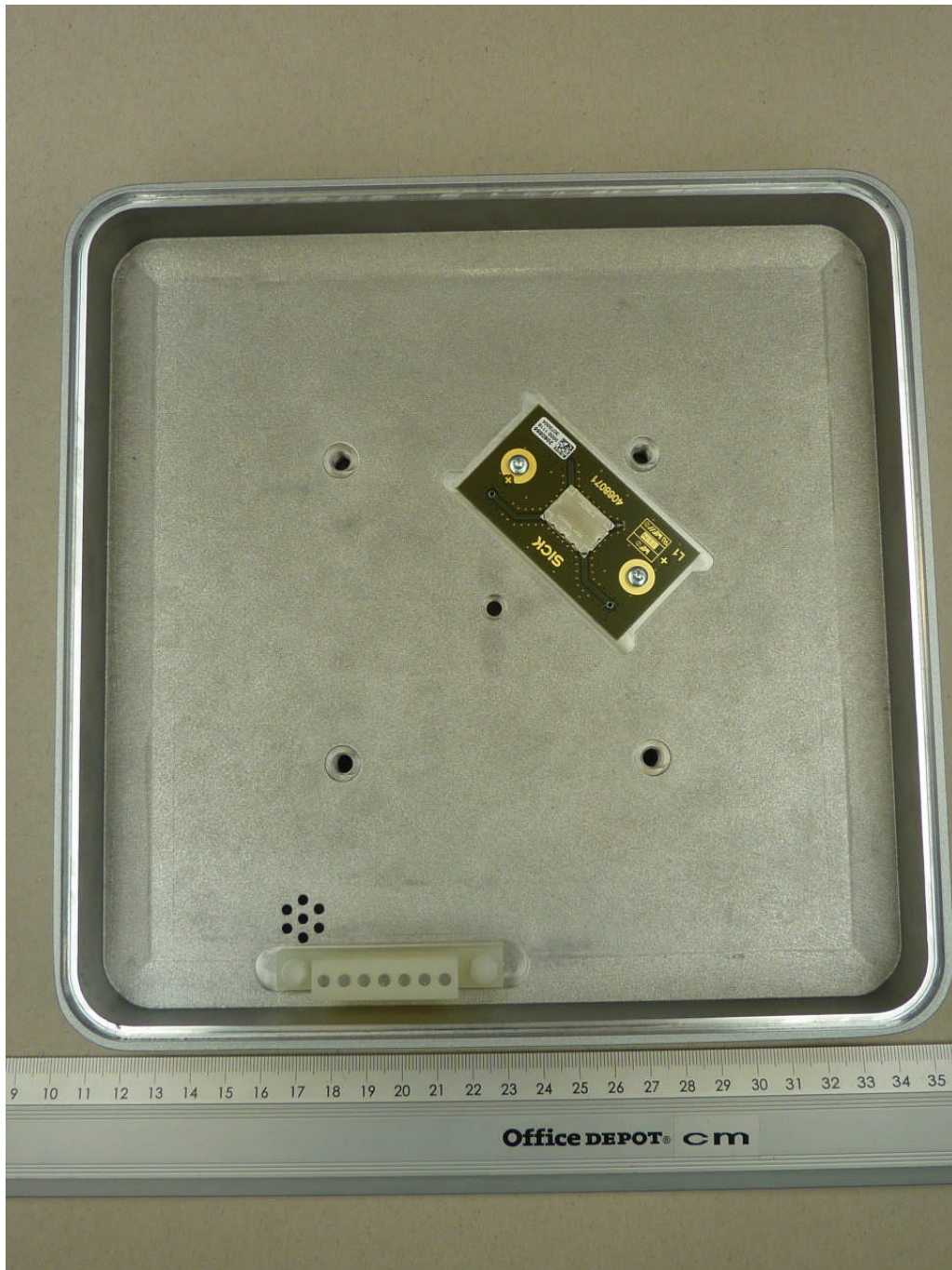
113961_23.JPG: RFU630, internal view 4
