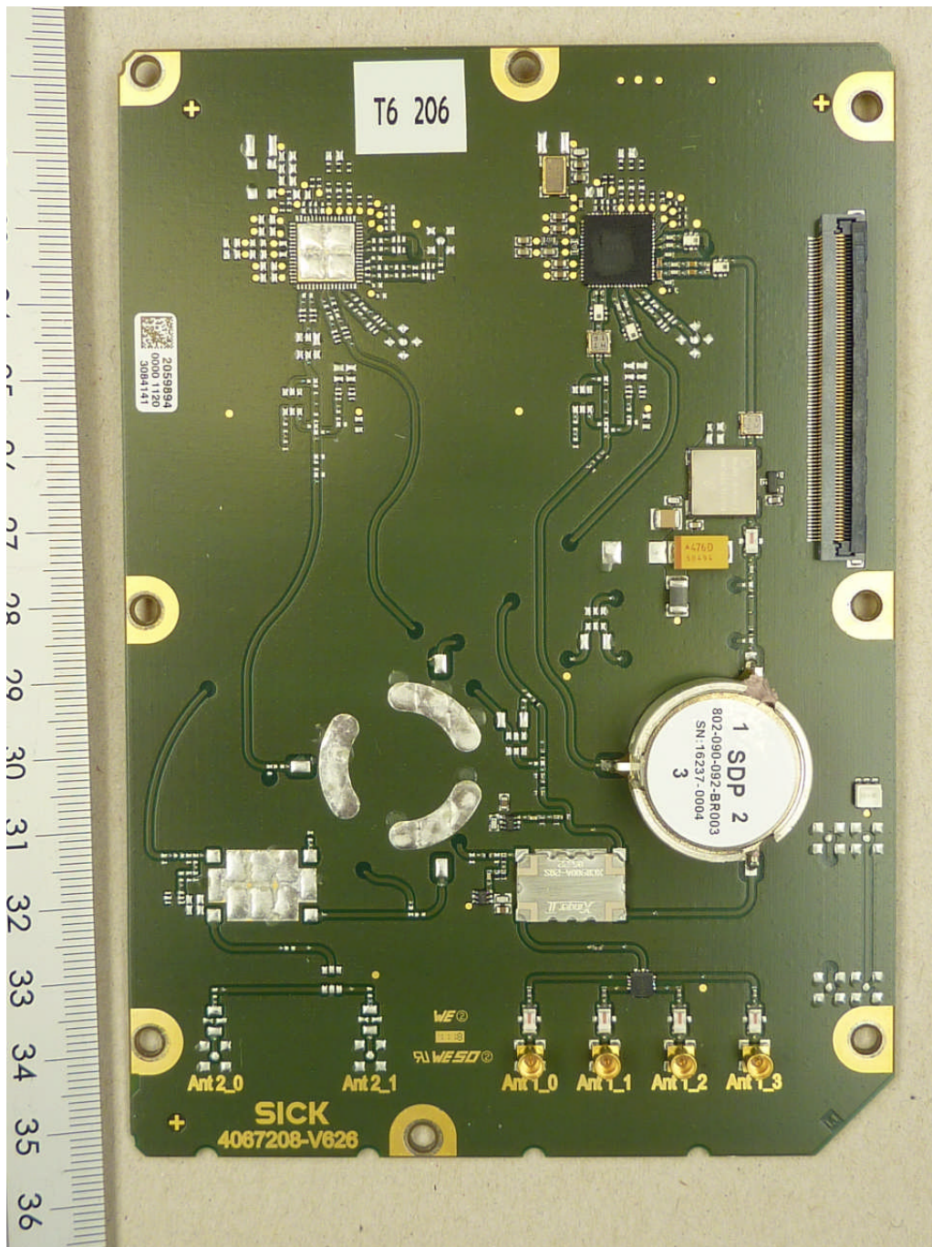
113961_20.JPG: RFU630, PCB 2, top view
