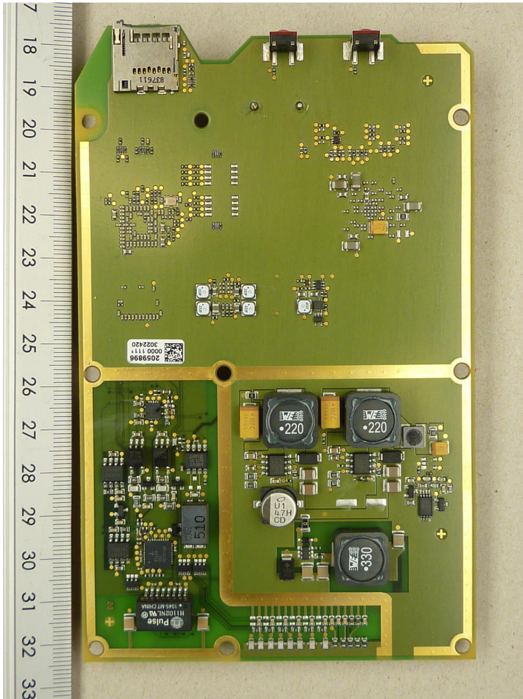
113961_18.JPG: RFU630, PCB 1, bottom view
