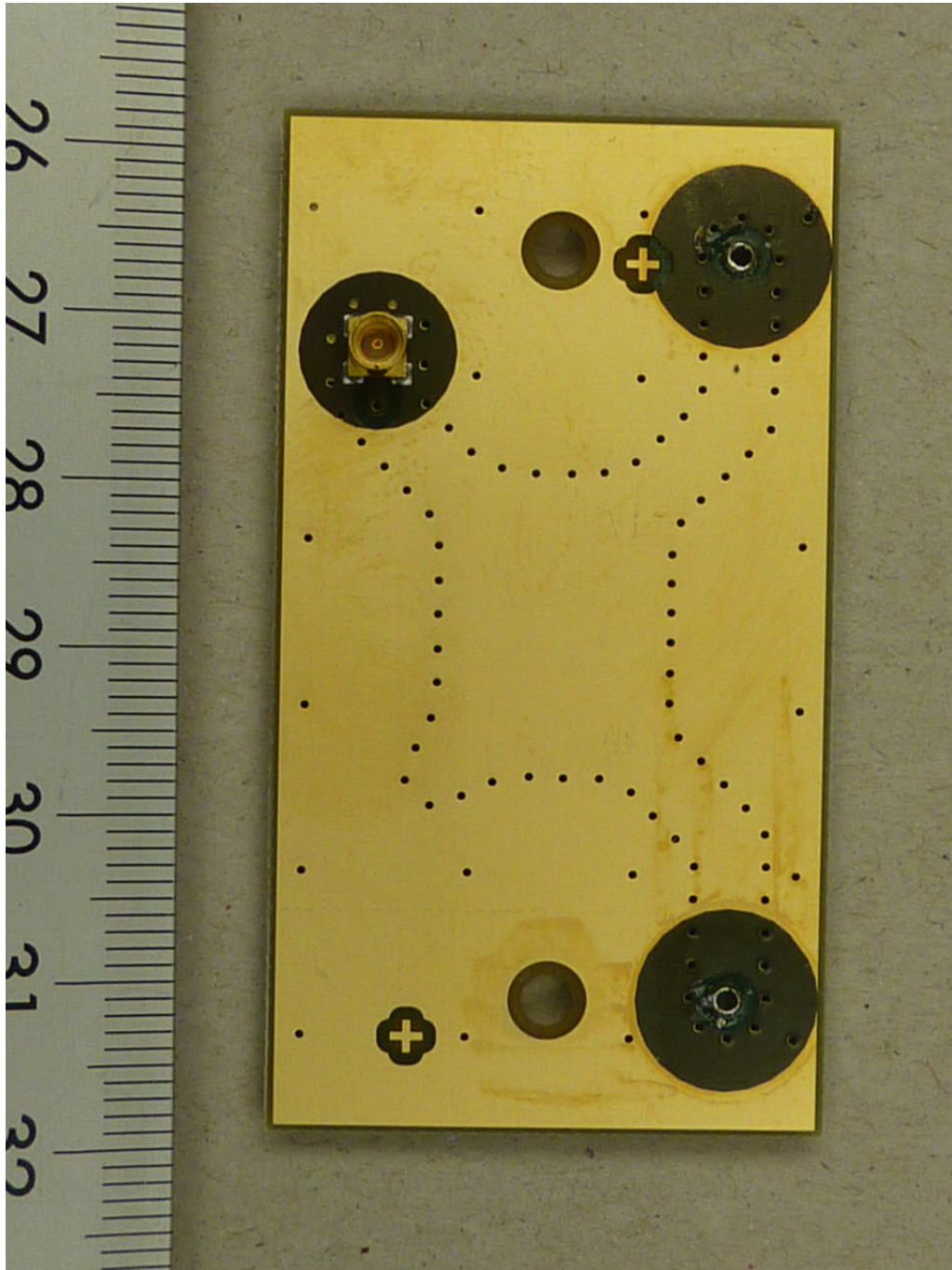
113961_25.JPG: RFU630, PCB 3, bottom view
