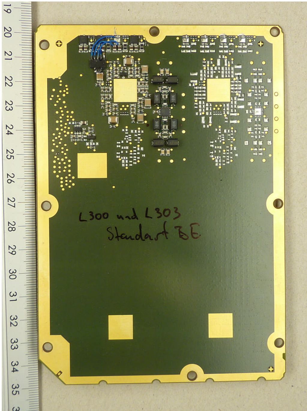
113961_21.JPG: RFU630, PCB 2, bottom view
