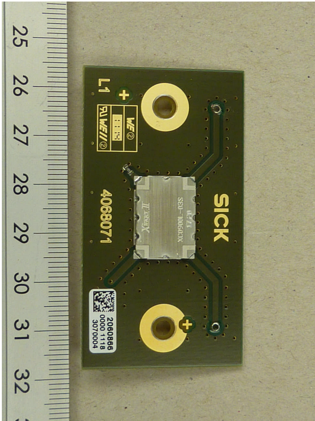
113961_24.JPG: RFU630, PCB 3, top view
