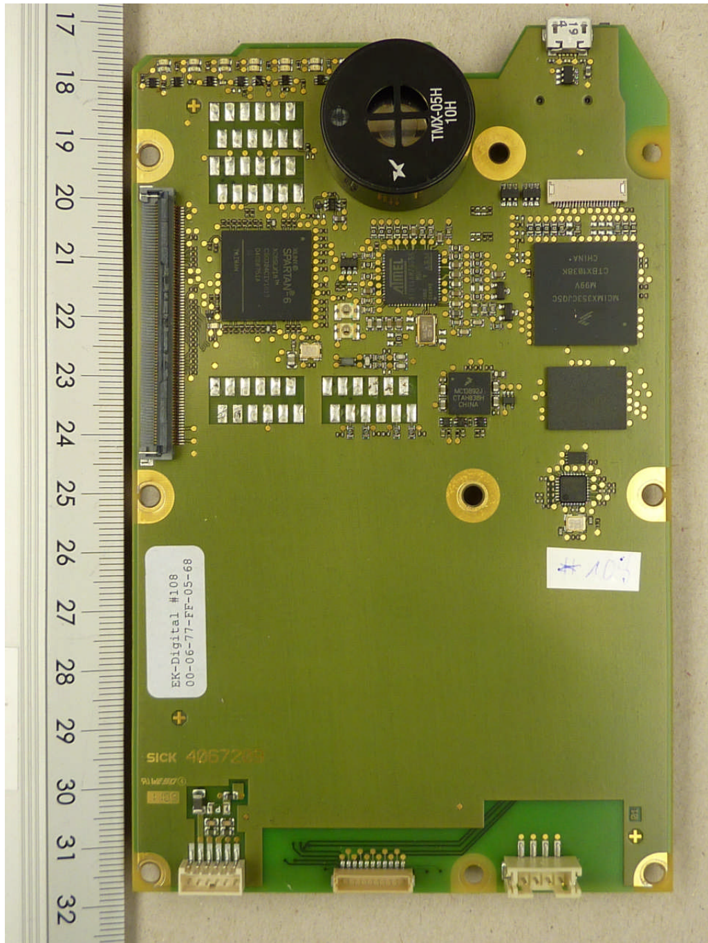
113961_19.JPG: RFU630, PCB 1, top view
