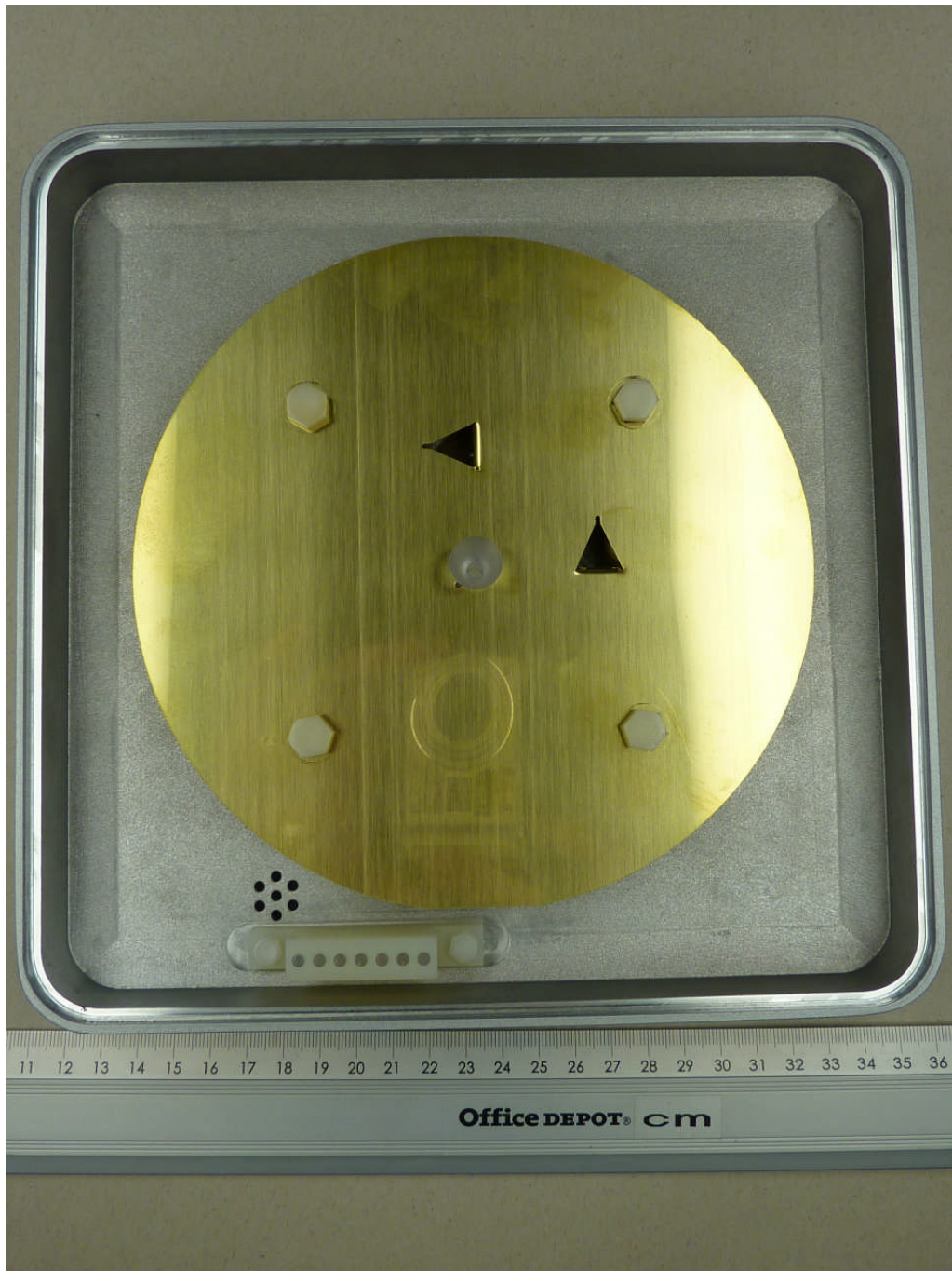
113961_22.JPG: RFU630, internal view 3
