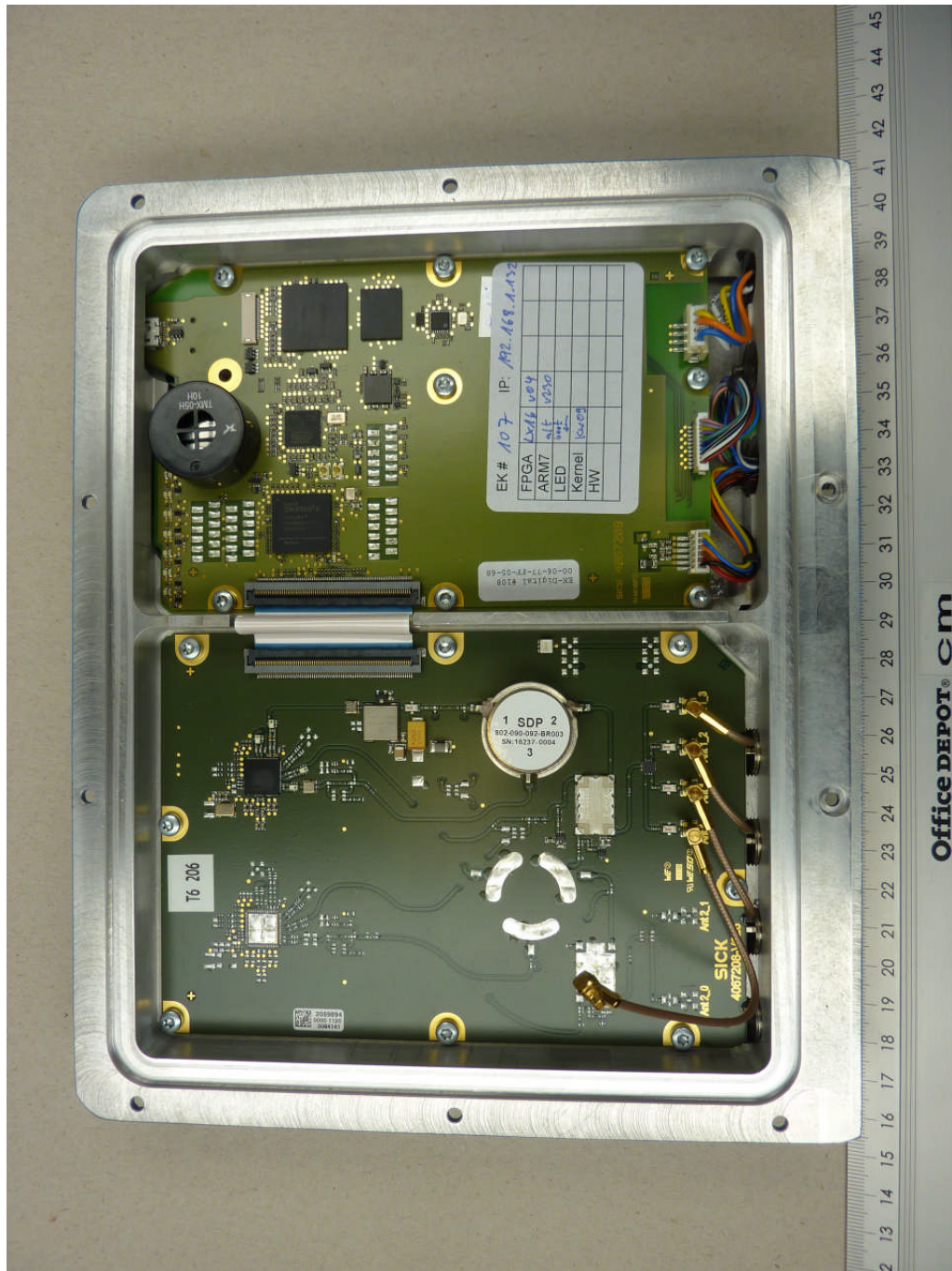
113961_15.JPG: RFU630, internal view 1
