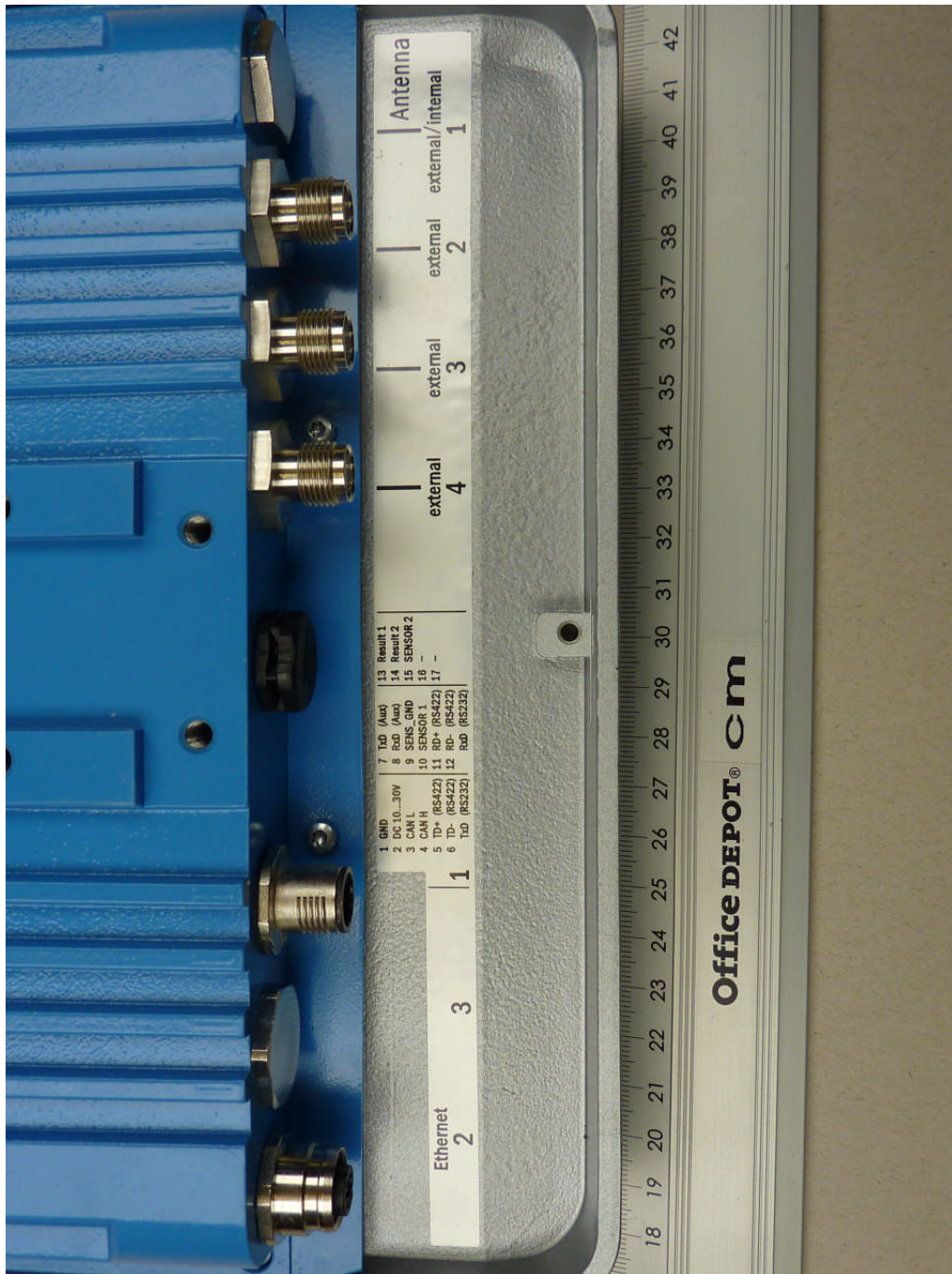
113961_13.JPG: RFU630, connector view
