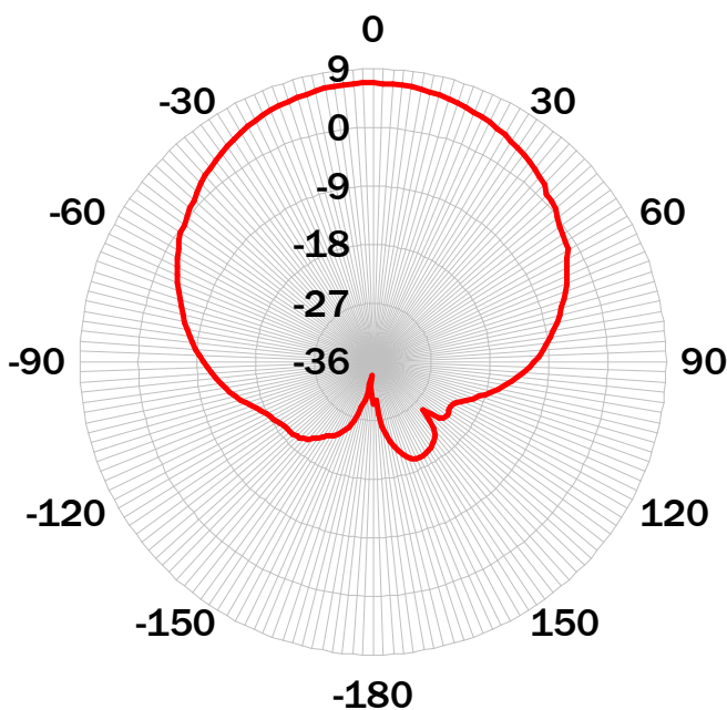
RADIATION PATTERN (915 MHz)
