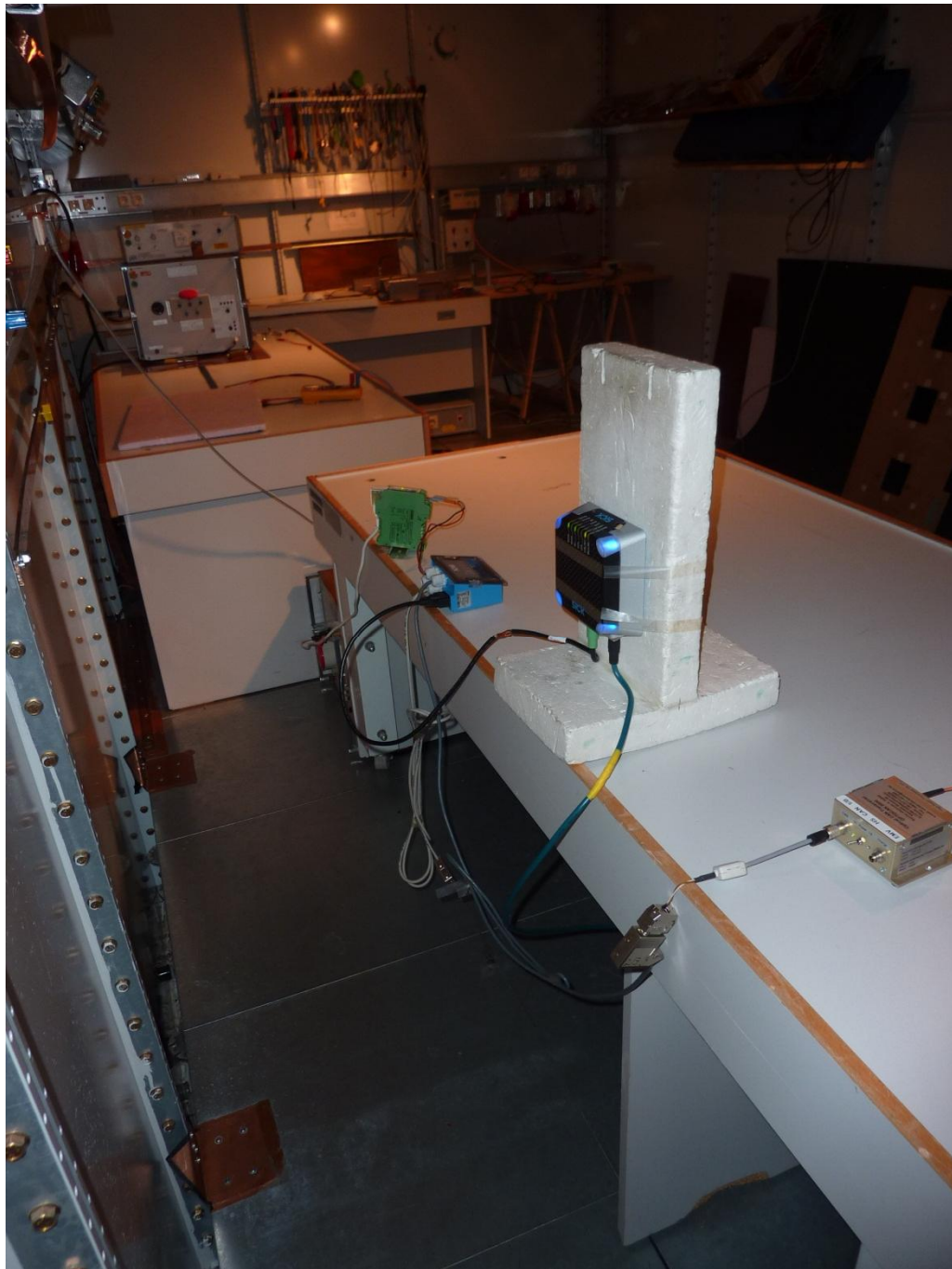
131992_13.JPG: RFU620-10101, test set-up shielded chamber
