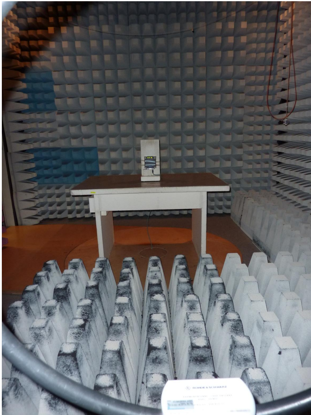
131991_5.JPG: RFU620-10501, test set-up fully anechoic chamber
