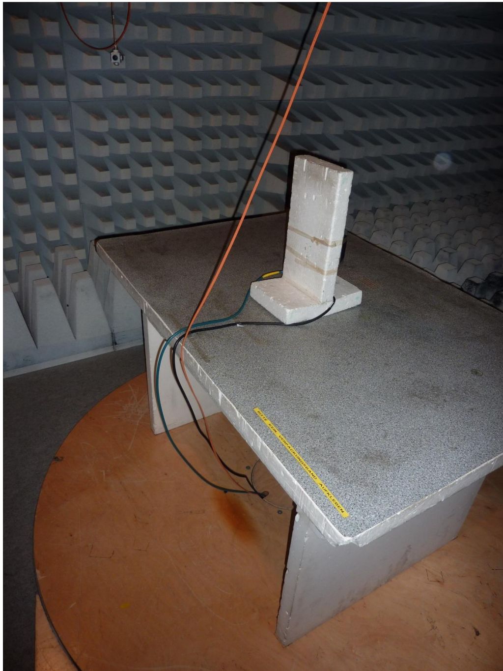
131992_6.JPG: RFU620-10101, test set-up fully anechoic chamber
