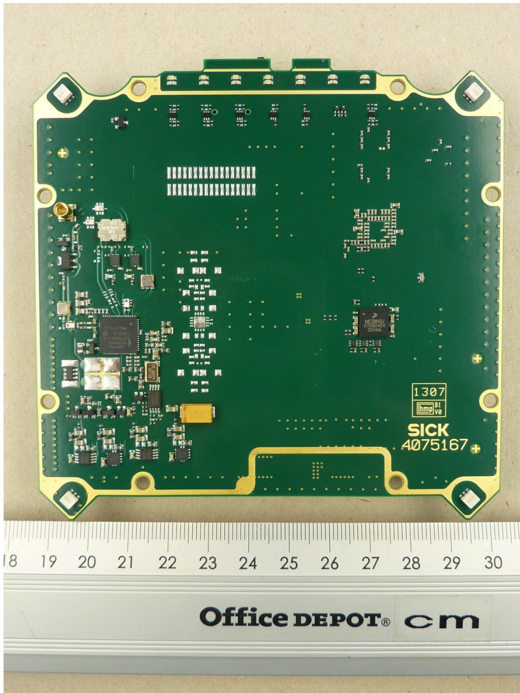
131992_h.JPG: RFU620-10101, EK-System PCB, bottom view
