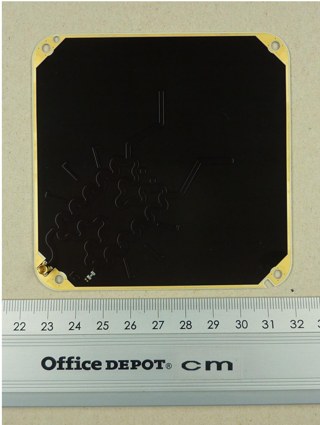
131991_i.JPG: RFU620-10501, EK-Koppler PCB, bottom view
