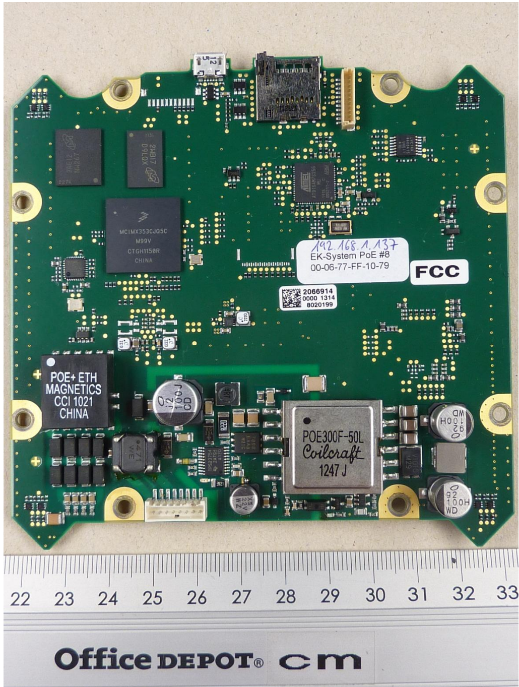
131991_e.JPG: RFU620-10501, EK-System PCB, top view
