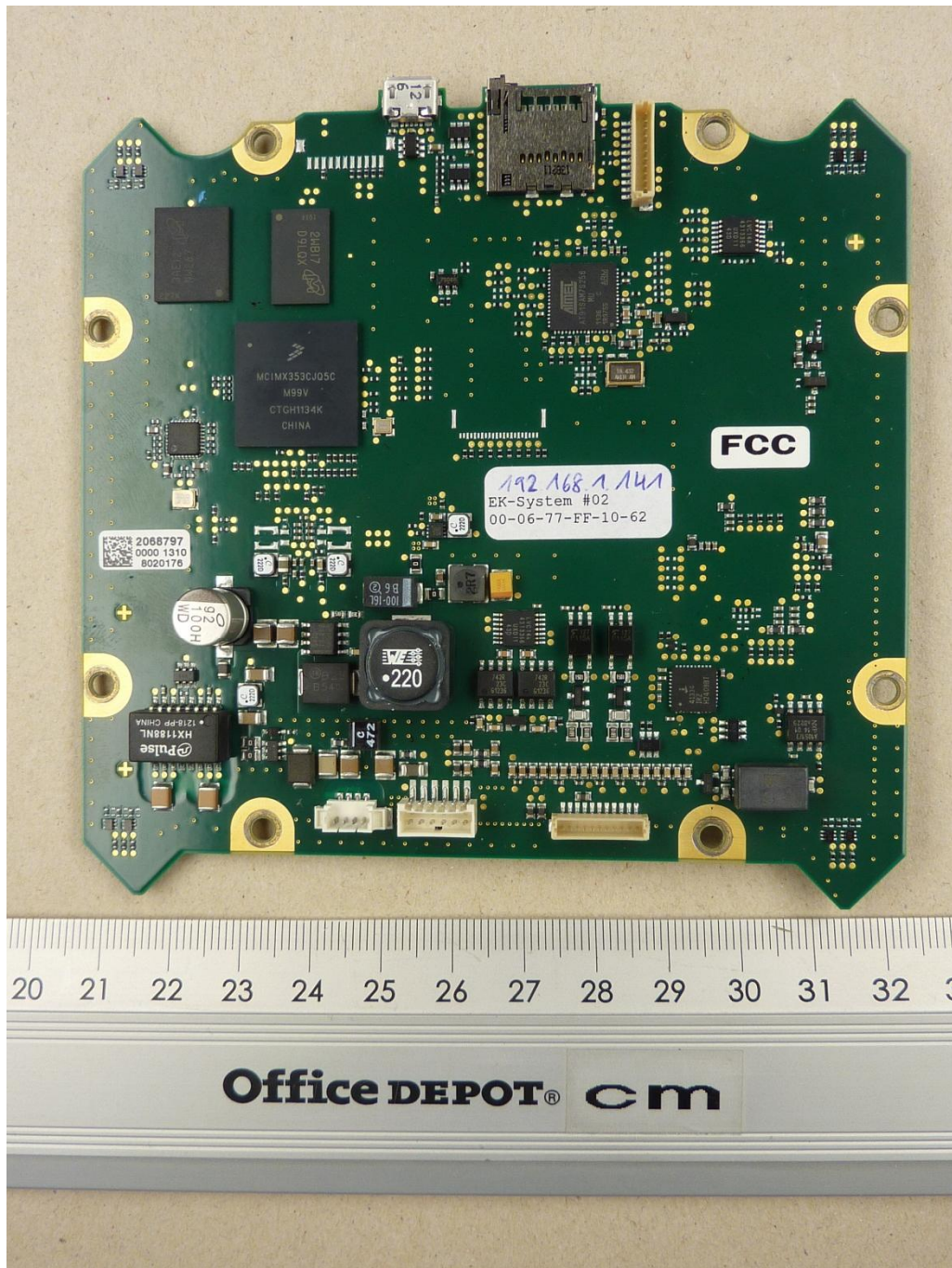
131992_g.JPG: RFU620-10101, EK-System PCB, top view
