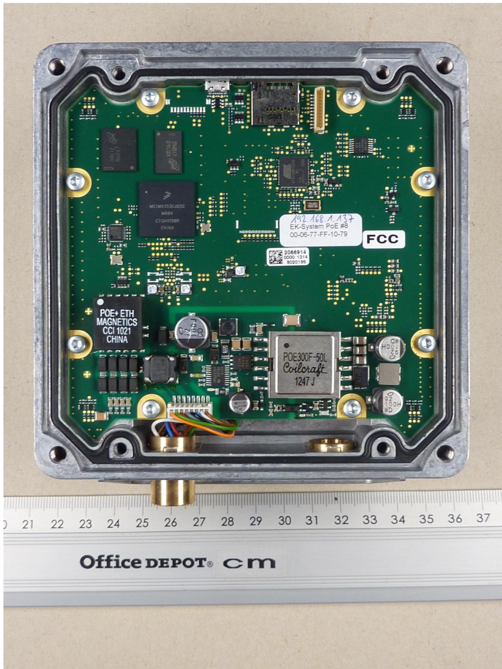
131991_c.JPG: RFU620-10501, internal view 1 (cover removed)
