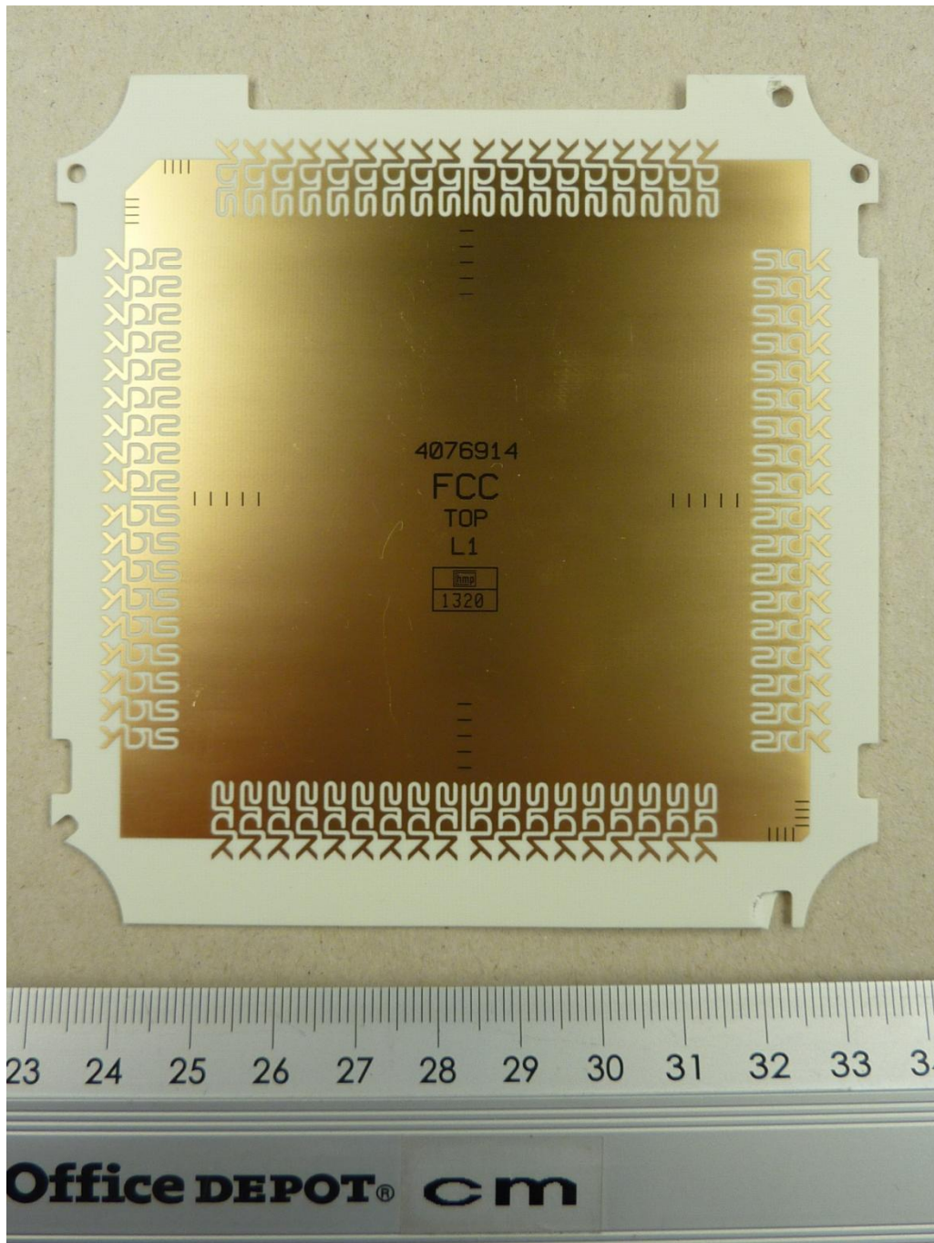
131992_j.JPG: RFU620-10101, LPL-Antenne PCB, top view
