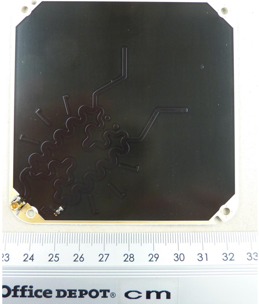
131992_e.JPG: RFU620-10101, EK-Koppler PCB, bottom view
