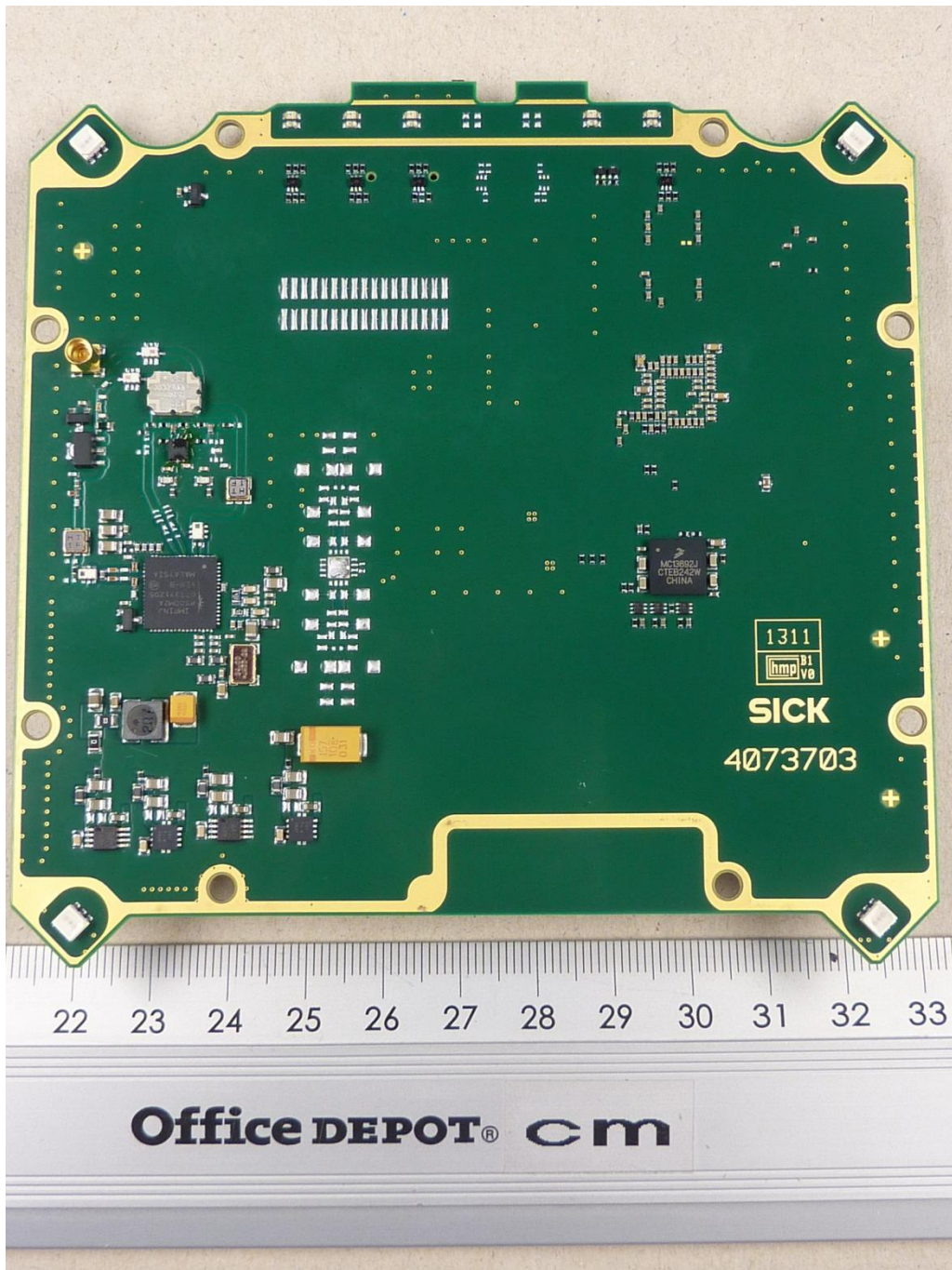
131991_f.JPG: RFU620-10501, EK-System PCB, bottom view
