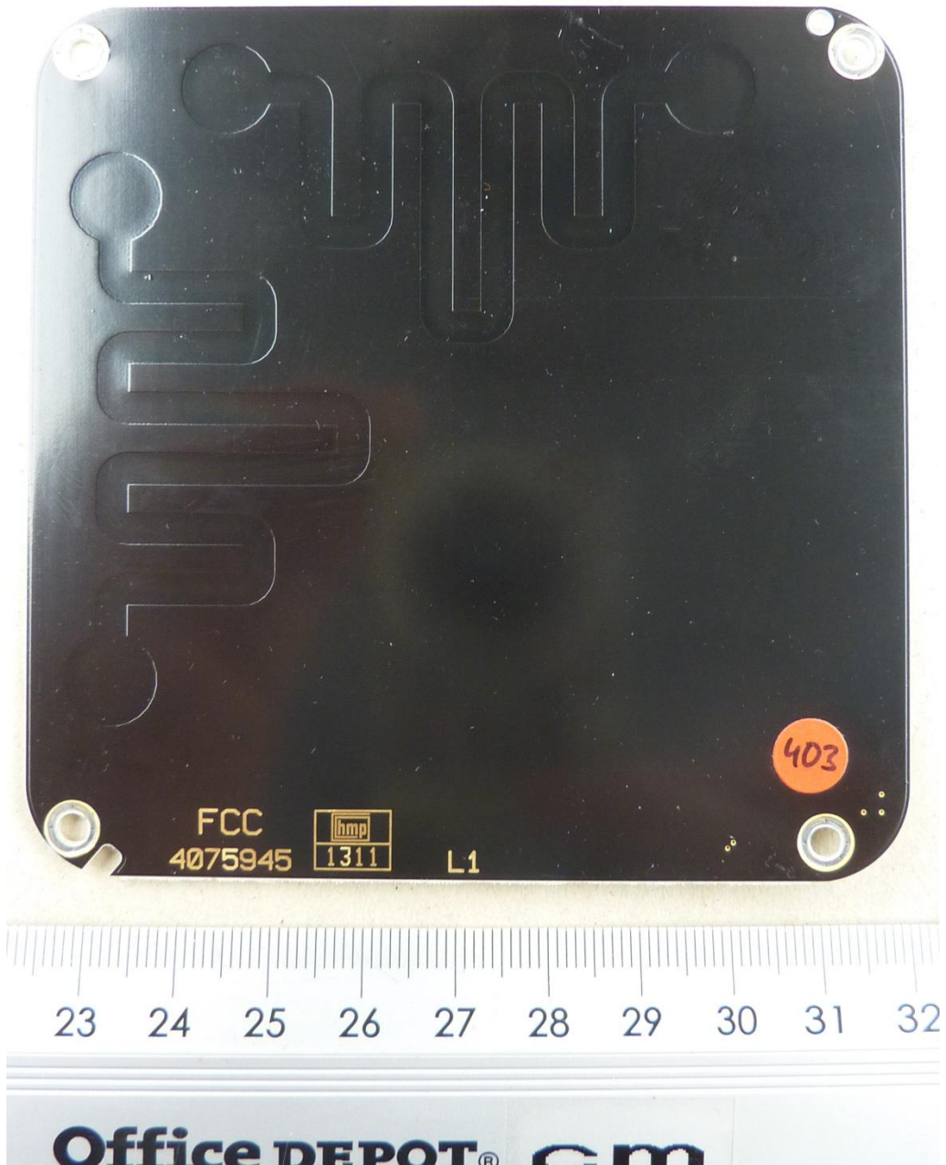
131992_m.JPG: RFU620-10101, EK-Koppler PCB, top view
