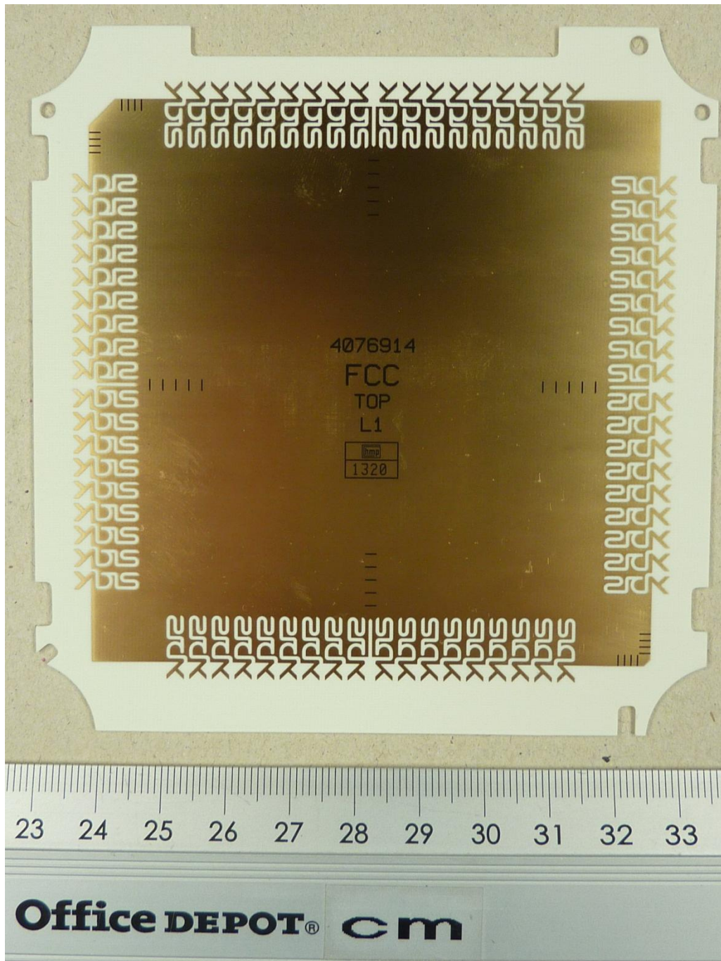
131991_g.JPG: RFU620-10501, LPL-Antenne PCB, top view
