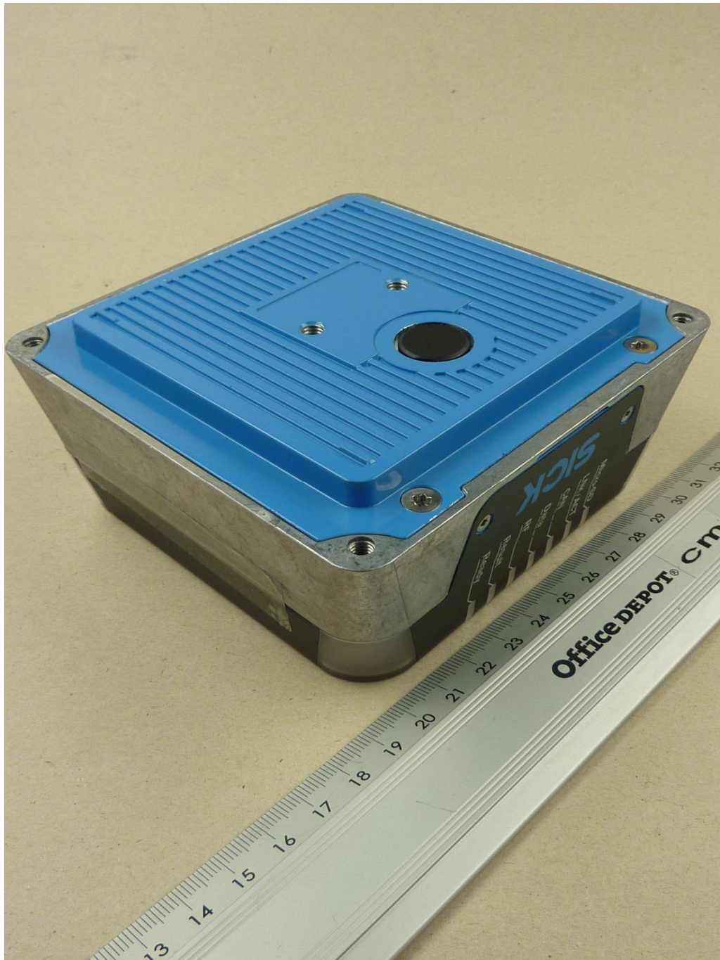
131991_b.JPG: RFU620-10501, 3-D.view 2
