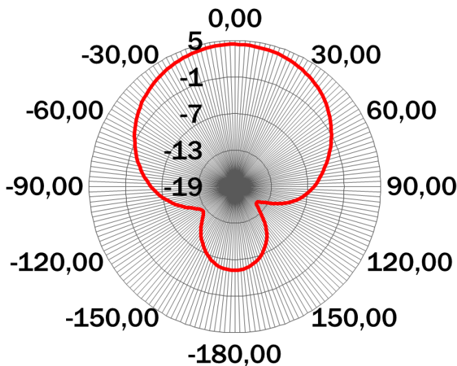
RADIATION PATTERN (915 MHz)
