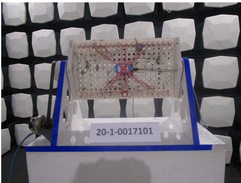
Photograph 4: EUT Test Setup in the fully anechoic chamber, close view
