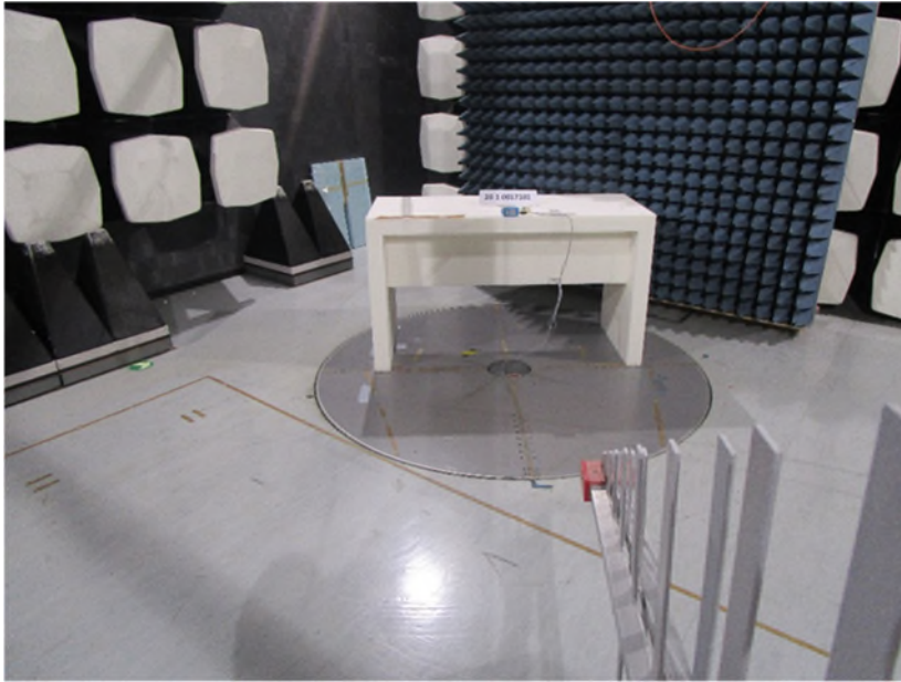
Photograph 1: EUT Test Setup in the anechoic chamber, overview
