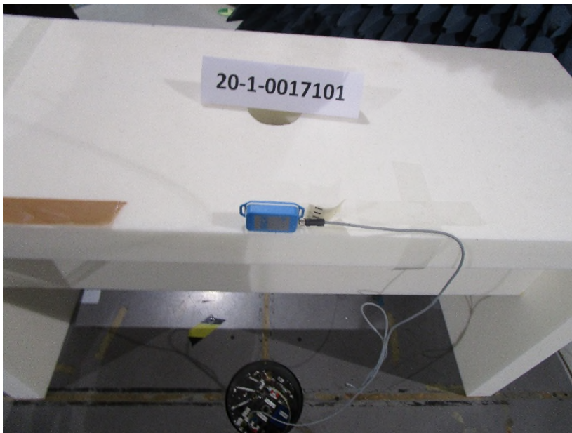
Photograph 2: EUT Test Setup in the anechoic chamber, close view
