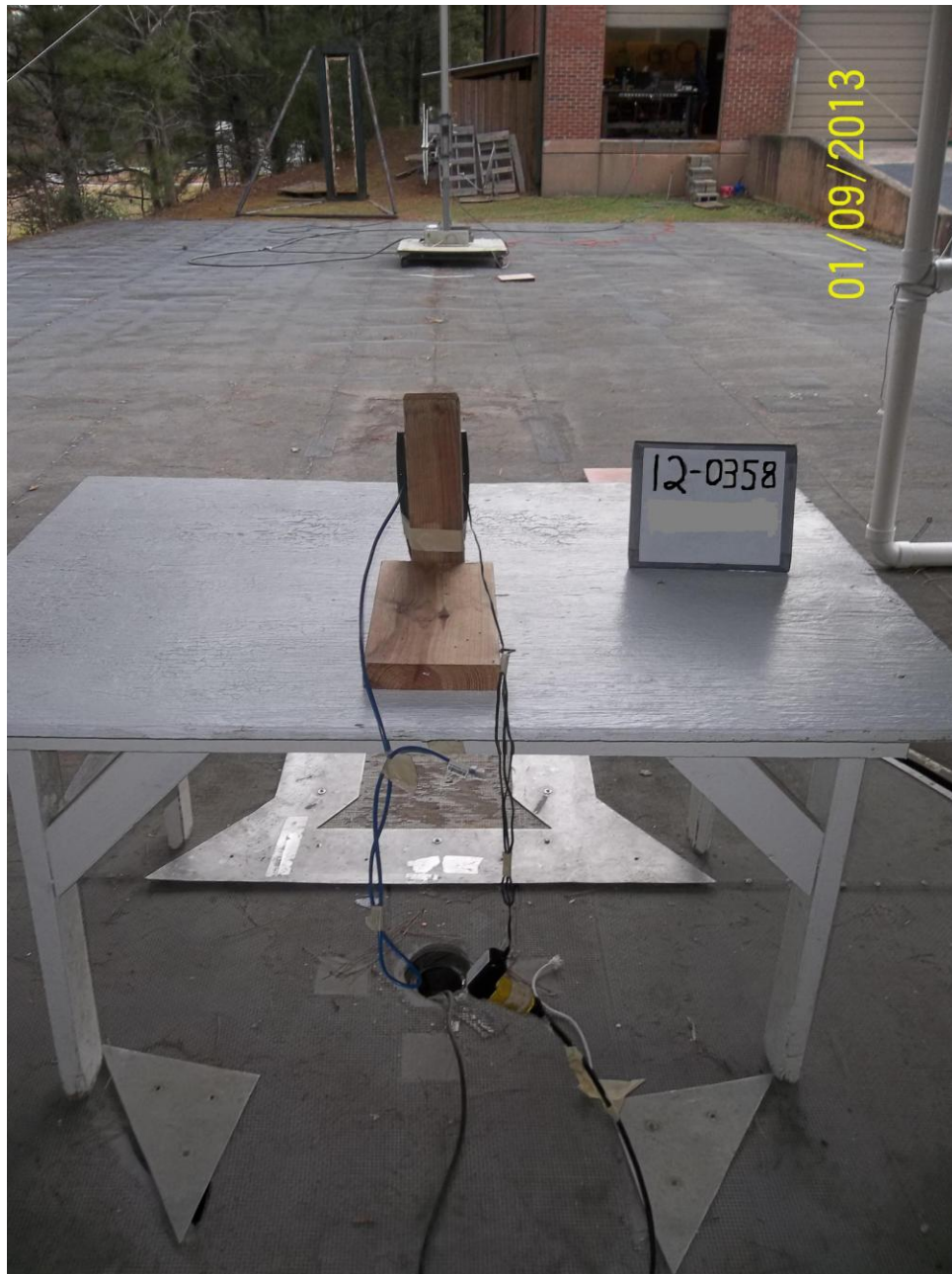
Figure 2- Test Setup Radiated Emissions Above 1 GHz
