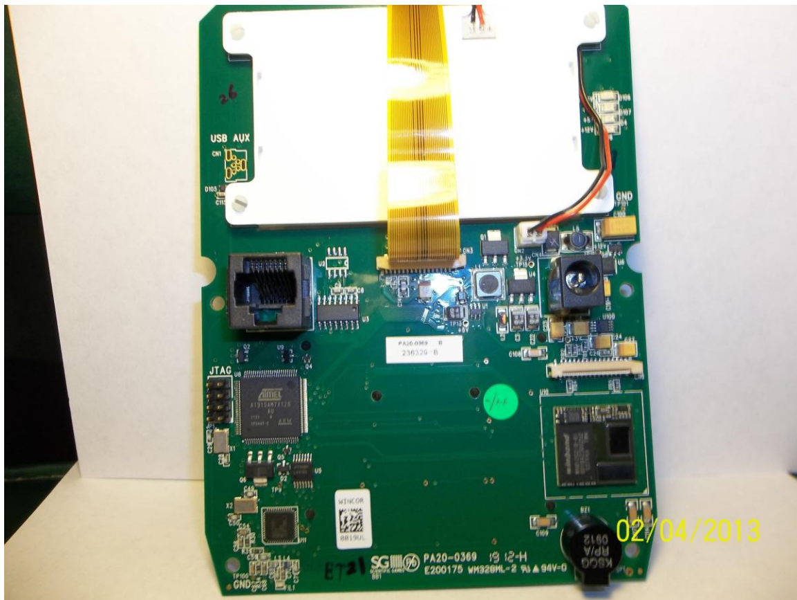
Figure 4- Back of PCB
