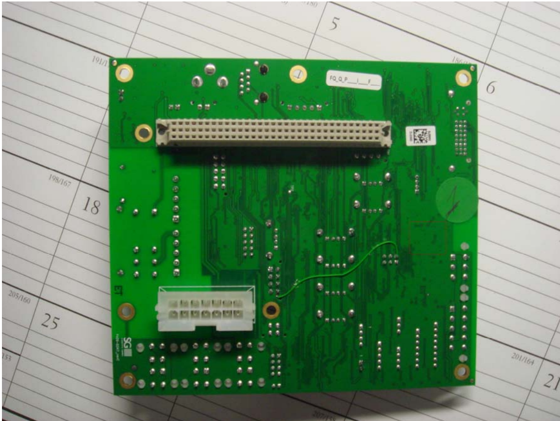
Photo 3 – PCB with Transmitter, Solder Side
