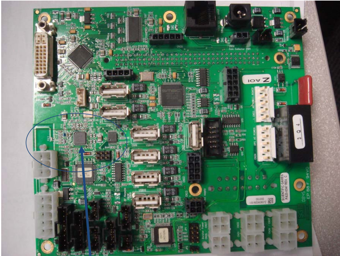
Photo 2 – PCB with Transmitter, Component Side
