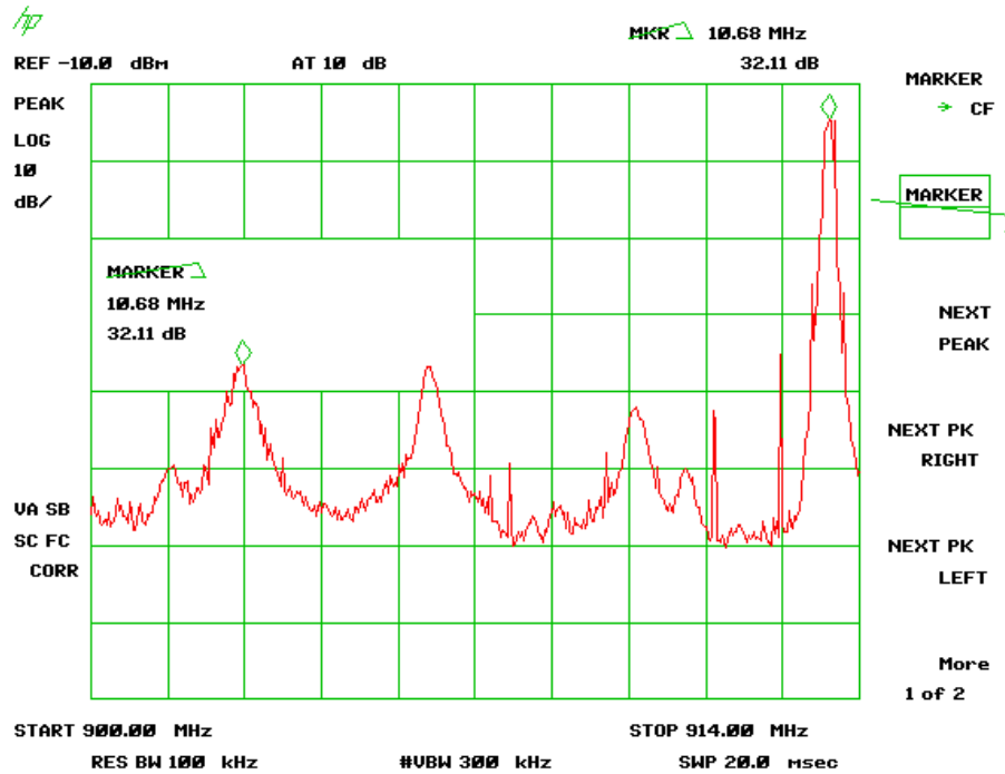
Figure 6 - Radiated Band Edge – Low Channel Delta – Peak
