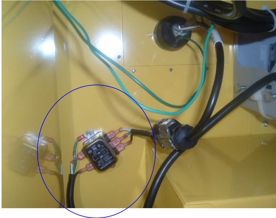
Figure 3 - Modification Photograph 2- EMI Line Filter Modification
