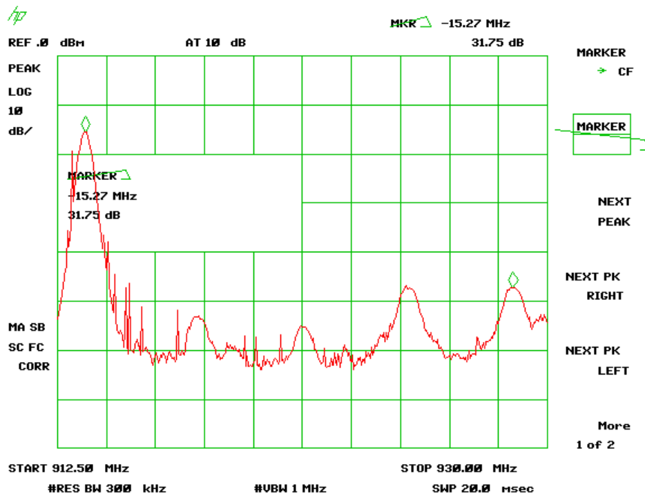
Figure 5 - Radiated Band Edge - High Channel Delta - Peak
