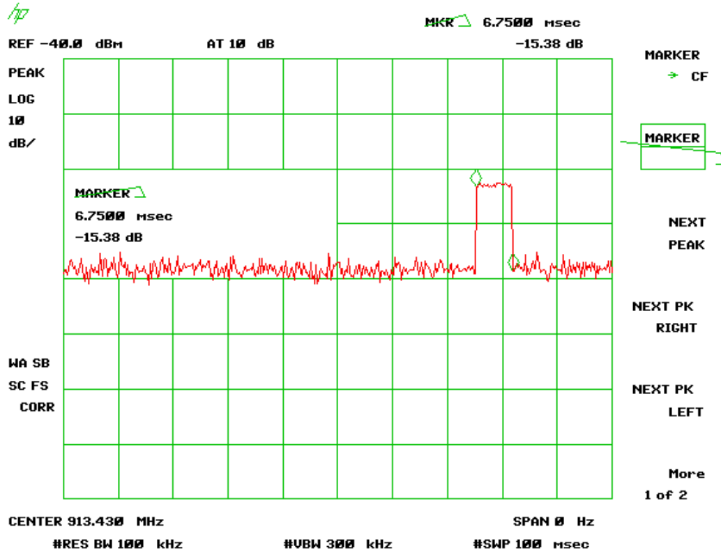
Figure 4 - Transmitter Pulse Width
