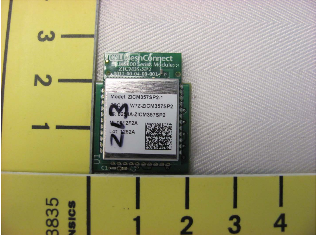
Illustration 2: Zigbee module
