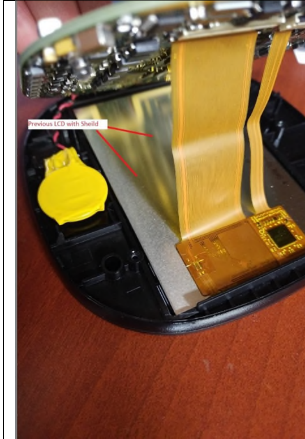
Figure 1 Previous Metal Shield around LCD
