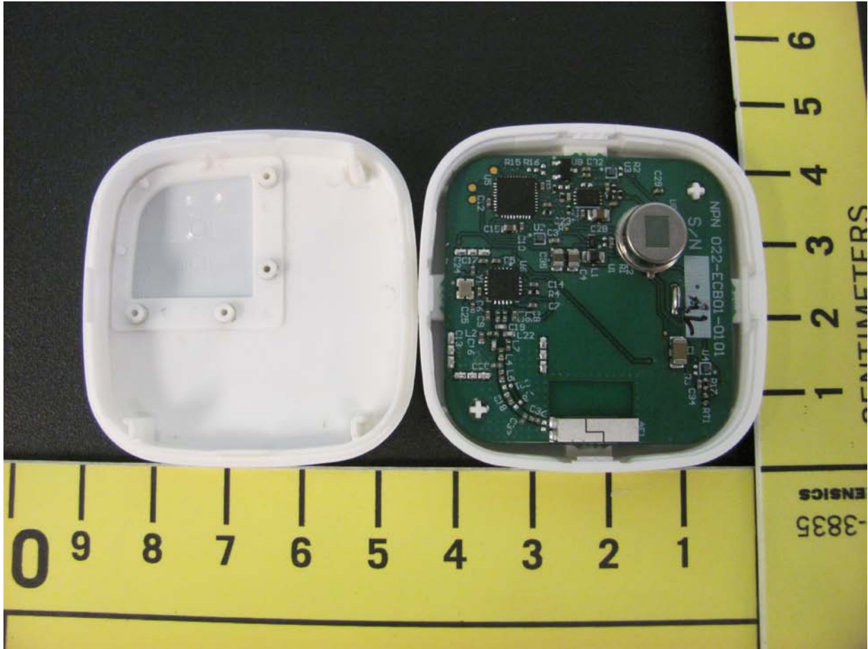
Illustration 1: EUT internal view – photo
