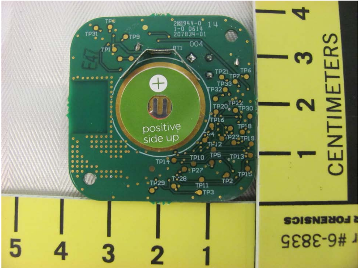
Illustration 3: EUT internal rear view – photo
