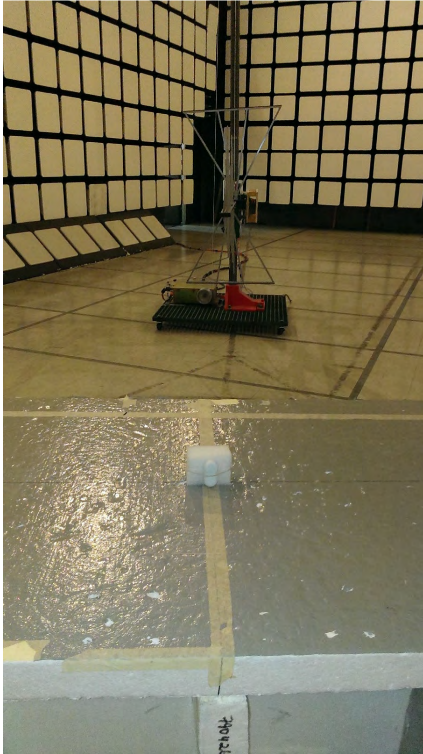
Radiated Emissions @ 3 m (30 – 1000 MHz)
