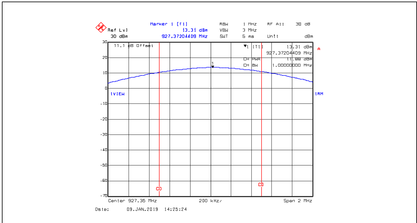
Plot 5.3.4.2. Maximum Conducted Output Power, FSK Modulation, Channel 49, 927.35 MHz
