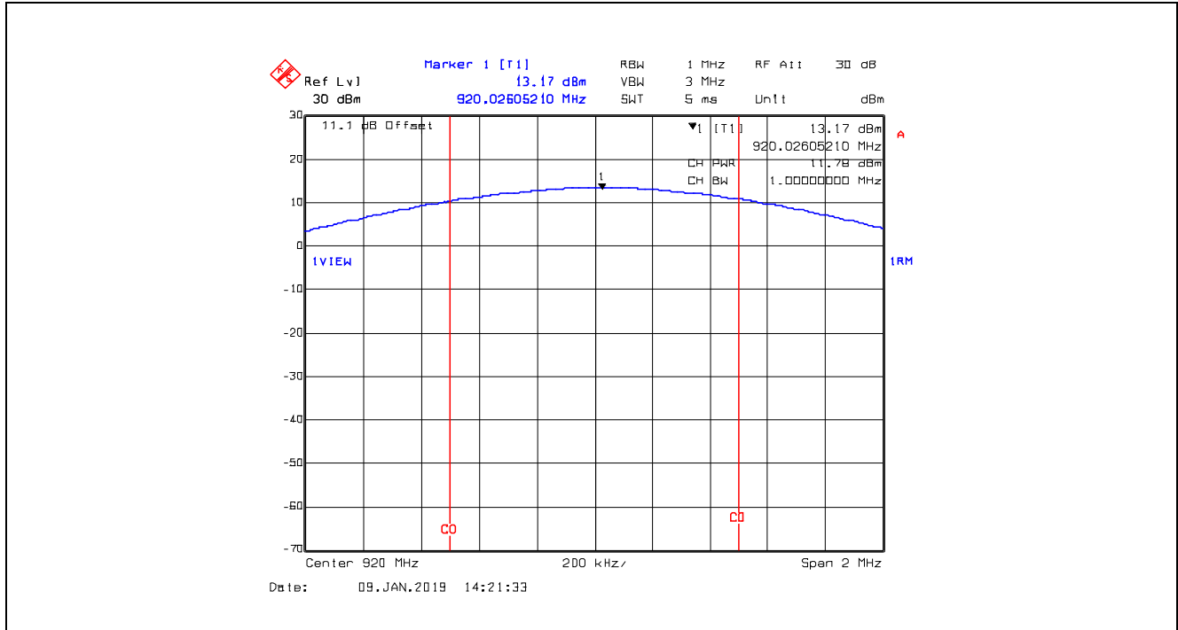
Plot 5.3.4.1. Maximum Conducted Output Power, FSK Modulation, Channel 0, 920.00 MHz
