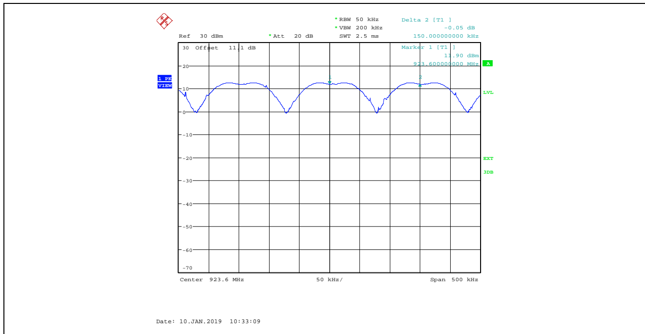
Plot 5.2.4.3. Carrier Frequency Separation
