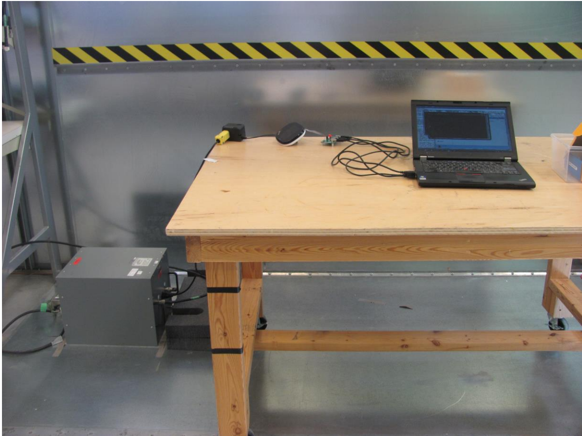
Figure 6 – Power Line Conducted Emissions Setup – Photo 1
