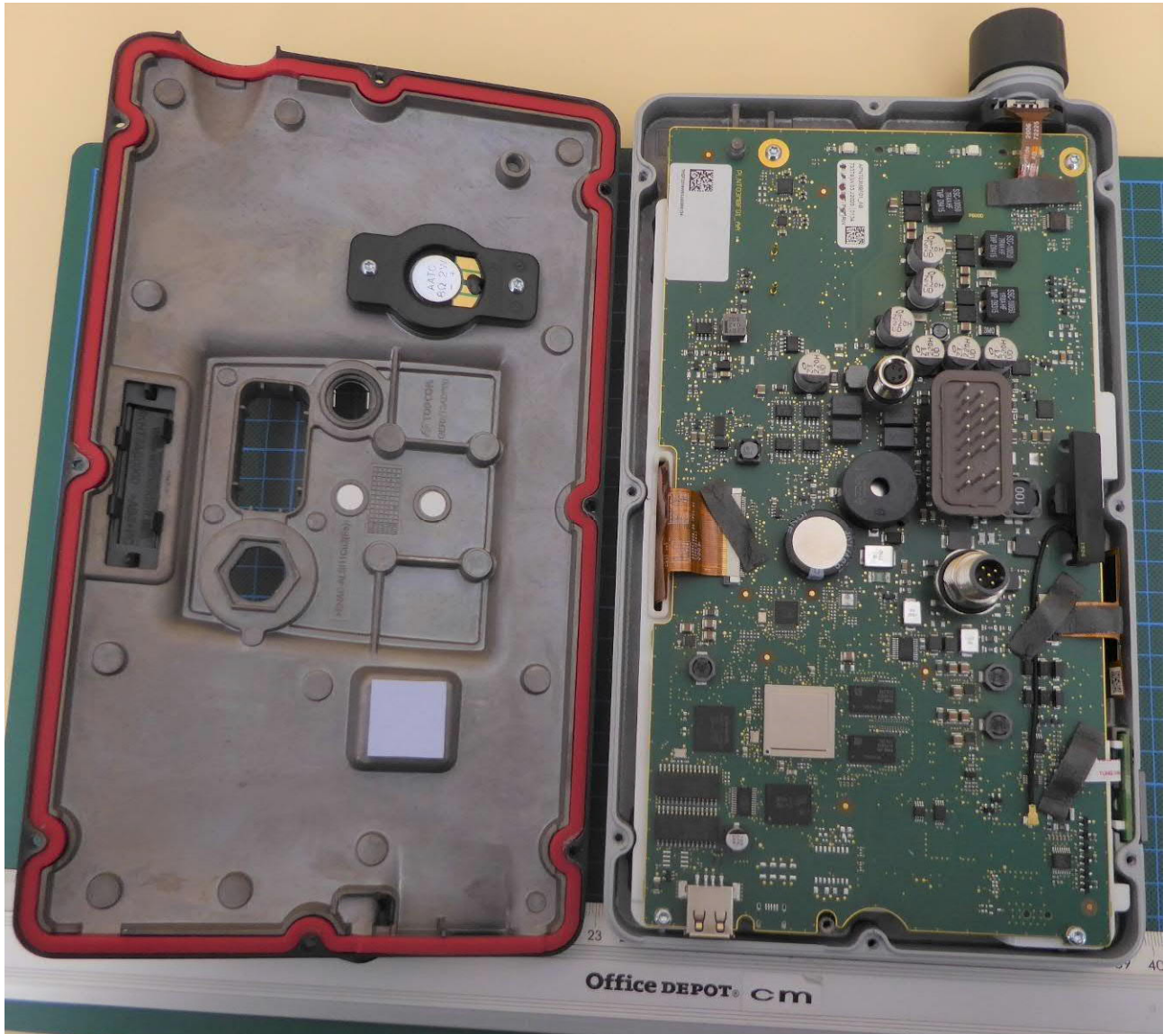
EUT – internal view 1
