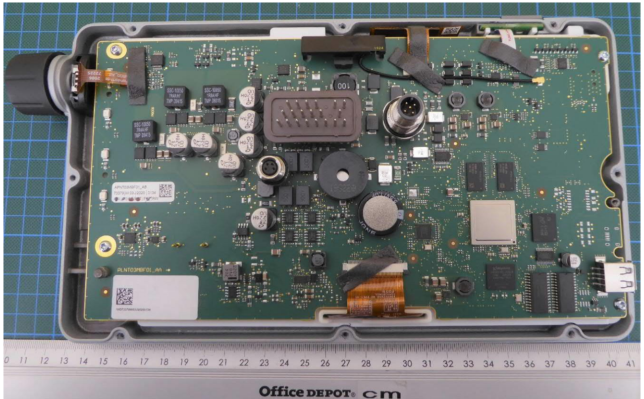
EUT – internal view 2
