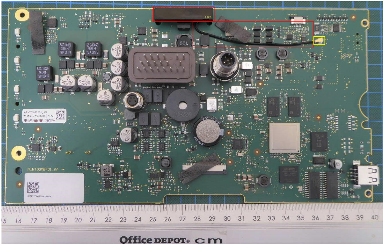
Main PCB – top view
