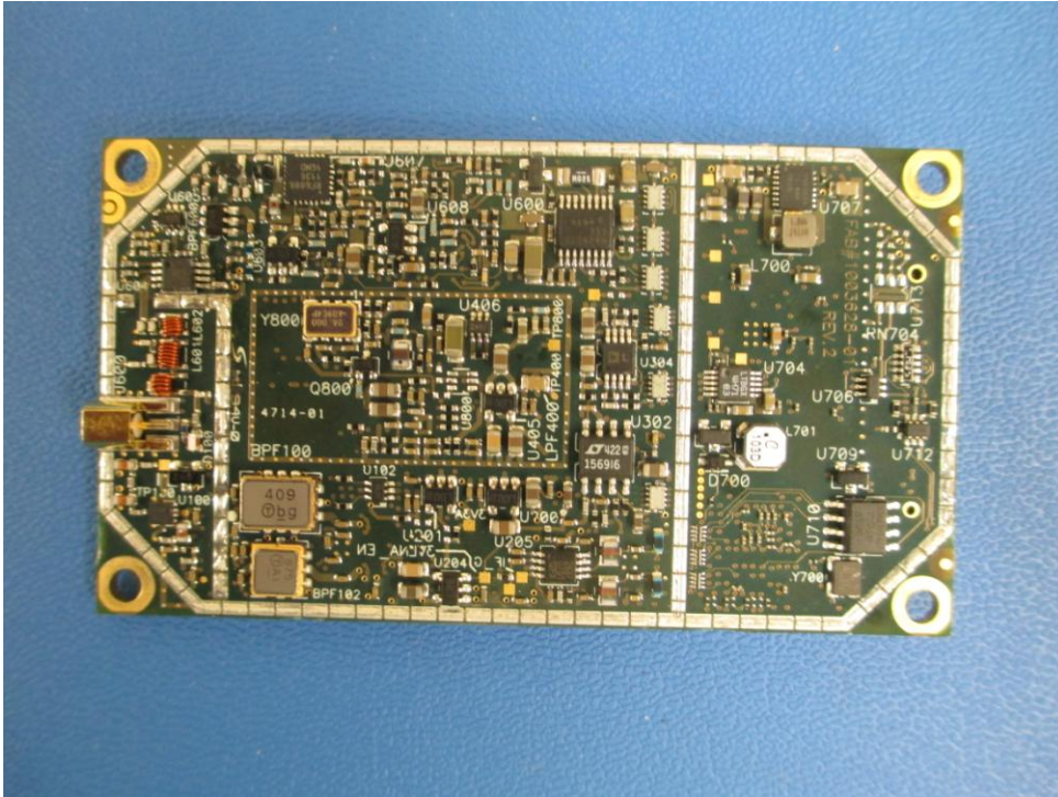
R2Lite UHF MODULE without SHIELD (TOP)
