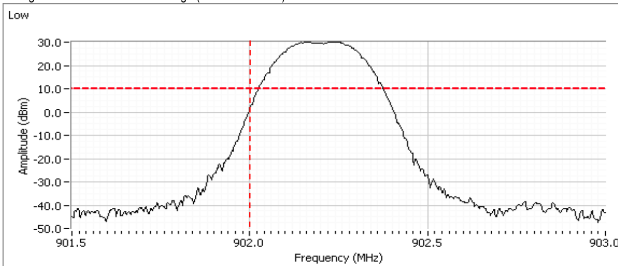
Plot showing -20 dBc at the lower band edge (Tx at 902.2 MHz)
