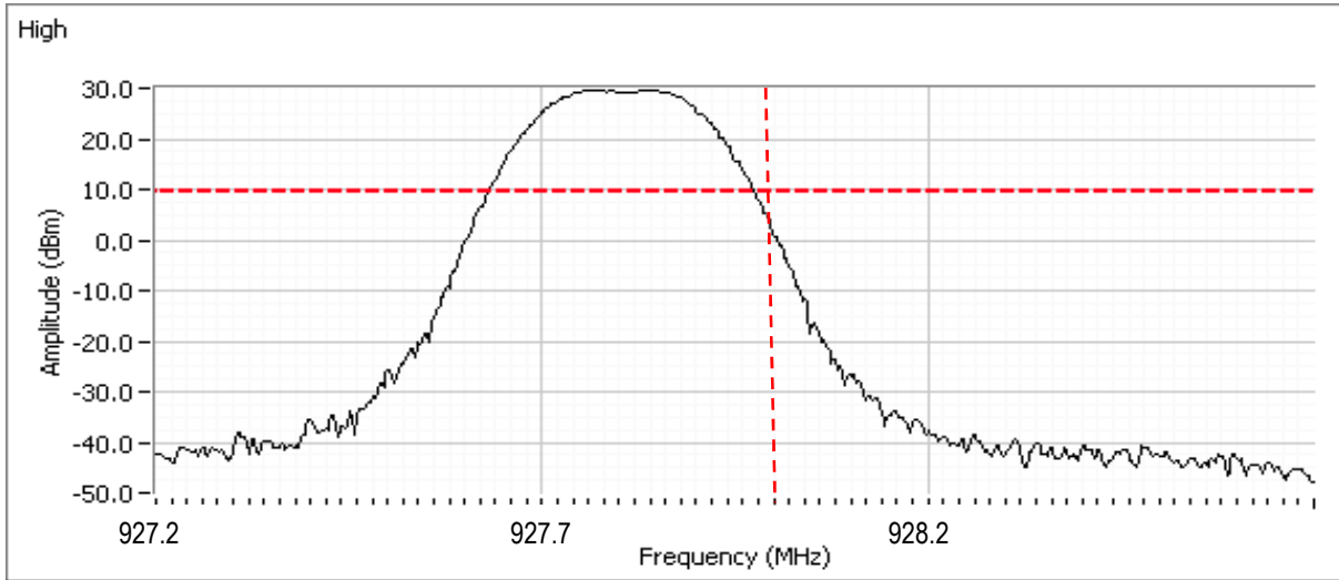
Plot showing -20 dBc at the upper band edge (Tx at 927.8 MHz)
