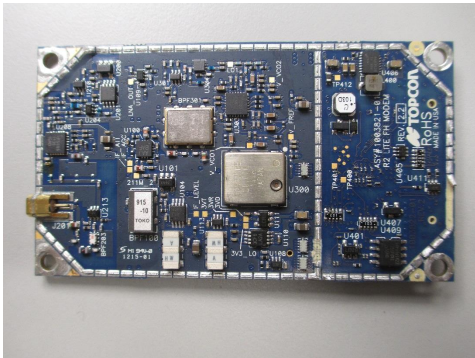
R2Lite FH915 MODULE without SHIELD (TOP)
