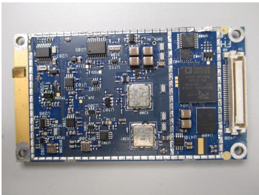
R2Lite FH915 MODULE without SHIELD (BOTTOM)
